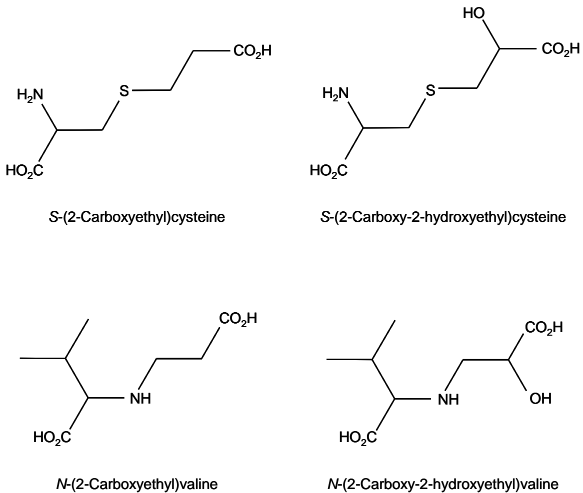
FIGURE 4 Cysteine and Valine Adducts of Acrylamide and Glycidamide
