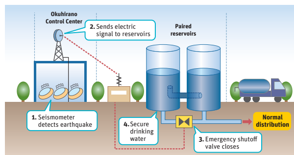
Figure 2. Okuhirano Control Center's Emergency Water Storage System, Kobe City
