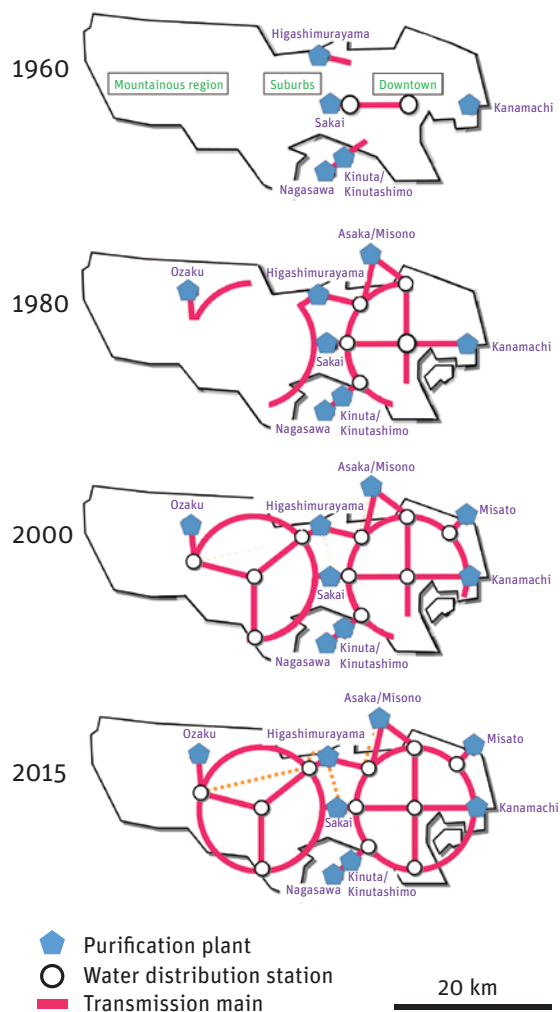
Figure 4. Interconnections of Water Treatment Plants with Pipelines, Tokyo, 1960–2015
