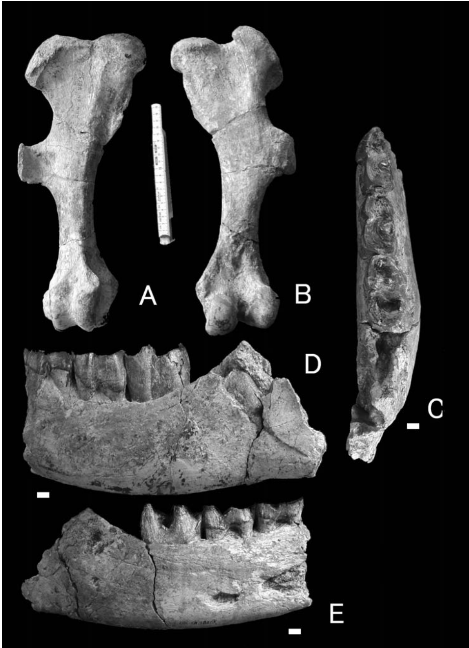
Fig. 6. A-B: cf. Paradiceros mukirii . A) dorsal and B) plantar views of the right femur (KNM-SH 40136). C-E: Chilotheridium pattersoni . C) occlusal, D) buccal and E) lingual views of the left mandible with P_4 - M_2 (KNM-SH 38405). Scales in cm (C-E).
