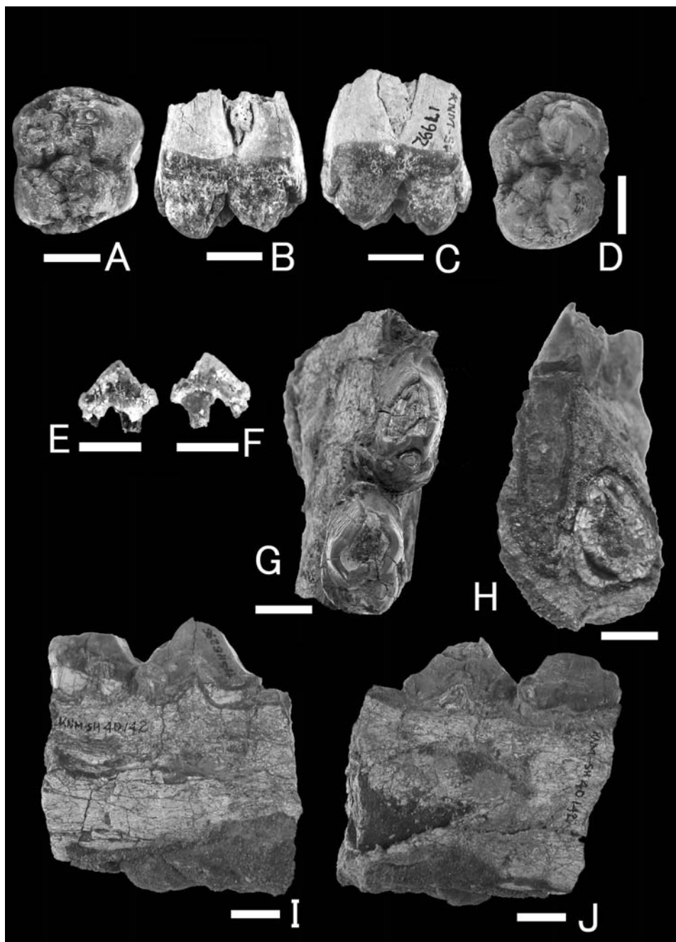
Fig. 8. A-D: Nyanzachoerus sp. A) occlusal, B) buccal and C) lingual views of the left M 2 (KNM-SH 17992); D) occlusal view of the left dP 47 (KNM-SH 18003). E-F: ? Nyanzachoerus devauxi . E) buccal and F) lingual views of the left lower premolar (KNM-SH 18010). G-J: Kenyapotamus coryndoni . G) occlusal, H) anterior, I) buccal and J) lingual views of the right mandible with P 3.4 (KNM-SH 40142). Scales in cm.
