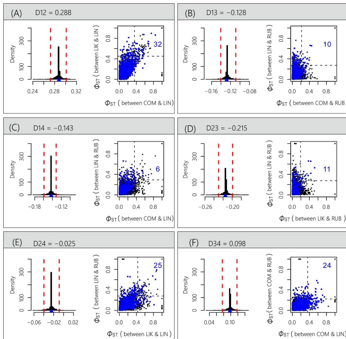
Figure 4. Tests of gene flow among each pair of taxa and population differentiation at putatively introgressed loci. Abbreviations for the four taxa: 1 = var. complanata , 2 = var. likiangensis , 3 = var. linzhiensis , 4 = var. rubescens . Positive DIJ represents gene flow between a pair of taxa I and J (I = 1, 2, 3; J = 2, 3, 4). For each pair of taxa, 1000 jackknife replicates were used to generate each density distribution, where the broken lines indicate the 95% confidence intervals and solid triangles denote observed value for each pair (shown on left side of each panel, A-F). For each pair of taxa, we also computed the \Phi_{ST} per locus and then plotted values for a particular taxon pair against another pair where one taxon was common to both pairs while the other two taxa involved were different (shown on right side of each panel, A-F). This was done for both putative introgressed loci (blue squares) and non-introgressed loci (black crosses). Thus, in panel A the plot is shown of values of \Phi_{ST} per locus for var. likiangensis versus var. linzhiensis against \Phi_{ST} values for var. complanata versus var. linzhiensis . Broken lines within each plot represent the 95% \Phi_{ST} -quantiles for all loci. Blue integers represent the number of putative introgressed loci for which \Phi_{ST} is higher than 95% \Phi_{ST} -quantiles in two dimensions.
