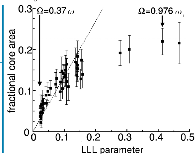
► Fig. 5: Fractional core area as a function of the LLL parameter. The fractional core area is the ratio of the square of the core size (measured using a Gaussian fit of the density dip at the vortex locations) and the area of the unit cell of the vortex lattice. The LLL parameter is the ratio of the energy splitting between two Landau levels ( 2\hbar\omega_{\perp} ) and the interaction energy characterized by the chemical potential \mu . The entrance in the LLL occurs for an LLL parameter of order unity. The broken line is the prediction obtained assuming that the vortex core is proportional to the healing length \xi . The dotted line corresponds to the expected limit for the LLL (figure obtained by the group of E. Cornell at Boulder [14]).
