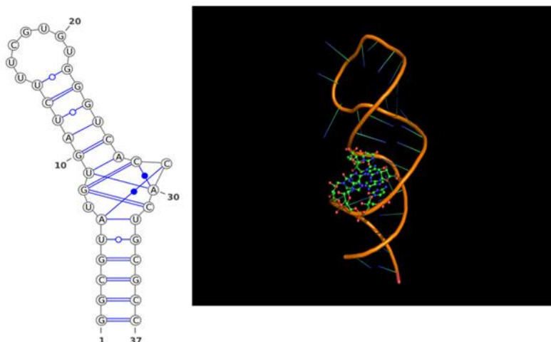
Figure 9 | An example of higher order structure (C-loop) in RNA by formation of base triples using non-canonical base pair from PDB: 1KOG (a) by schematic representation and (b) by molecular visualizer
