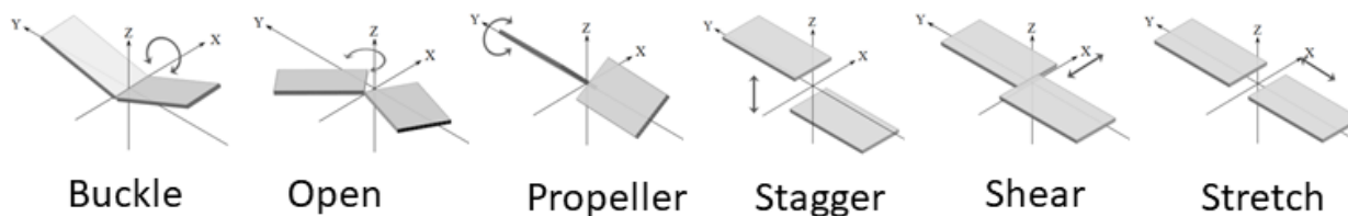
Figure 8 | IUPAC recommended Intra Base Pair parameters used to describe geometry of Watson-Crick or Non-Canonical base pair
