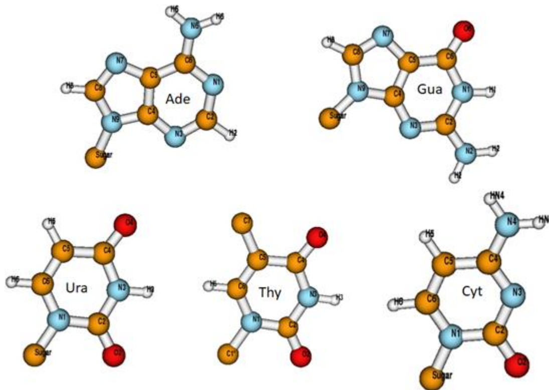
Figure 2 | IUPAC-IUB recommended nomenclature of nucleotide base atoms of Adenine, Guanine, Uracil and Cytosine bases (created in MOLDEDN).
