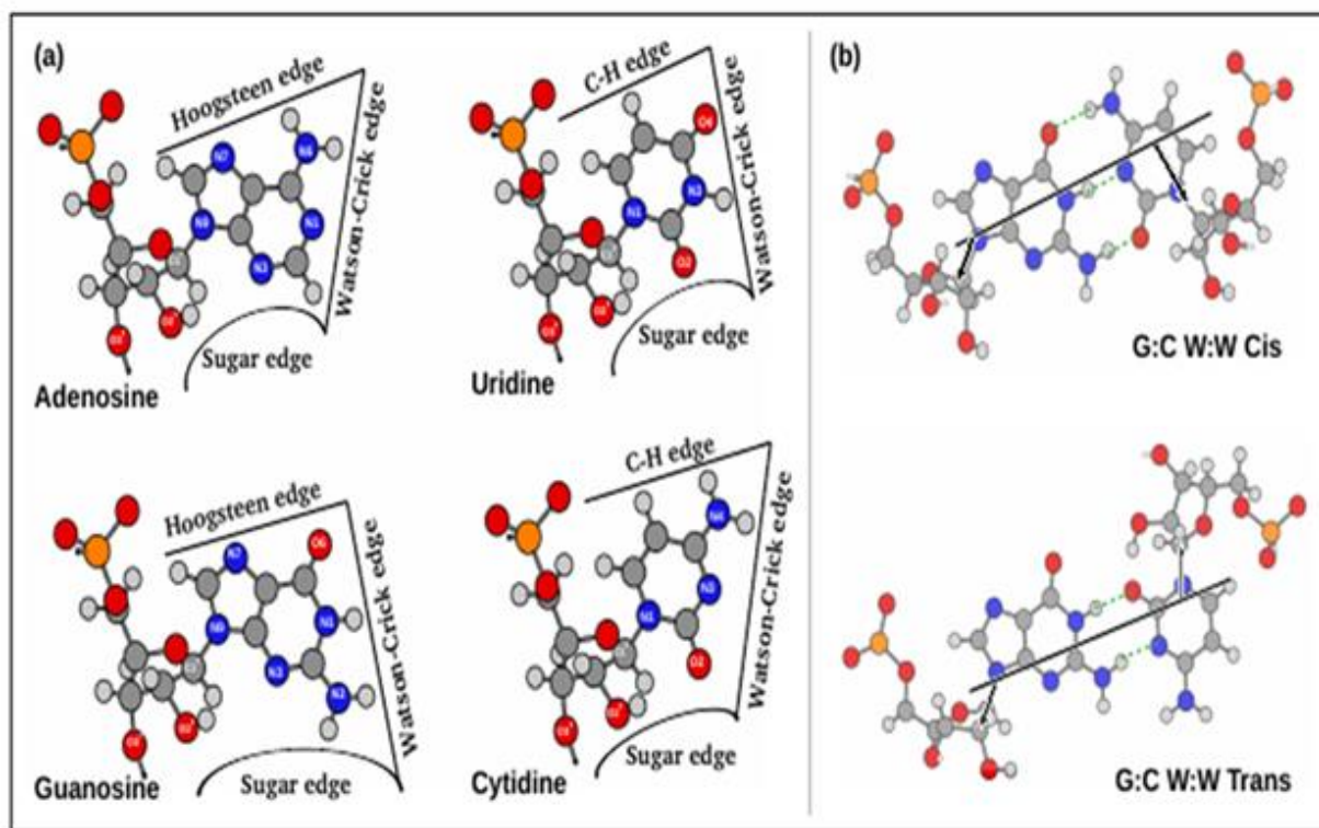
Figure 5 | (a) Three hydrogen bonding edges of the four nucleotides (Guanine), showing nomenclature of each edge and (b) Cis and Trans orientations of the sugar moieties of the two nucleotide residues glycosidic bonds of a base pair with respect to hydrogen bonding direction. The arrows in (b) indicate glycosidic bonds as vectors.
