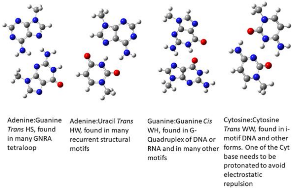
Figure 1 | Examples of few frequently observed non-canonical base pairs, (a) Adenine: Guanine trans Hoogsteen/Sugar-edge, (b) Adenine: Uracil trans Hoogsteen/Watson-Crick, (c) Guanine: Guanine cis Watson-Crick/Hoogsteen; (d) Protonated Cytosine (+): Cytosine trans Watson-Crick/Watson-Crick
