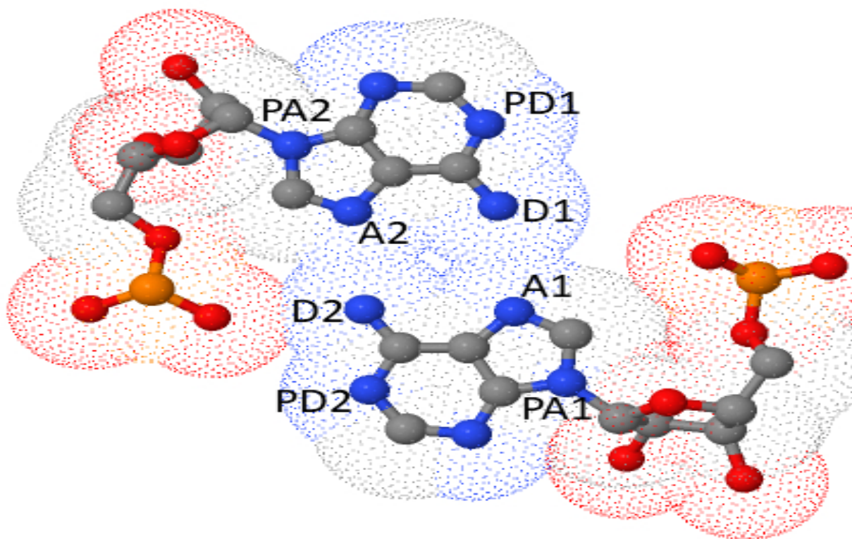
Figure 7 | Descriptions of the hydrogen bonding atoms, along with their precursors, for a typical non-canonical base pair (as used by BPFIND)
