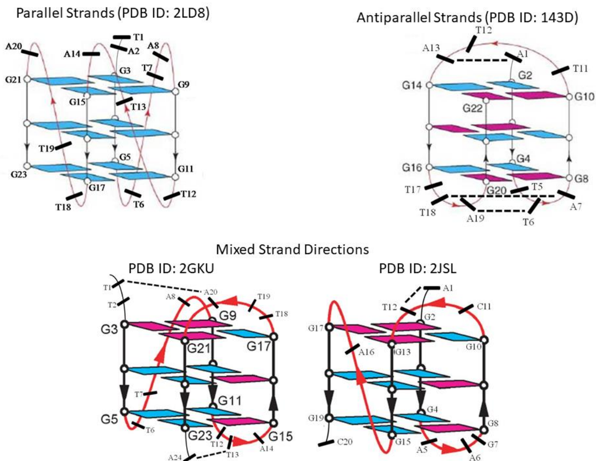
Figure 4 | Three G-quadruplexes stack to form four stranded telomere with different topologies for d(GGATTGGGATTGGGATTGGG) sequence
