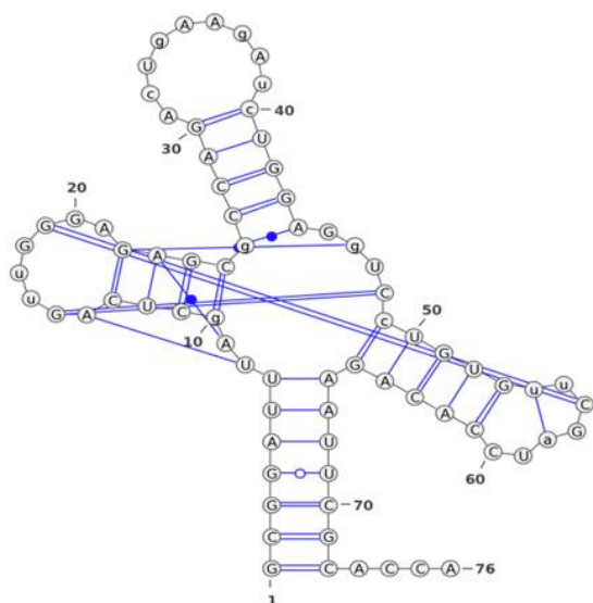
Figure 6 | (a) Cloverleaf model of tRNAPhe (picture created by VARNA [35] for PDB: 1EHZ) and (b) A typical base triplet involving residues 9, 12 and 23 of the same tRNA
