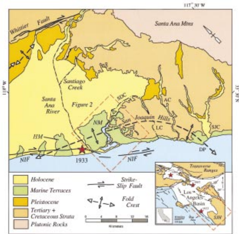
Figure 1. Regional map of San Joaquin Hills (SJH) showing approximate location of fold crest of San Joaquin Hills anticline. Other features: AC—Aliso Canyon, DP—Dana Point, HM—Huntington Mesa, LC—Laguna Canyon, NIF—Newport-Inglewood fault, NM—Newport Mesa, SDC—San Diego Creek, and SJC—San Juan Capistrano. Epicenters of 1933, 1987, and 1994 earthquakes are marked by stars. Modified from Vedder et al. (1957). Inset map shows greater Los Angeles region.
