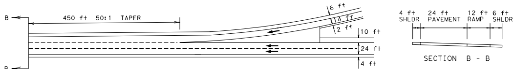
DETAIL OF ENTRANCE RAMP GORE
