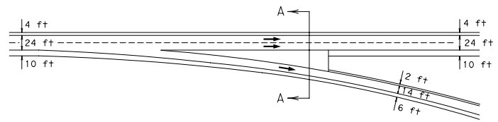
DETAIL OF EXIT RAMP GORE
