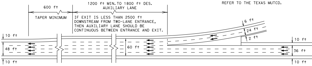
MULTILANE MERGE
