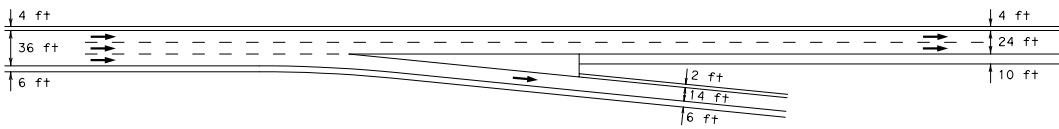
AUXILIARY LANE TERMINATION
