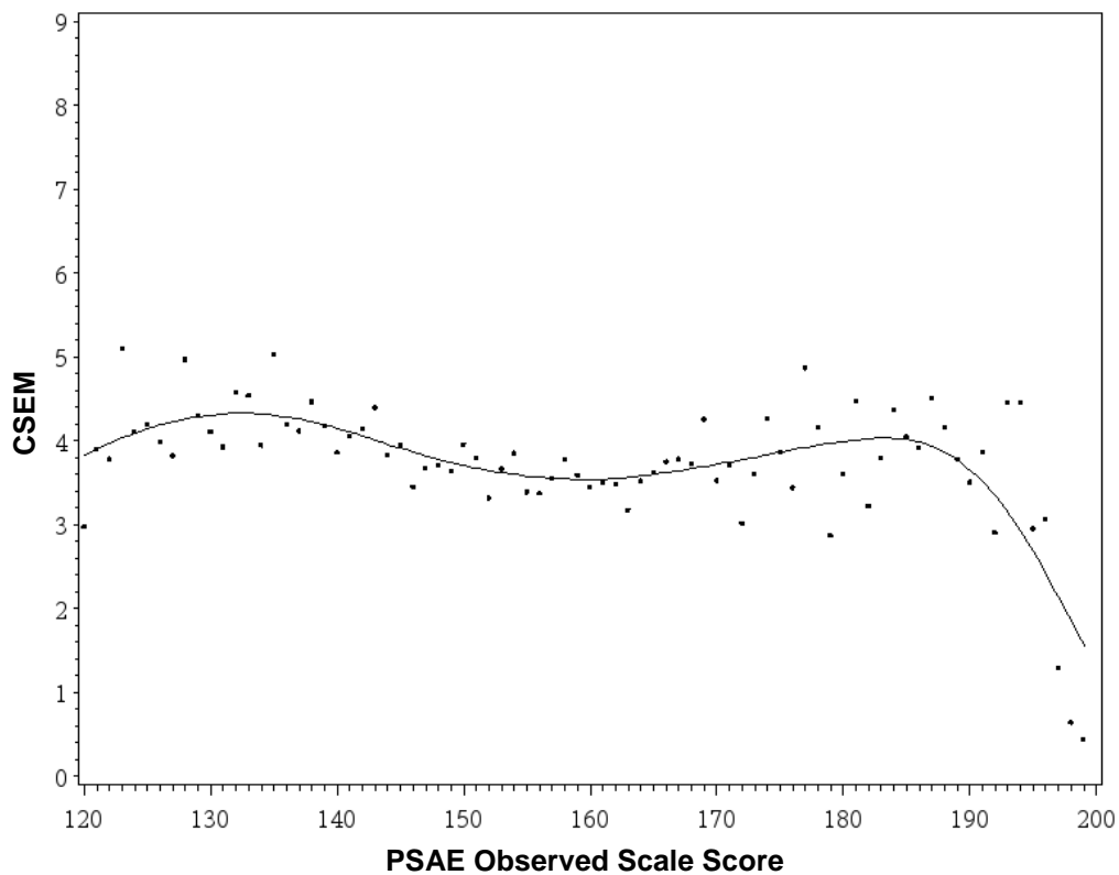
Figure 4.9: PSAE Writing – Conditional Standard Errors of Measurement (CSEM) by Observed Scale Score for the PSAE Spring 2010 Administration
