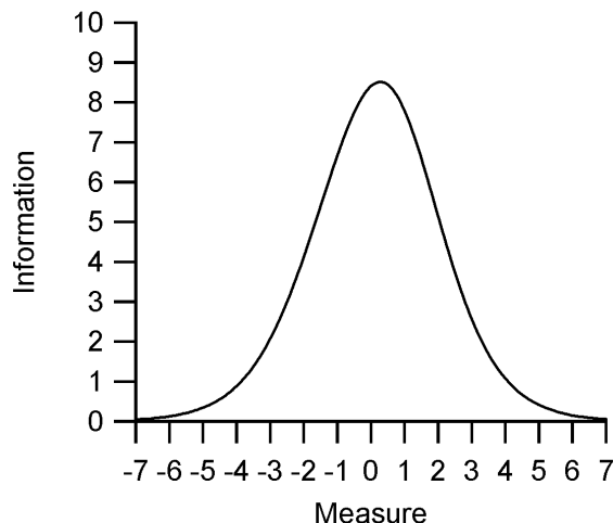
Figure 2.1: 2010 ISBE-Developed Science Test Information Function
