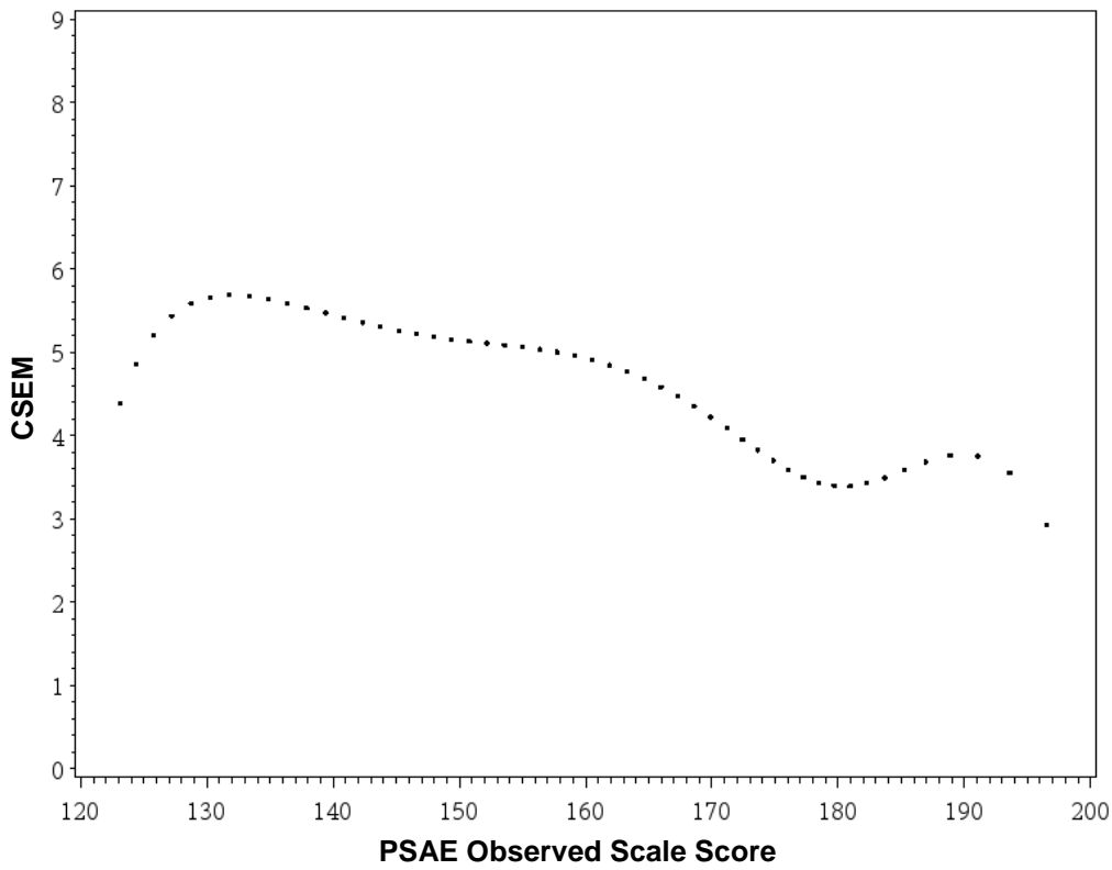
Figure 4.7: PSAE Mathematics – Conditional Standard Errors of Measurement (CSEM) by Observed Scale Score for the PSAE Spring 2010 Administration
