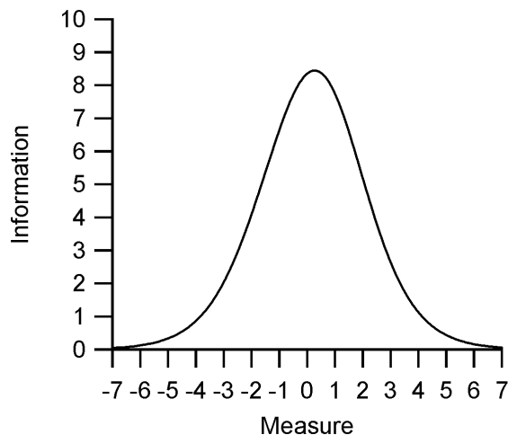
Figure 2.1: 2011 ISBE-Developed Science Test Information Function
