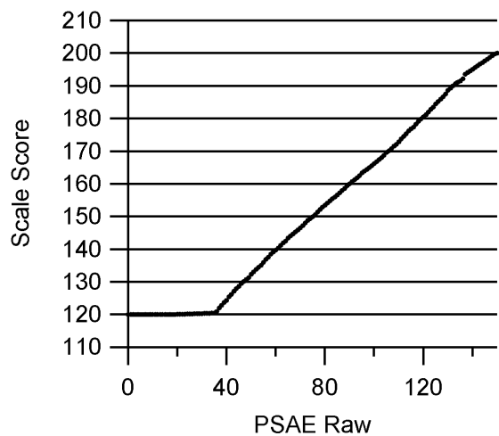
Figure 4.4: Raw-to-Scale-Score Transformation for PSAE Writing
