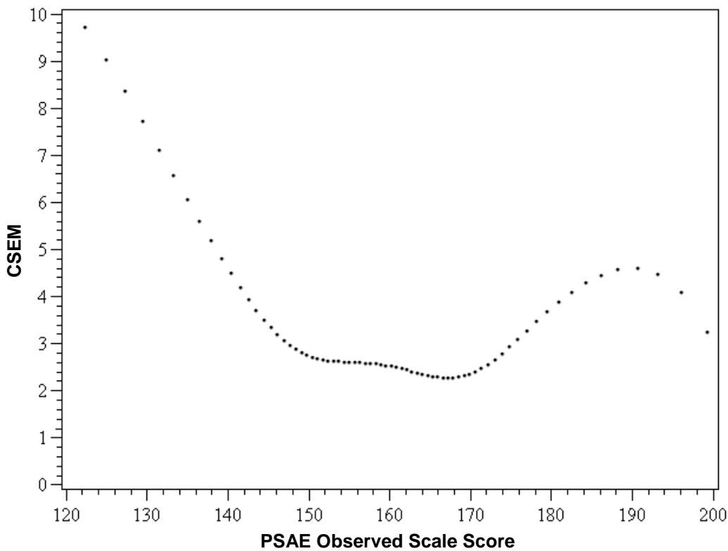
Figure 4.7: PSAE Mathematics – Conditional Standard Errors of Measurement (CSEM) by Observed Scale Score for the PSAE Spring 2011 Administration
