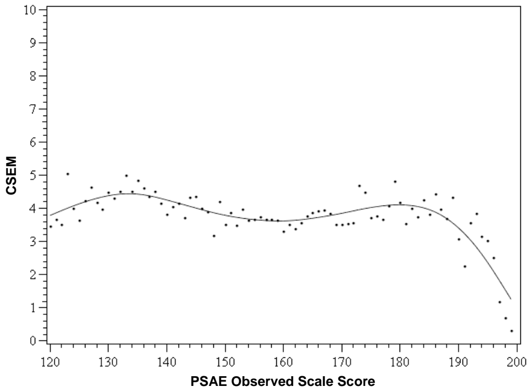
Figure 4.9: PSAE Writing – Conditional Standard Errors of Measurement (CSEM) by Observed Scale Score for the PSAE Spring 2011 Administration
