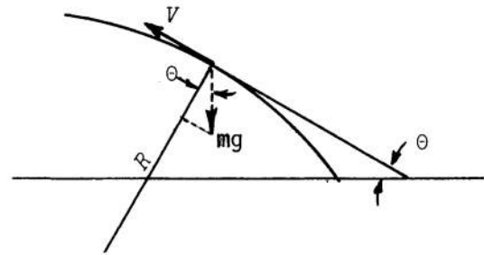
Figure 4-7. Diagram of Gravity Force on Projectile
