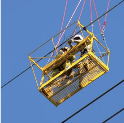
Insulator Cleaning System (by SIMPLEX)
