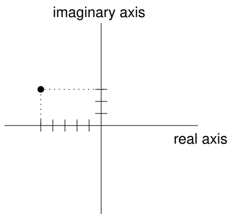
Cartesian coordinates
