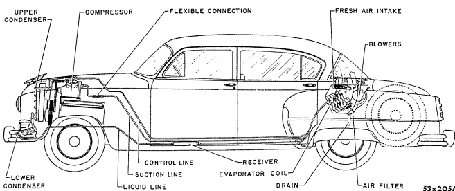
Figure 7: The automotive air-conditioning system developed by Airtemp Division of Chrysler Corporation in 1953 featuring a dual-condenser arrangement and R-22 refrigerant. 9
