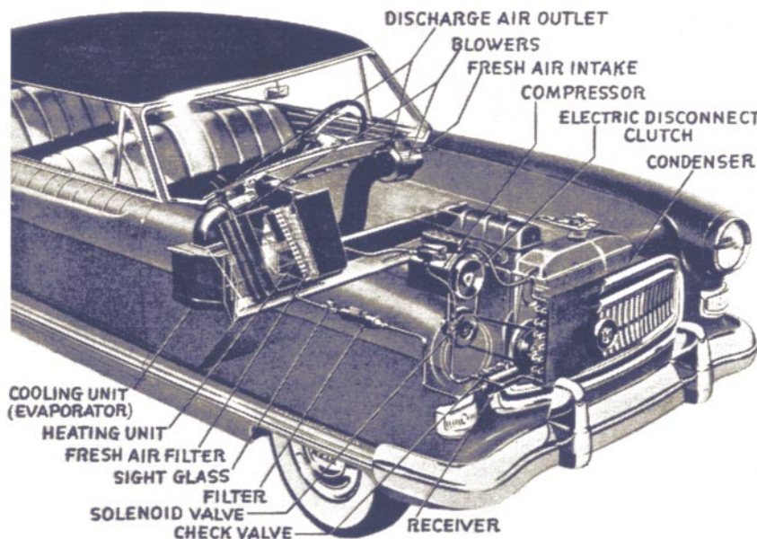
Figure 9: The 1954 Nash All-Weather Eye automotive air-conditioning system with a single knob control that pioneered the automatic four-season controls. 11
