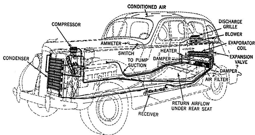
Figure 3: The first practical automotive air-conditioning system developed by Packard in 1939. 3
