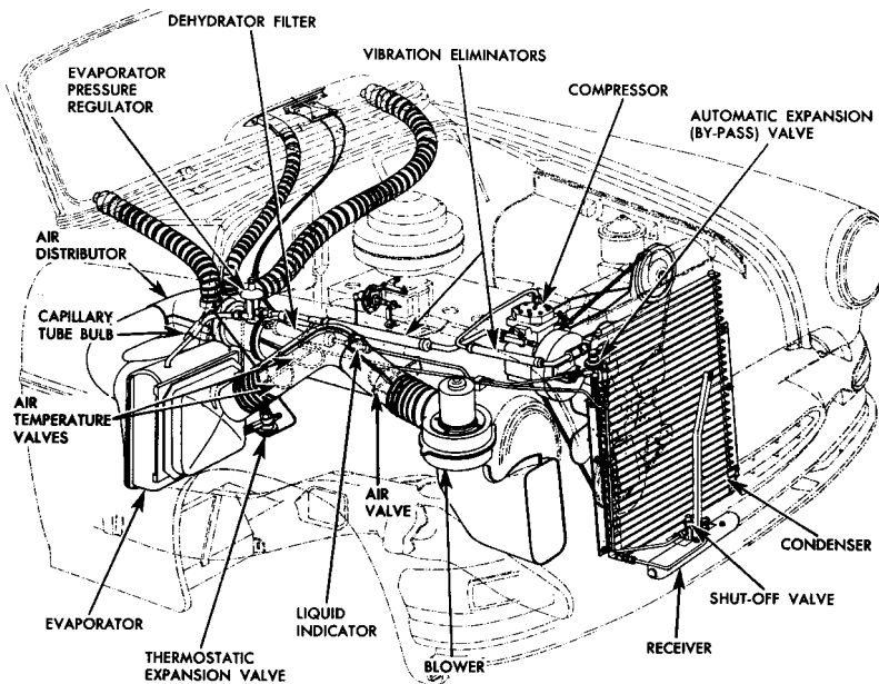
Figure 8: Underhood disposition of the components of the automotive air-conditioning system developed by Harrison Radiator and Pontiac Divisions of General Motors in 1953 that became an industry standard. 10
