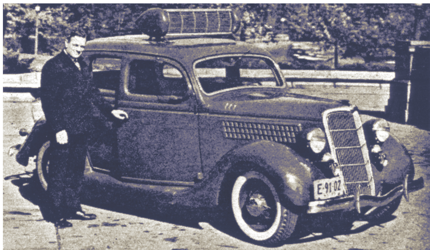
Figure 4: The Ford V-8 five-passenger car used in the feasibility study of bus air conditioning in 1934 by Houde Engineering of Buffalo, N.Y. and Carrier Engineering of Newark, N.J. 4
