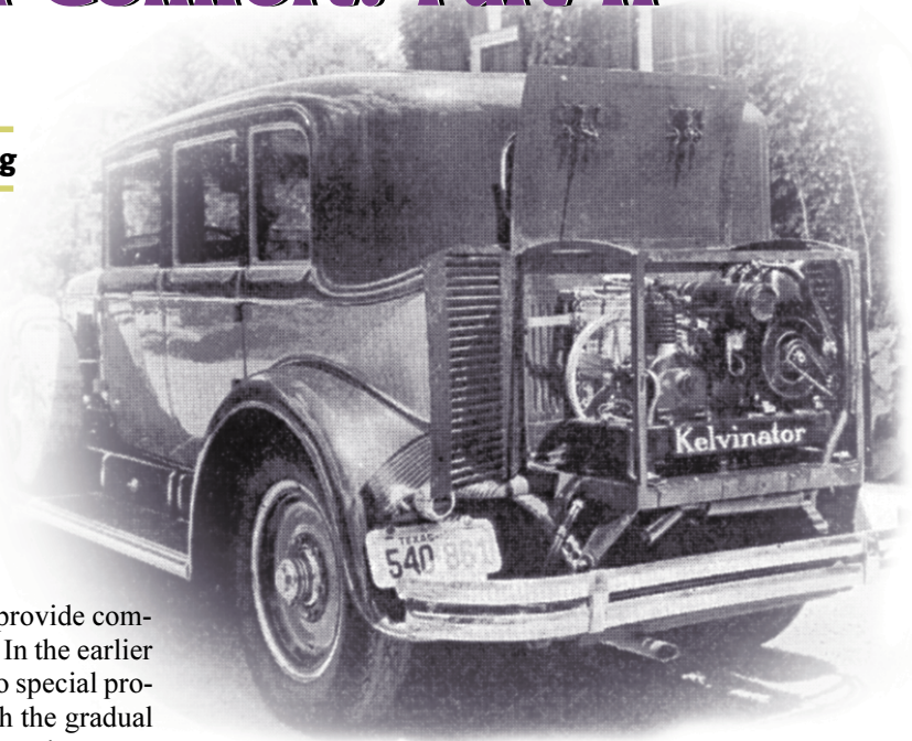
Figure 1: The first car air conditioned by C&C Kelvinator Co. for John Hamman Jr. of Houston, Texas in 1930. 2
