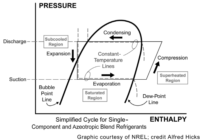
Figure G-1 Refrigerant Property Diagram—Azeotropic
