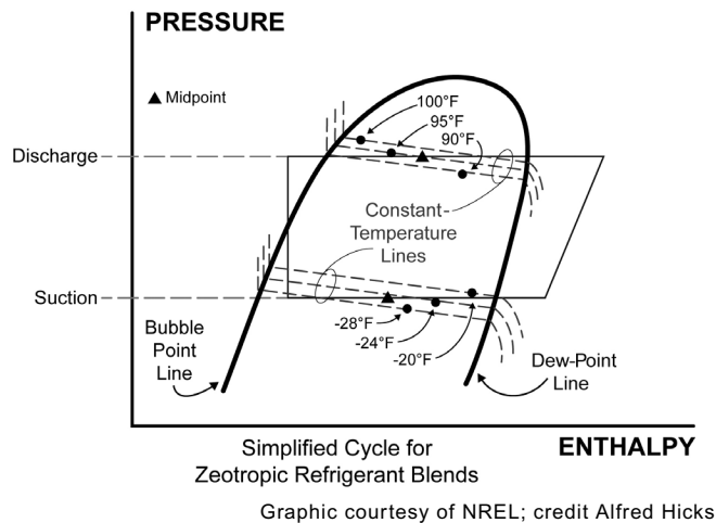
Figure G-2 Refrigerant Property Diagram—Zeotropic
