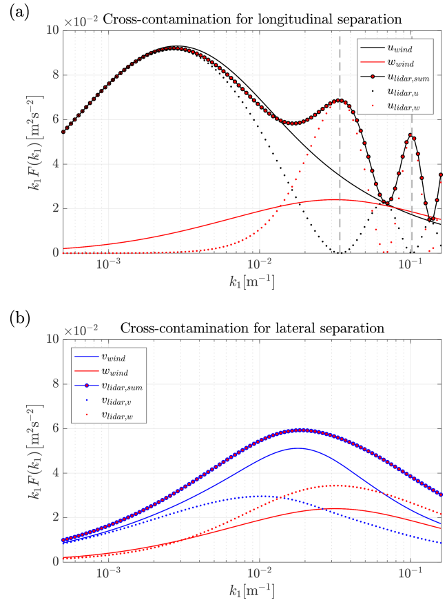
Figure 3. Modeled cross-contamination effect inherent in (a) the u spectrum from two longitudinally separated points with \Delta x = D_C and (b) the v spectrum from two laterally separated points with \Delta y = D_C . The solid lines are the spectra of the involved wind components. The dotted lines show the contribution of these wind components to the lidar spectra (circle markers). Averaging along the lines of sight is excluded.
