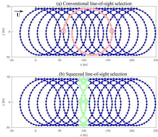
Figure 4. Selection of line-of-sight measurements for the reconstruction of one wind vector for when (a, in red) conventional VAD processing and (b, in green) the method of squeezed measurement circles is applied. Within the red and green segments, small red and green rings indicate the particular beams selected for two-beam processing. In this example, U = 19.5 \text{ m s}^{-1} , D_C = 92.3 \text{ m} and f_S = 1 \text{ Hz} .
