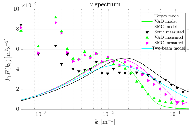
Figure 6. Modeled (solid lines) and measured (triangle markers) v spectra from all data processing methods. Colors correspond to processing method.
