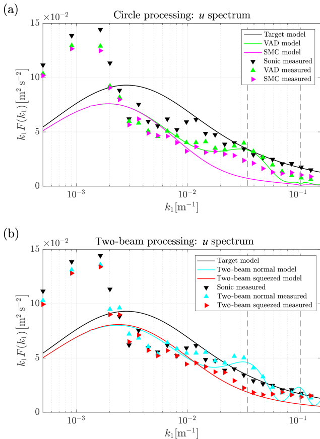
Figure 5. Modeled (solid lines) and measured (triangle markers) u spectra from data processing for which (a) all radial measurements are used and (b) only two beams are used. Colors correspond to the processing method. The grey vertical dashed lines represent the first and second resonance wave numbers.
