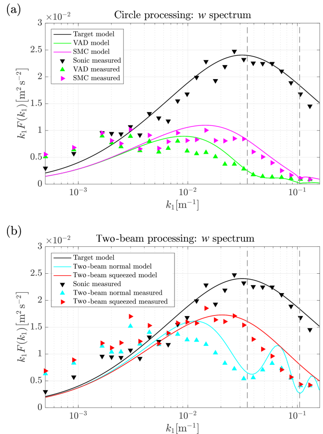
Figure 7. Modeled (solid lines) and measured (triangle markers) w spectra from data processing for which (a) all radial measurements are used and (b) only two beams are used. Colors correspond to processing method. The grey vertical dashed lines represent the first and second resonance wave numbers.
