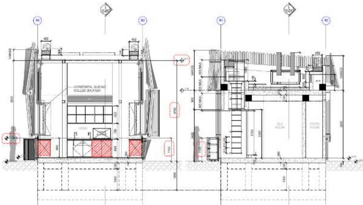
SECTION B
