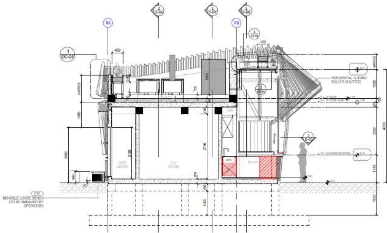
SECTION A
