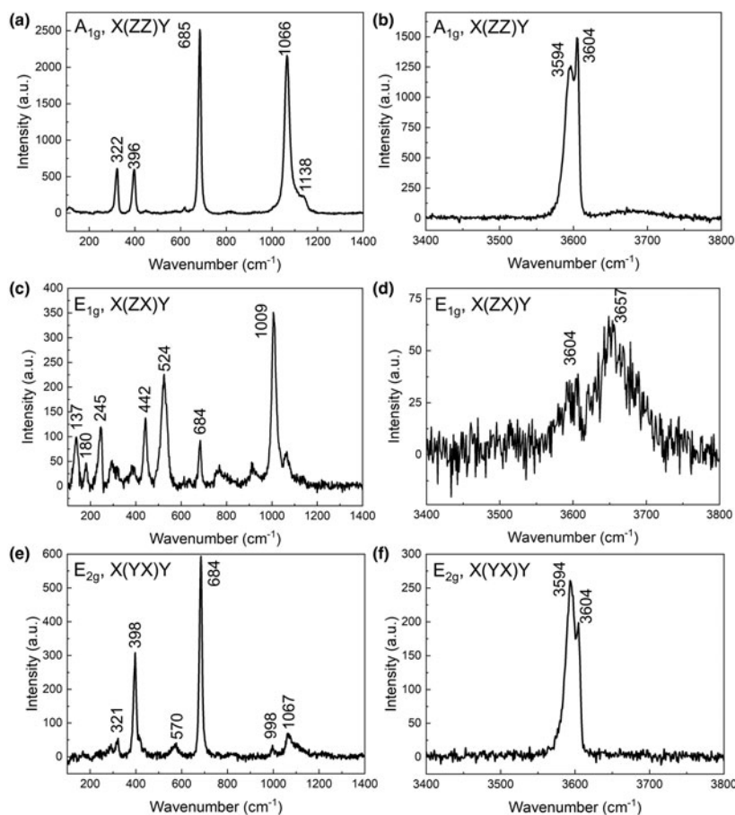
Fig. 9. Polarised Raman spectra of beryl. (a,b) k \perp c axis and E_{\text{inc}} \parallel c axis and E_{\text{R}} \parallel c axis, (c,d) k \perp c axis and E_{\text{inc}} \parallel c axis and E_{\text{R}} \perp c axis, (e,f) k \perp c axis and E_{\text{inc}} \perp c axis and E_{\text{R}} \perp c axis. k is the incident wave-vector, E_{\text{inc}} and E_{\text{R}} are the polarisation directions of the fundamental and Raman light, respectively. The crystallographic z axis is parallel to optical c axis. A_{1g} indicates the non-degenerate symmetric modes, E_{1g} / E_{2g} indicate the doubly degenerate symmetric modes. Peak assignments are listed in Table S6.
