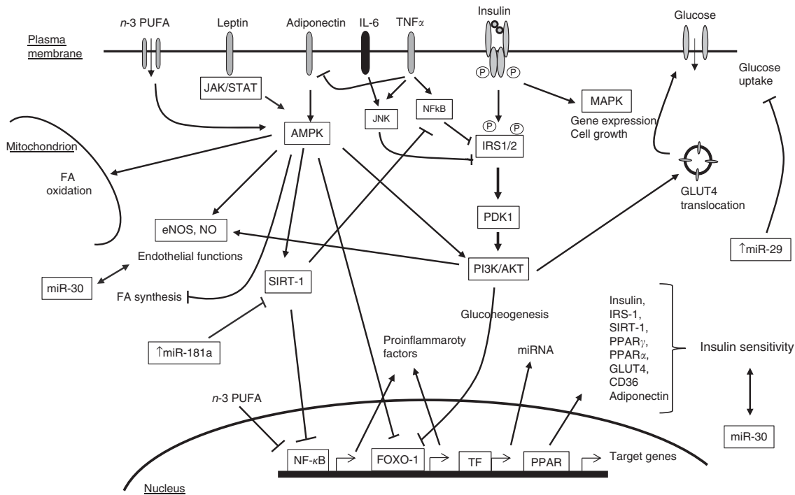
Fig. 2. Crosstalk among signalling pathways in regulating glucose metabolism. All of the factors that appear in this scheme are potential points of action of polyphenols. \longrightarrow , Activation; \longleftarrow , inhibition; \longleftrightarrow , modulation; JAK/STAT, Janus kinase/signal transducer and activator of transcription; AMPK, AMP-activated protein kinase; JNK, c-Jun N -terminal kinase; IRS1/2, insulin receptor substrate 1/2; MAPK, mitogen-activated protein kinases; PDK1, 3-phosphoinositide-dependent protein kinase-1; PI3K, phosphatidylinositol-3-kinase; Akt, protein kinase B; SIRT-1, sirtuin 1; NO, nitric oxide; eNOS, endothelial NO synthase; FOXO1, forkhead box protein O1; TF, transcription factors; miRNA, microRNA; FA, fatty acids.
