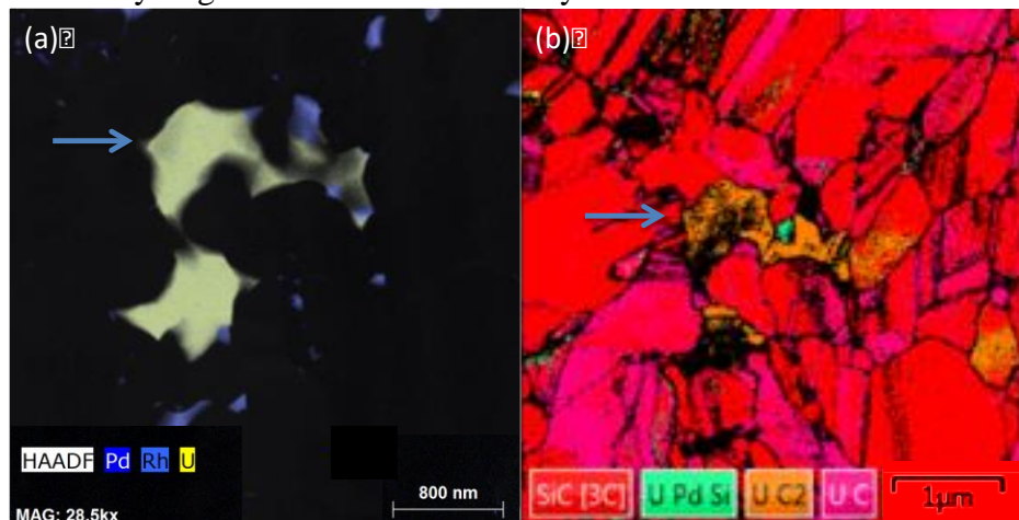
Figure 1. (a) STEM/EDS map of fission product precipitates at the boundaries of SiC grains. In this example, from the as-irradiated particle, uranium is shown both co-located with metallic fission products Pd and Rh, and on its own. (b) Is a tKD Euler micrograph of the same region, as indicated by the blue arrows. Preliminary results indicate UC 2 as the bulk uranium precipitate.
