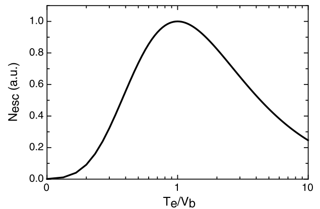
Figure 3. The number of escaping electrons per unit laser energy as a function of T_e/V_b .
