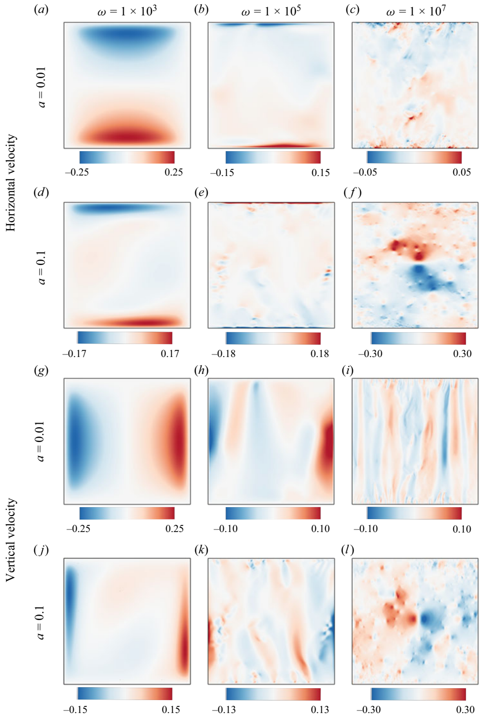
Figure 3. Typical snapshots of the horizontal velocity u/aw and vertical velocity w/aw fields for two different a , which are (a-c, g-i) a = 0.01 and (d-f, j-l) a = 0.1 , and for three different \omega , which are (a, d, g, j) \omega = 10^3 , (b, e, h, k) \omega = 10^5 and (c, f, i, l) \omega = 10^7 .
