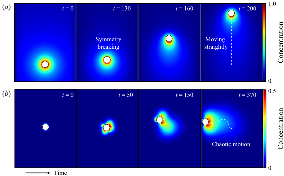
Figure 13. The concentration cross-section from three-dimensional simulations of an isotropic catalytic particle for Pe = 10 and 60; again, Sc = 1 . The simulation is at a domain L_x \times L_y \times L_z = 20R \times 20R \times 40R , in terms of the particle radius R . The grids are 201 \times 201 \times 401 . To better demonstrate the chaotic trajectory, the motion of the particle in panel (b) is projected to x - z plane. (a) Here Pe = 10 , the particle moves in a straight way; (b) Pe = 60 , plumes are generated at the surface of the particle, which starts to move irregularly.
