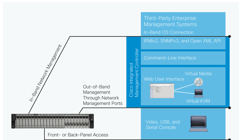
Figure 2 Cisco IMC Manages Standalone Servers Through Physical and Logical Interfaces
