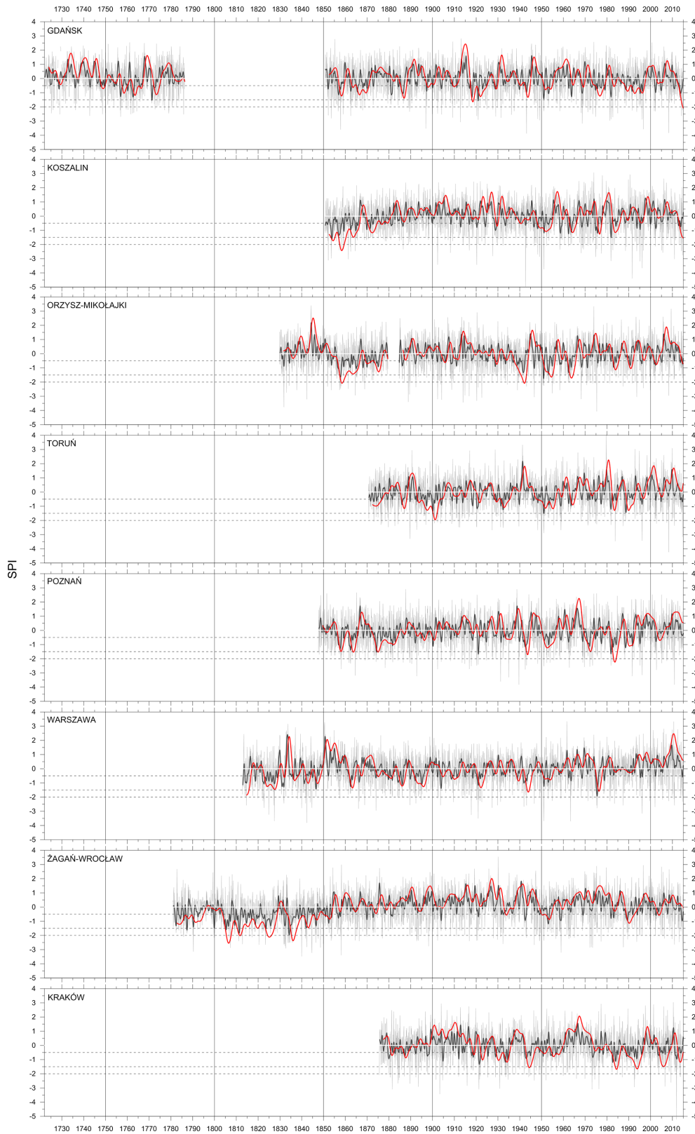
Figure 8. Variability in SPI: 1-month (grey curve), 3-month (black curve), and 24-month (red curve) variabilities calculated from the Polish instrumental series listed in Table 2 (oriented from north to south) in the period 1722–2015. SPI3 and SPI24 were filtered by 10-element and 30-element low-pass Gauss filters, respectively. Dashed lines indicate thresholds taken for distinguishing drought categories (see Sect. 3).
