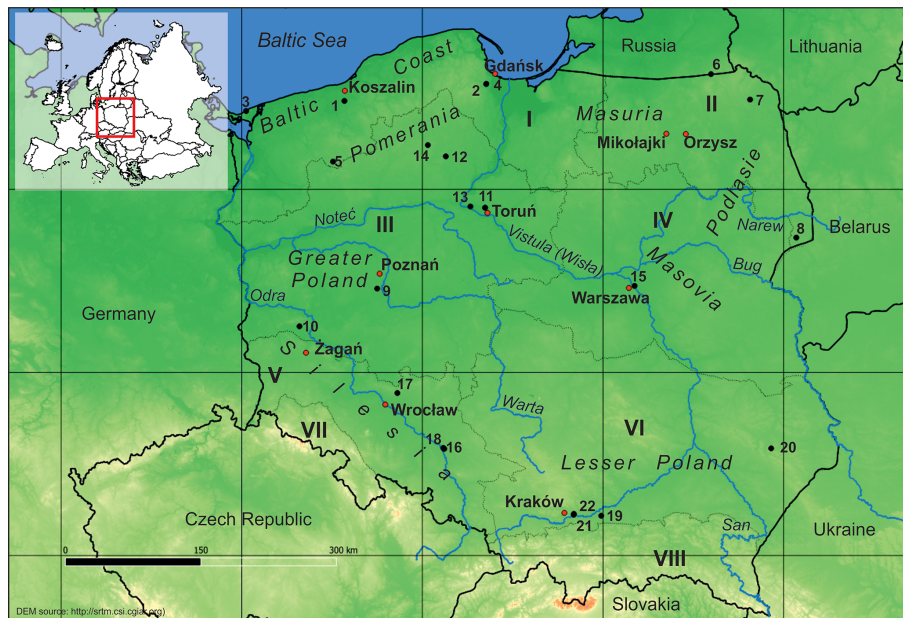
Figure 1. Location of dendrochronological sites and natural-forest regions (black dots and black dotted lines, respectively; for more details see Table 1) as well as meteorological series (red dots) and geographical regions (for more details see Table 2) used in the study.
