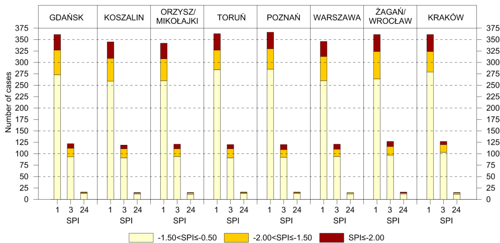
Figure 12. Frequencies of dry months (SPI1), short-term droughts (SPI3), and long-term droughts (SPI24) in Poland, including three intensity categories calculated using Łabędzki's formula.
