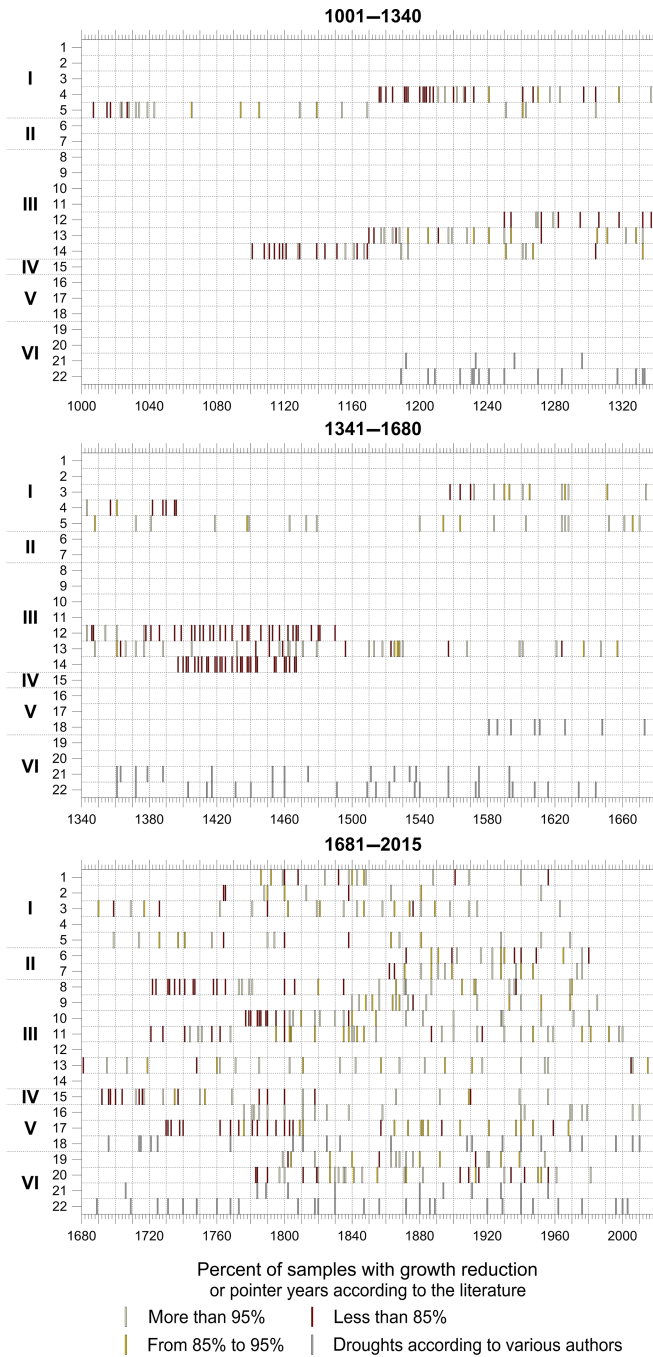
Figure 6. Pointer years in Poland (1001–2015).
