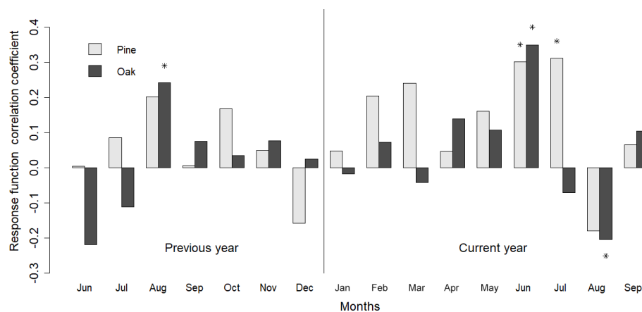
Figure 2. Climate growth relationships between tree rings in pine (grey bars) and oak (black bars) and monthly totals of precipitation. Key: asterisks indicate statistically significant correlation coefficients at the level of 0.05. Climate data were taken from Toruń Meteorological Station.
