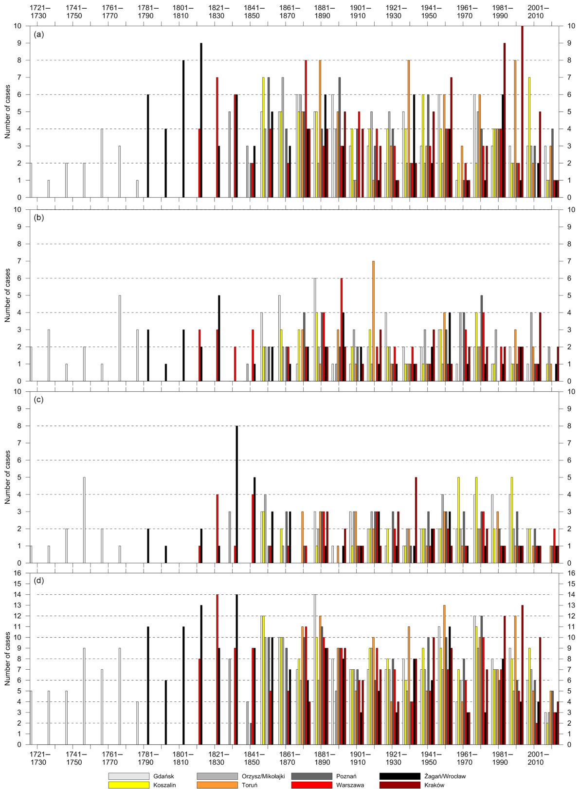
Figure 9. Decadal frequency of droughts in Poland in 1722–2015 identified using SPI1. Key: (a) moderate droughts, (b) severe droughts, (c) extreme droughts, and (d) all-category droughts.
