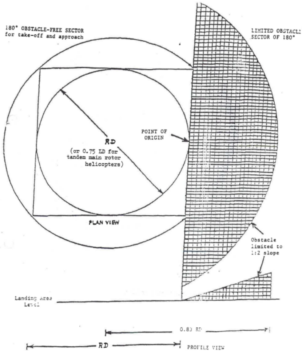
Figure 13-4 – Helideck obstacle limitation sector: 180^\circ for moderate climate
