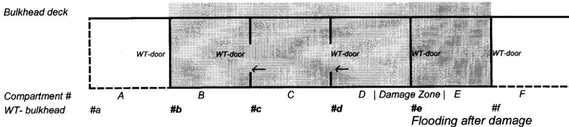
Figure 2 – Two-compartment ship
