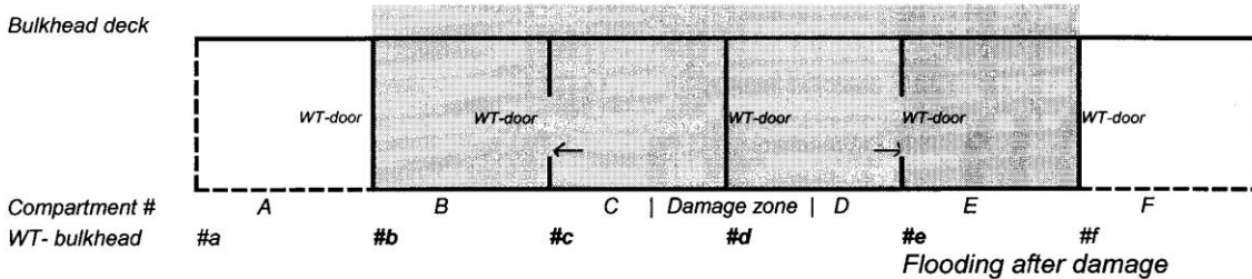
Figure 1 – Two-compartment ship
