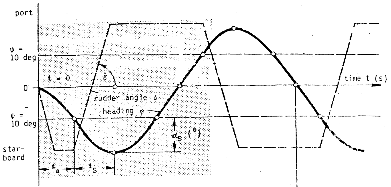
Fig.2 - Most important part of zig-zag test (example of 20^\circ/10^\circ zig-zag test)
