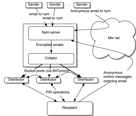
Figure 1: The Pynchon Gate Architecture
