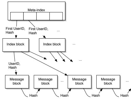
Figure 2: The meta-index and bucket pool
