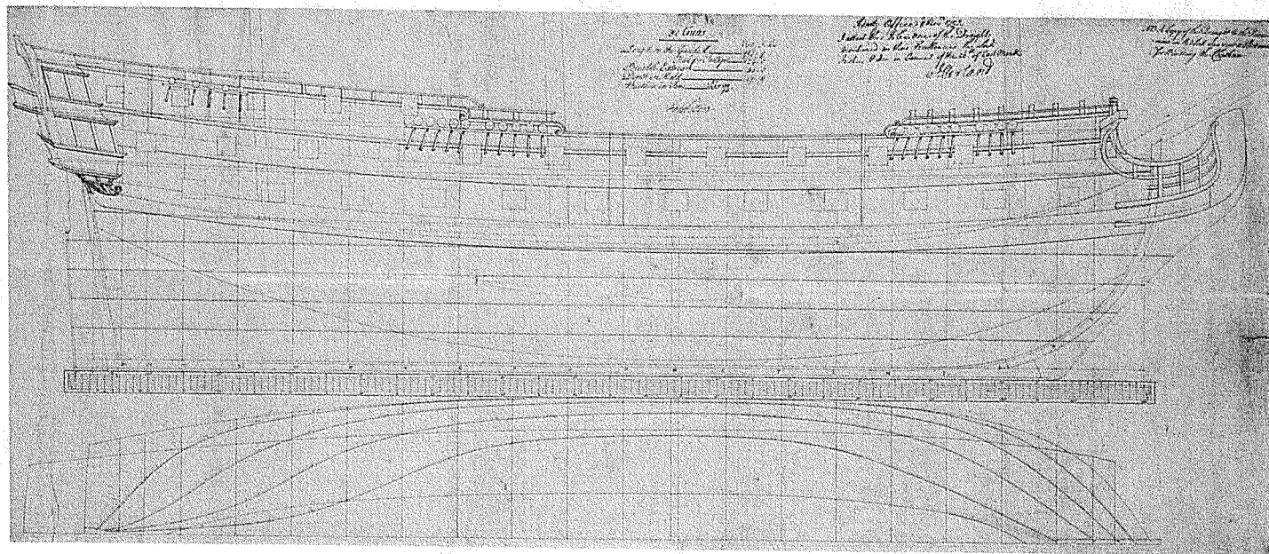
Draft of HMS Chatham.
