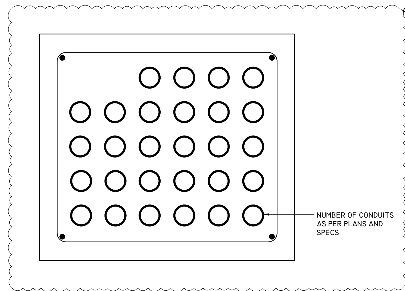
DETAIL - SECTION "A" NOT TO SCALE 6
