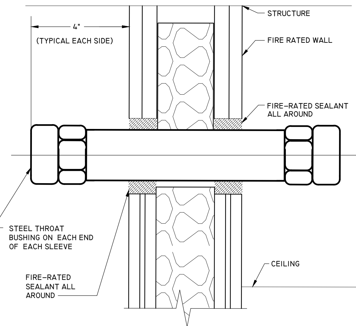
DETAIL - WALL SLEEVE NOT TO SCALE 2
