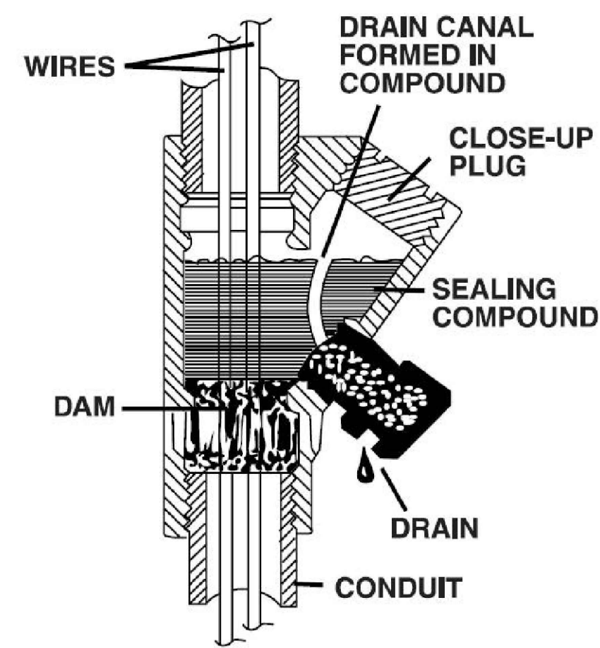
DETAIL - CONDUIT SEALING FITTINGS NOT TO SCALE 5
