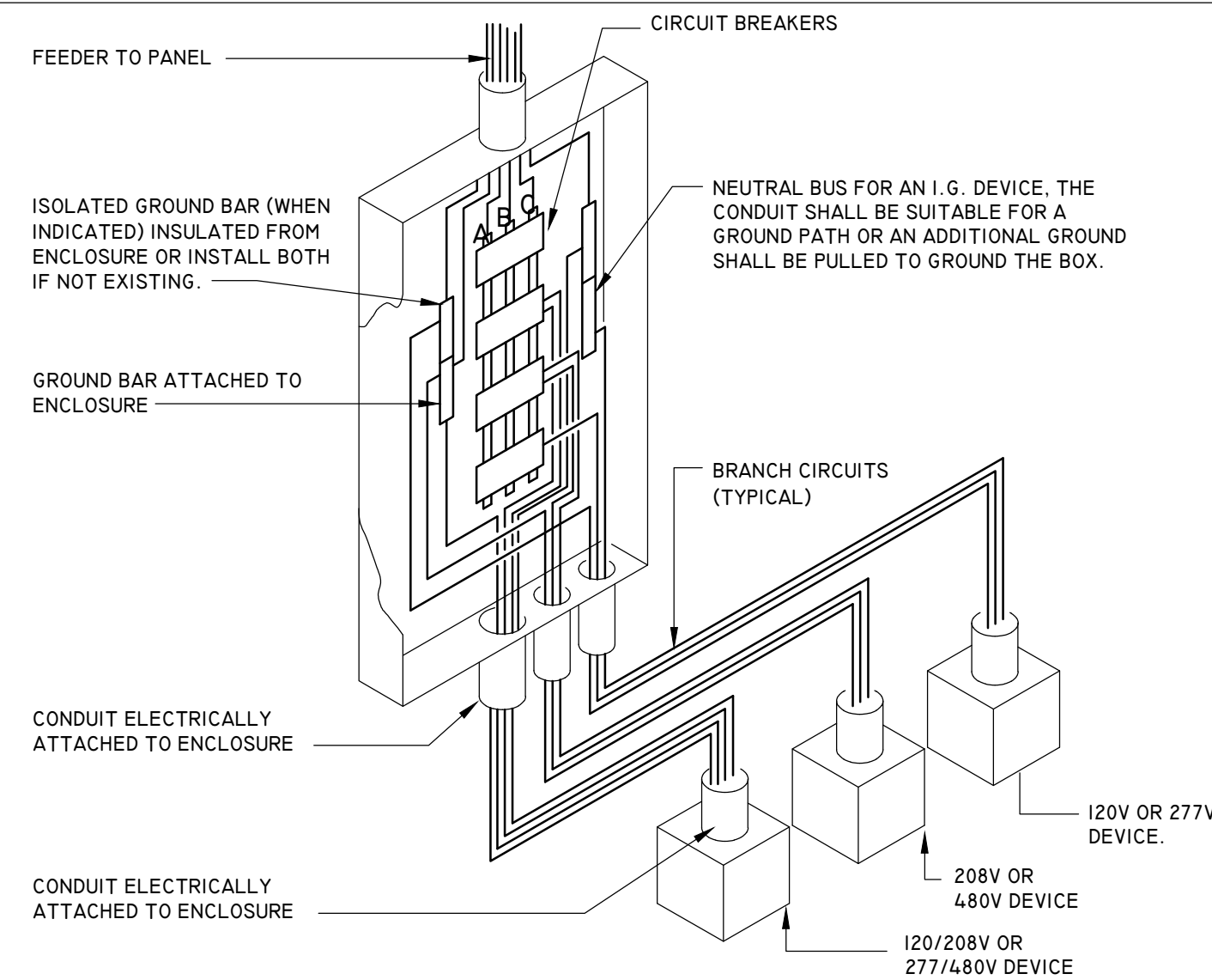
DETAIL - PANEL GROUNDING NOT TO SCALE 3
