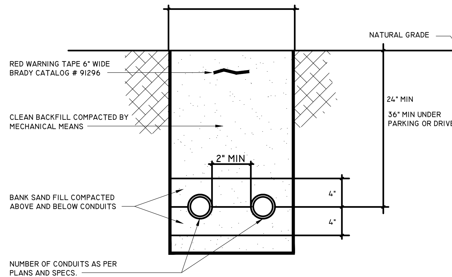
DETAIL - TRENCH (OTHER THAN SERVICE) NOT TO SCALE 1
