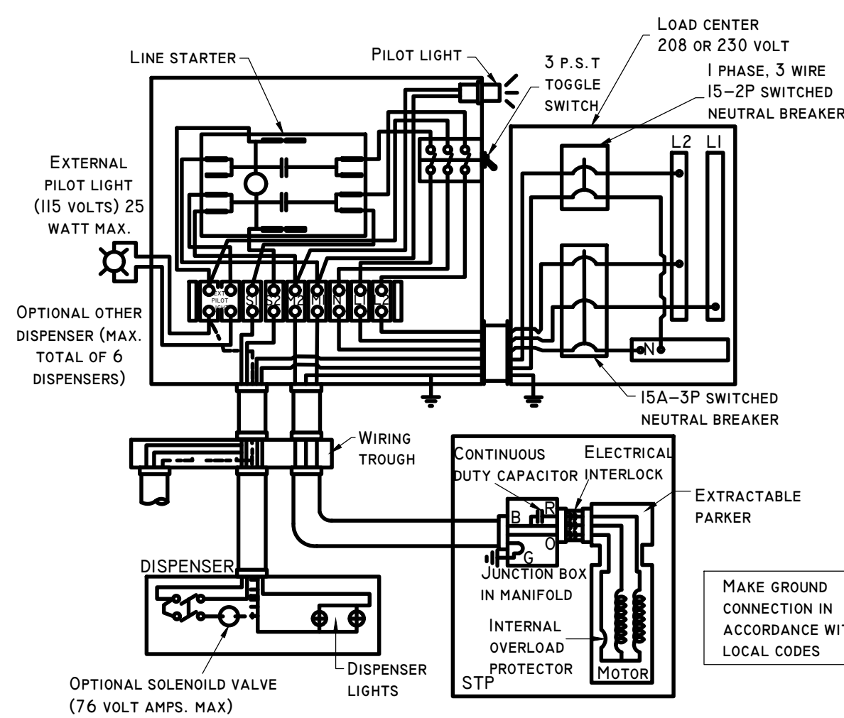
DETAIL - FROM THE PANEL TO THE RED JACKET STP NOT TO SCALE 4
