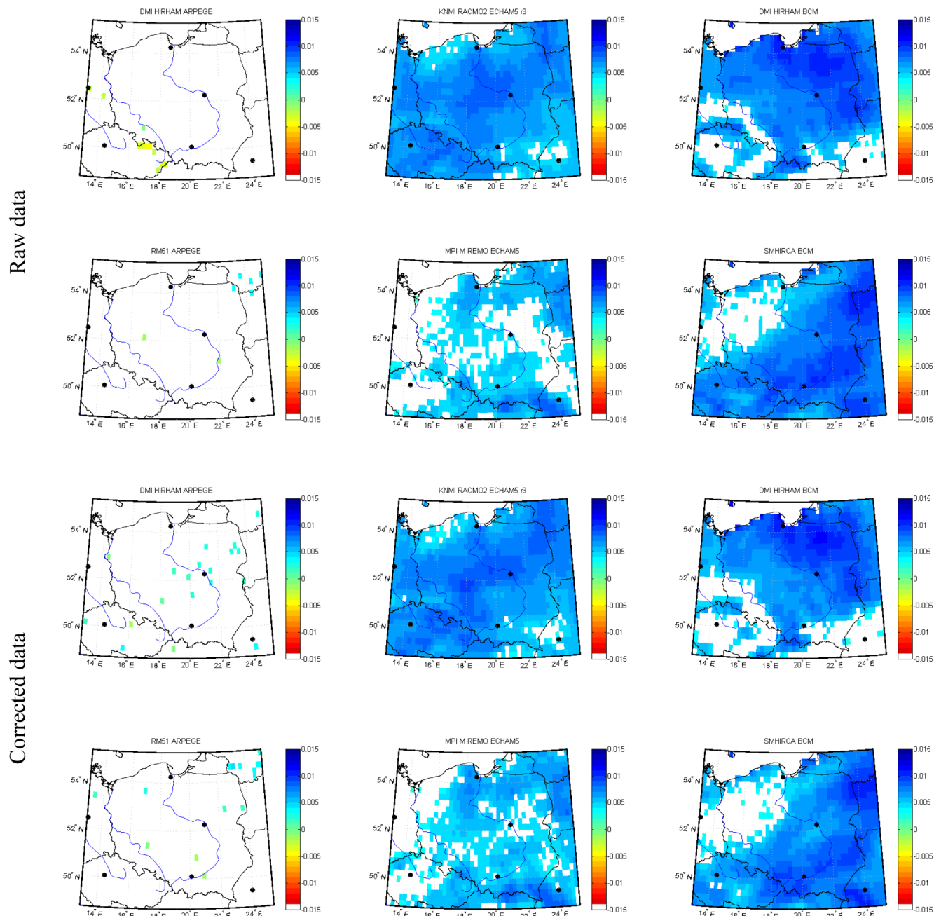
Figure 8. The results of the Mann–Kendall trend analysis for SPI 1 for January. The colour scale denotes the slope of the estimated trend. White colour indicates a lack of a statistically significant trend.
