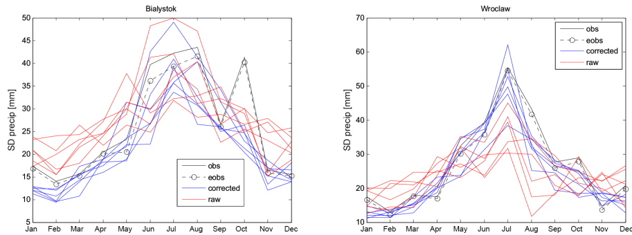
Figure 4. Comparison of standard deviation of monthly sum of precipitation calculated over the reference time period for two grid cells located close to Białystok (NE Poland) and Wrocław (SW Poland). The black continuous line denotes observations from meteorological stations, black dashed lines denote observations from the E-OBS reanalysis, red lines denote precipitation values from uncorrected RCMs, and blue lines denote bias corrected RCM precipitation data.
