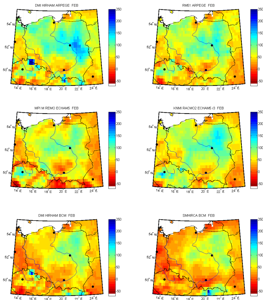
Figure 5. Comparison of spatial patterns of differences in the standard deviation of monthly precipitation for February for uncorrected relative to corrected RCM data for the month of February for the reference period 1971–2000.
