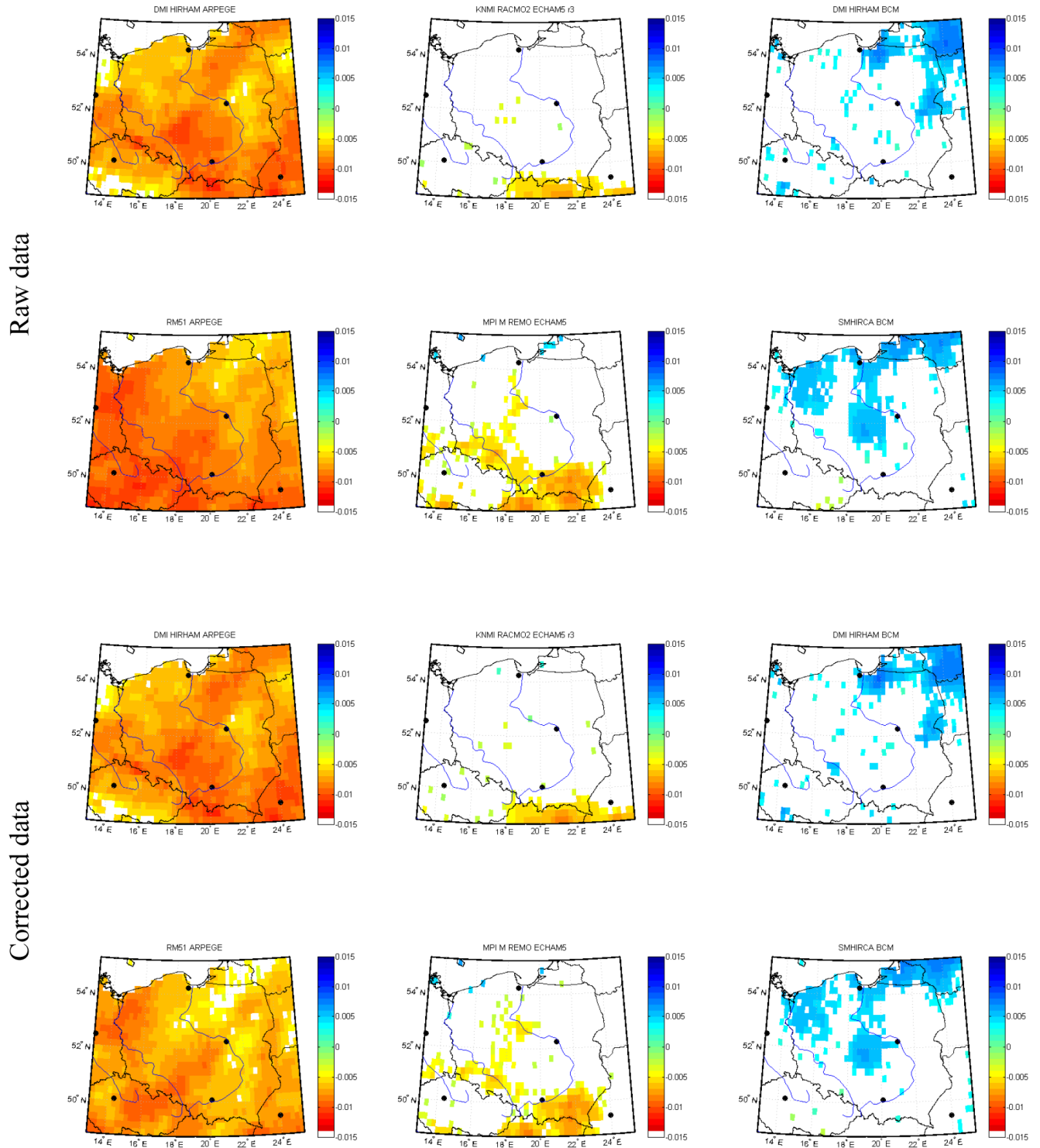
Figure 9. Results of the modified Mann–Kendall test for SPI 1 for July. Colour scale denotes the slope of the estimated trend. White areas indicate a lack of a statistically significant trend.
