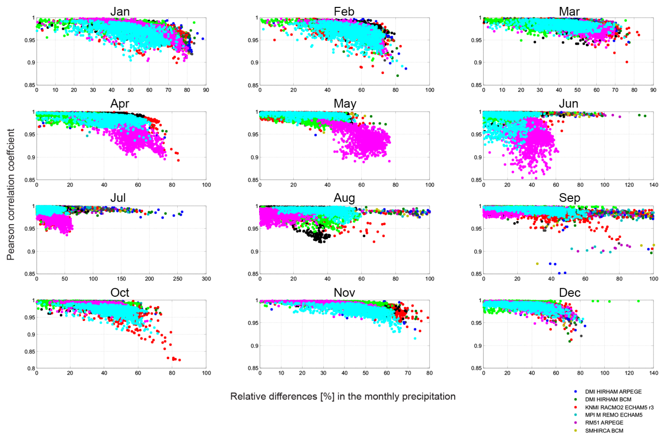
Figure 15. The scatter plots showing relationship between relative differences in the raw and corrected monthly sum of precipitation and Pearson correlation coefficient estimated for raw and corrected SPI 1 values for all grid cells.
