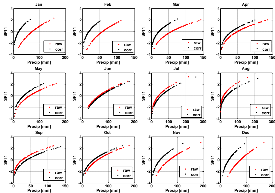
Figure 14. The scatter plots showing relationship between monthly sum of precipitation and estimated SPI 1 values for one grid cell located close to Białystok (NE Poland) for DMI HIRHAM ARPEGE model. The colour denotes type of data used, red colour – uncorrected precipitation and SPI 1, black corrected ones.
