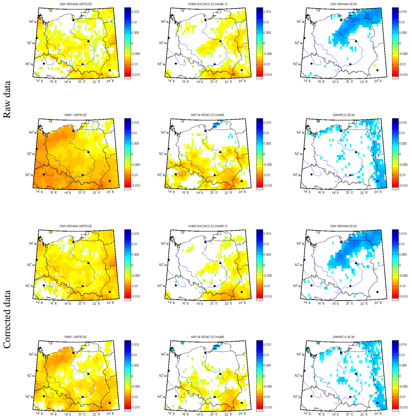
Figure 12. Trend for the SPI 3 for the summer period (JJA). The colour scale denotes the slope of the estimated trend. The white areas indicate the lack of a statistically significant trend.
