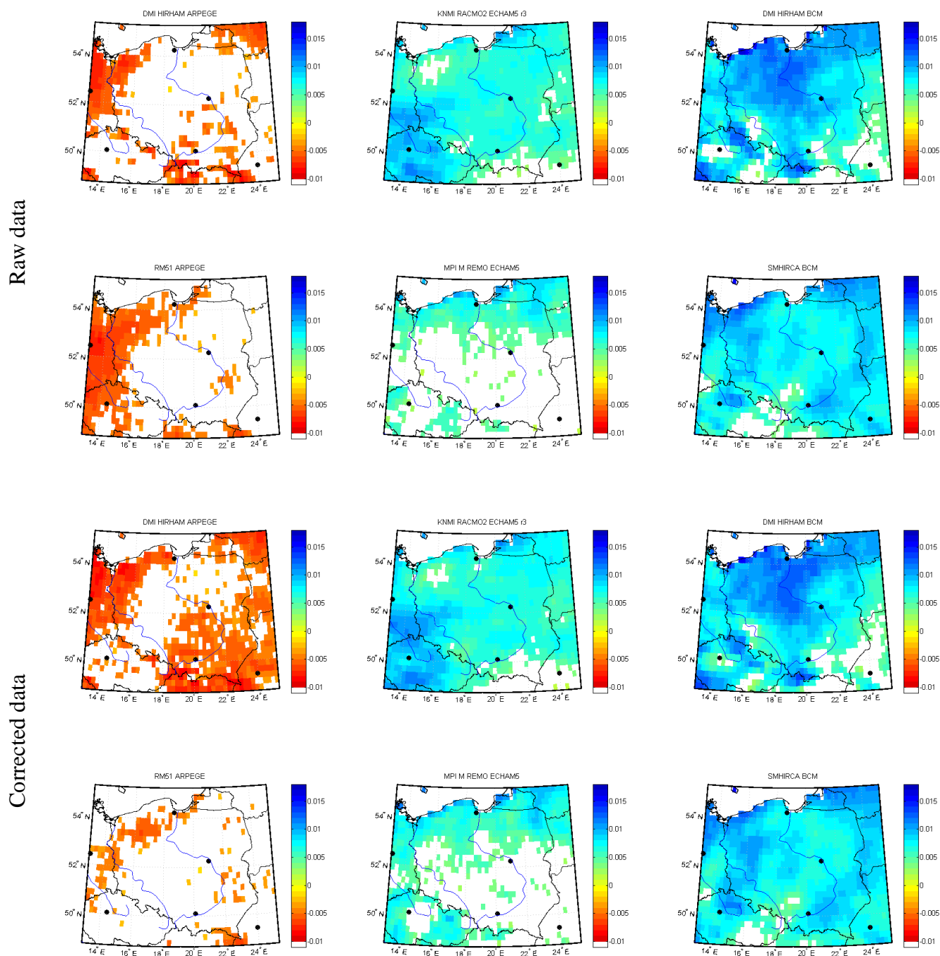
Figure 13. Trends in the SPI 12. Colour scale denotes the slope of the estimated linear trend. White areas indicate the lack of statistically significant trend.
