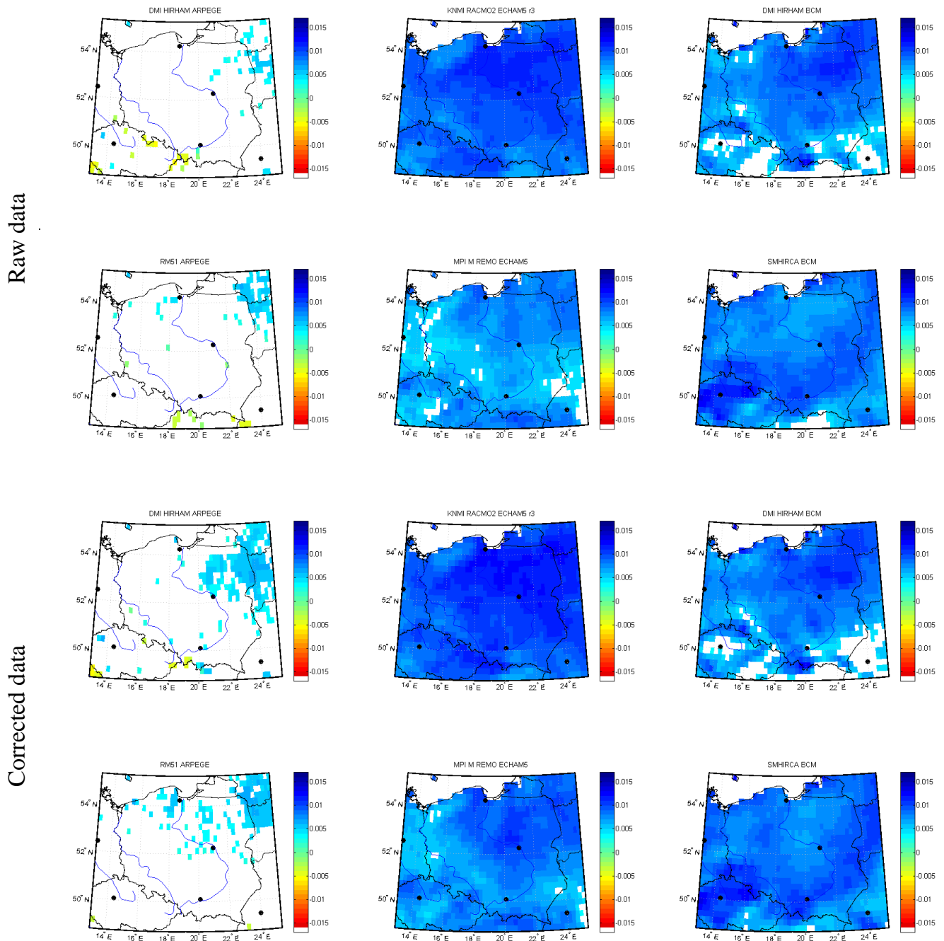
Figure 11. Results of the trend estimation using the Mann–Kendall method for the SPI 3 for the winter season (DJF). Colour scale denotes slope of the estimated trend. White colour denotes lack of statistically significant trends.
