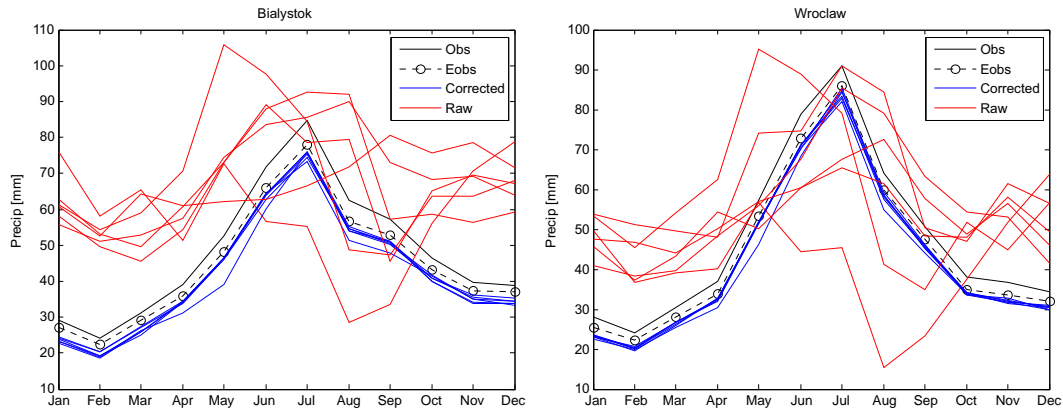
Figure 2. Comparison of mean monthly sums of precipitation calculated over the reference time period for two grid cells located close to Białystok (NE Poland) and Wrocław (SW Poland). Black continuous lines denote observations from meteorological stations, dashed lines denote observations from E-OBS reanalysis grid cells, red lines denote uncorrected precipitation series from the RCMs, and blue lines denote the bias corrected precipitation series.
