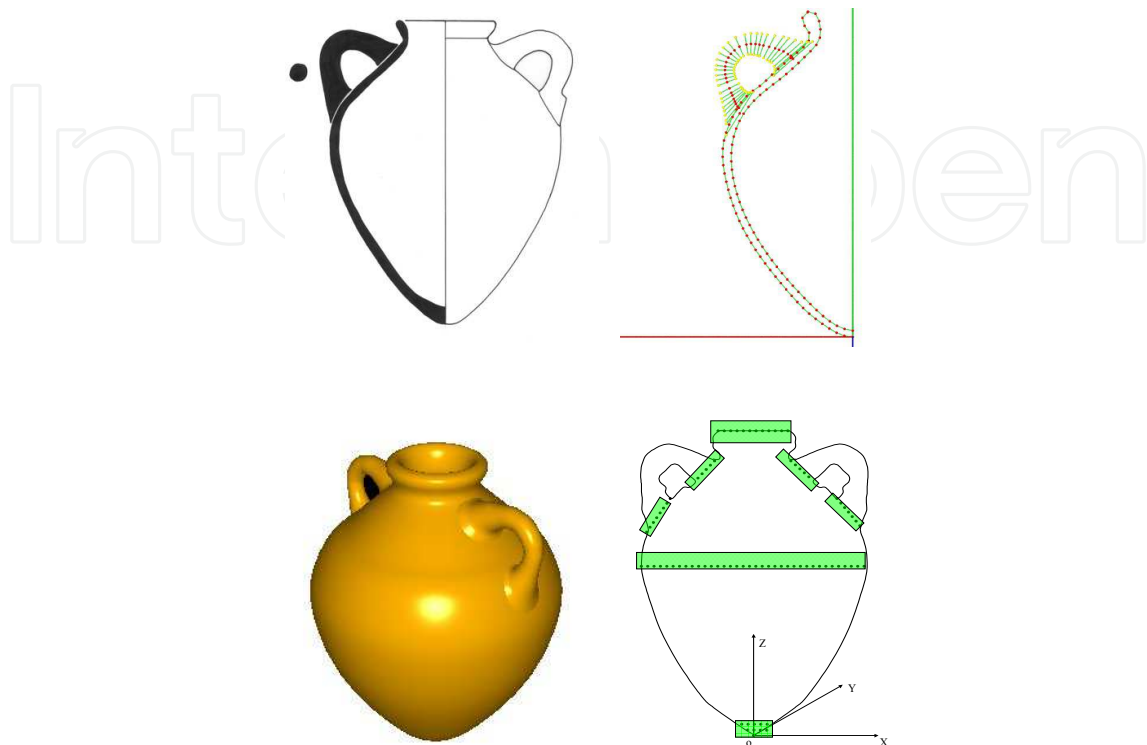
Fig. 1. On the left, the graphical model designed until now by archaeologists. On the middle two images, a CAD interpretation of this model. On the right, the five zones where photogrammetric measurements can be taken on an amphora.
