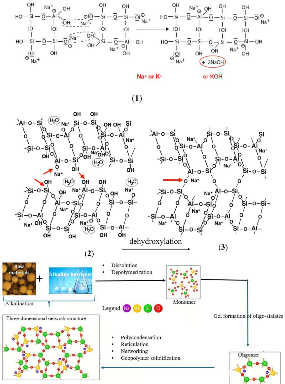
Figure 4. Alkali-aluminosilicate geopolymerization process [20].
