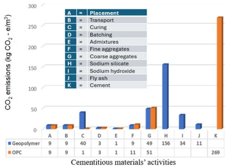
Figure 6. Illustration of the CO 2 -e emissions of concrete mixtures utilizing Portland cement or GPC [120].
