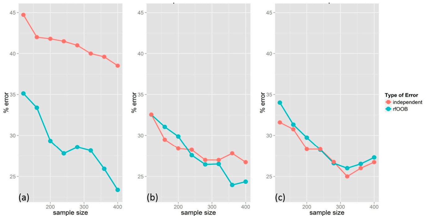
Figure 8. Mean of rfOOB and independently assessed error for 25 iterative classifications varying the sample size with All Variables (a), Important Variables (b), and Uncorrelated Important Variables (c).
