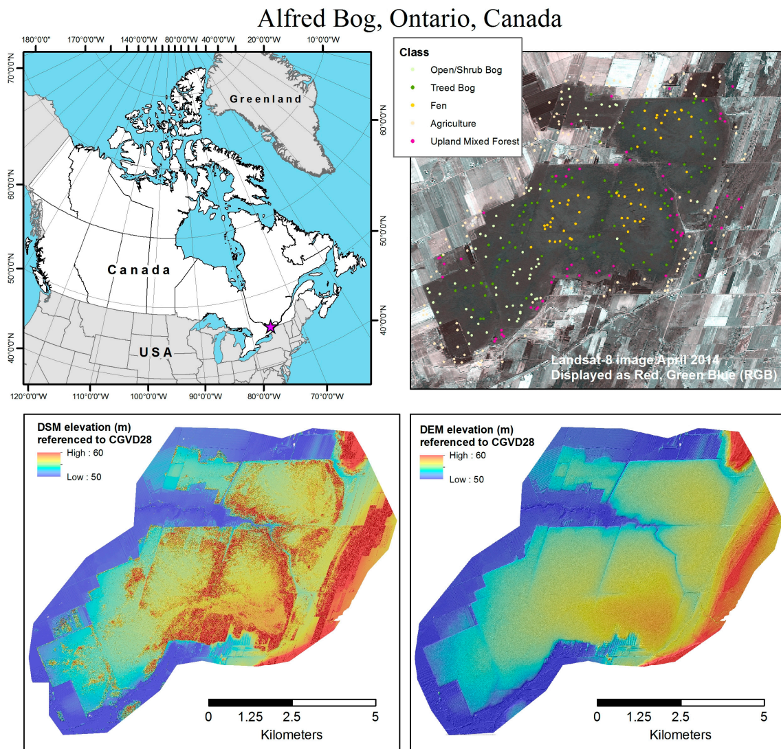
Figure 1. Study area map. Top left shows location within Canada (purple star). Top right shows Landsat-8 4-3-2 red/greed/blue image with training data points overlain. Bottom left shows LiDAR Digital Surface Model (DSM). Bottom right shows LiDAR Digital Elevation Model (DEM).
