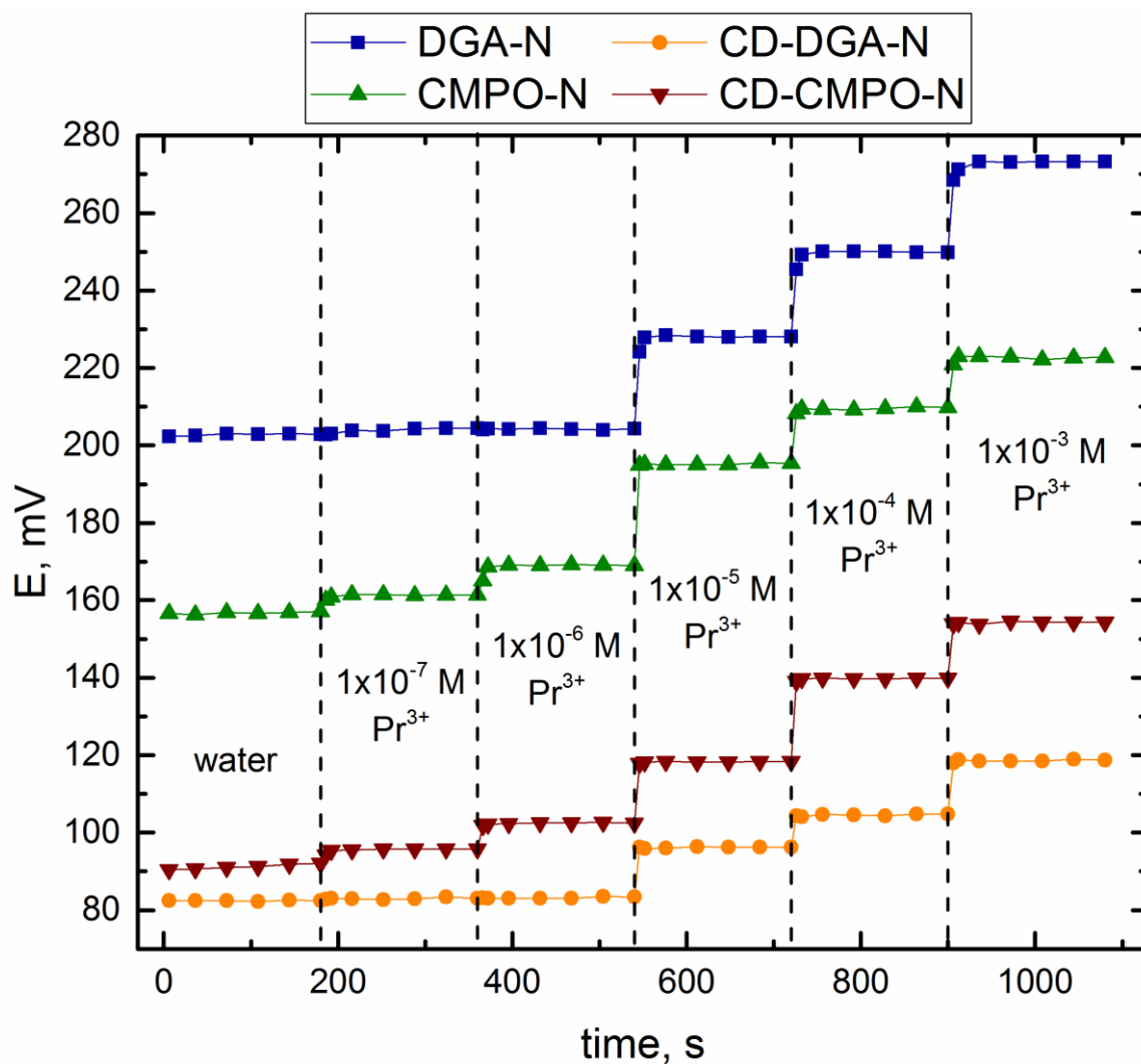
Figure S1. Dynamic response of the sensors DGA-N, CD-DGA-N, CMPO-N, CD-CMPO-N in presence of the praseodymium cations.
