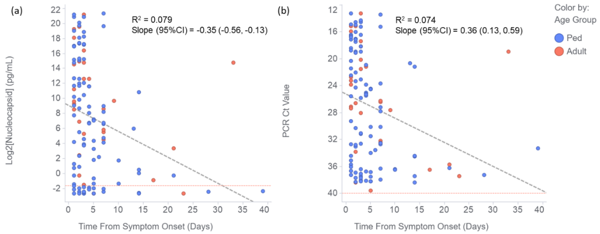
Figure 3. Correlation of (a) nucleocapsid concentration (log2-transformed) and (b) PCR Ct value with time from symptom onset for clinical NP swab samples from PCR-positive adults (red circles) and children (Ped, blue circles). The plots also show the linear regression fit to the data (diagonal dashed grey lines).
