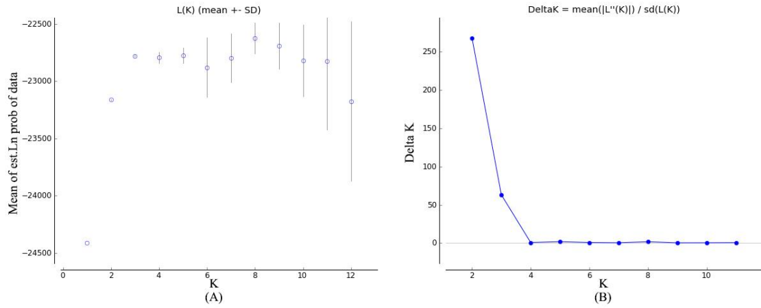
Supplementary file S3. Optimal K value estimated by likelihood of the probability of data L(K) (A) and Delta K (B)
