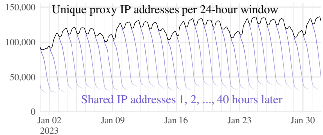
Figure 7: Proxy churn in January 2023. The dark upper line shows the number of unique proxy IP addresses in overlapping 24-hour windows. The lighter, descending lines indicate how many of the same IP addresses were in later 24-hour windows, at 1-hour increments up to 40 hours later. It takes about 20 hours for 50% of the proxy pool to turn over.
