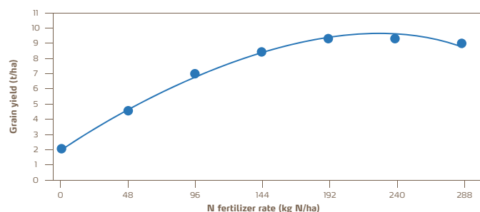
Figure 4: Yield response of winter wheat to increasing N fertilizer rates identifies an optimum rate after which yields decline. Source: F. Brentrup et al, 2004. 22
