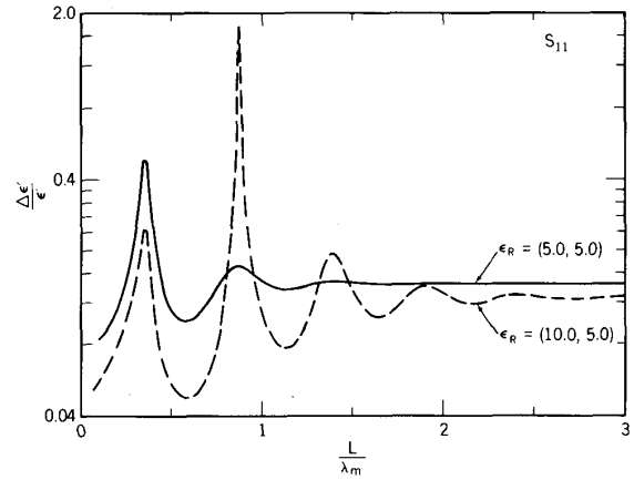
Fig. 8. The relative uncertainty in \epsilon_R^k(\omega) for S_{11} (25) as a function of frequency for a high-loss material as a function of normalized length with \epsilon_R^k = (5.0, 5.0) in solid line and (10.0, 5.0) in dashed line. The S -parameter uncertainties are the same as in Fig. 4. (See footnote 1.)
