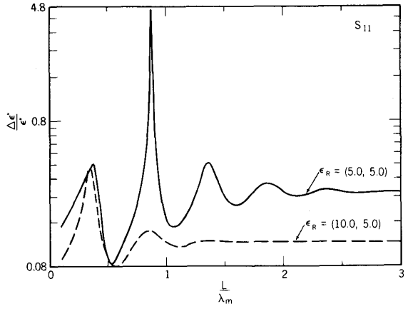
Fig. 9. The relative uncertainty in \epsilon_R^k(\omega) for S_{11} from (26) as a function of frequency for a high-loss material as a function of normalized length with \epsilon_R^k = (5.0, 5.0) in solid line and (10.0, 5.0) in dashed line. The S -parameter uncertainties are the same as in Fig. 4. (See footnote 1.)
