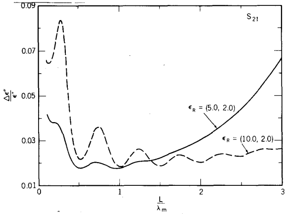
Fig. 7. The relative uncertainty in \epsilon_R^k(\omega) for S_{21} from (26) as a function of frequency for a high-loss material as a function of normalized length, for \epsilon_R^k = (5.0, 2.0) in solid line and (10.0, 2.0) in dashed line. The S -parameter uncertainties are the same as in Fig. 4. (See footnote 1.)
