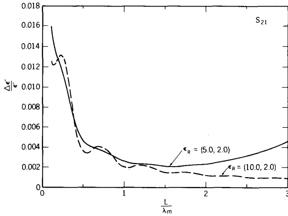
Fig. 6. The relative uncertainty in \epsilon_R^k(\omega) for S_{21} from (25) as a function of frequency for a high-loss material as a function of normalized length, with \epsilon_R^k = (5.0, 2.0) in solid line and (10.0, 2.0) in dashed line. The S -parameter uncertainties are the same as in Fig. 4. (See footnote 1.)
