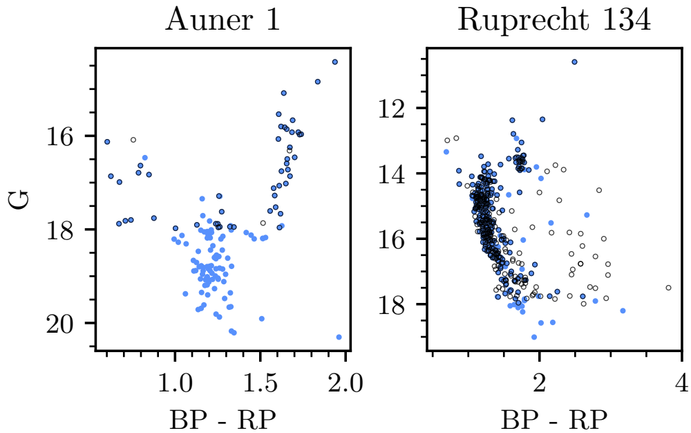
Fig. 3.1.: Comparison of cluster membership lists detected using Gaia DR3 data cut at G < 18 (black empty circles) and a Rybizki et al. 2022 v1 criterion greater than 0.5 (blue filled circles) using separate runs of HDBSCAN and our pipeline for each cut, shown for Auner 1 (left) and Ruprecht 134 (right).
