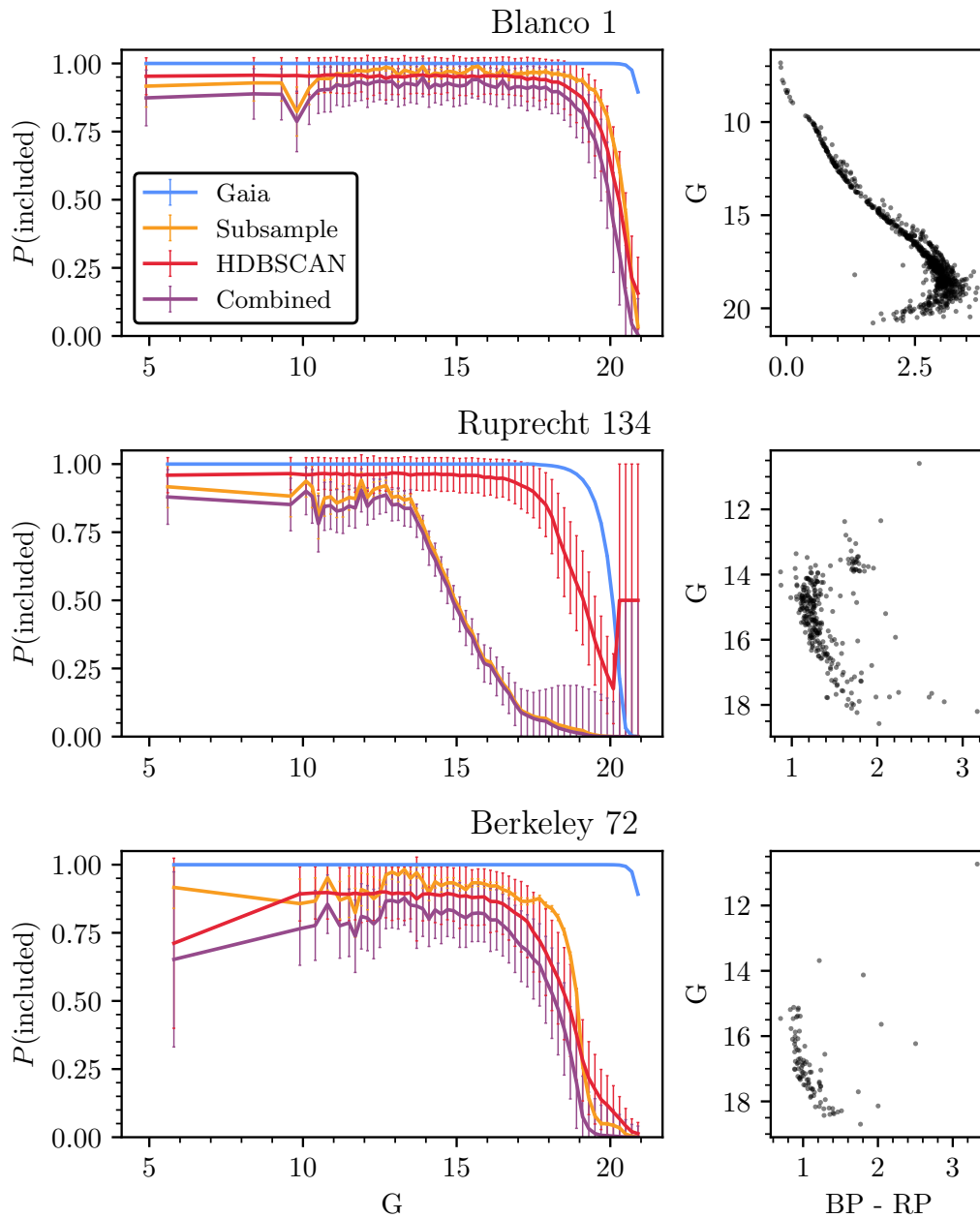
Fig. 4.2.: Estimated cluster selection functions for three OCs from Paper 2: Blanco 1, Ruprecht 134, and Berkeley 72. The left column shows computed cluster selection functions and a combined cluster selection function after accounting for all three dominant selection effects. The right column shows the CMD of each considered cluster for comparison.
