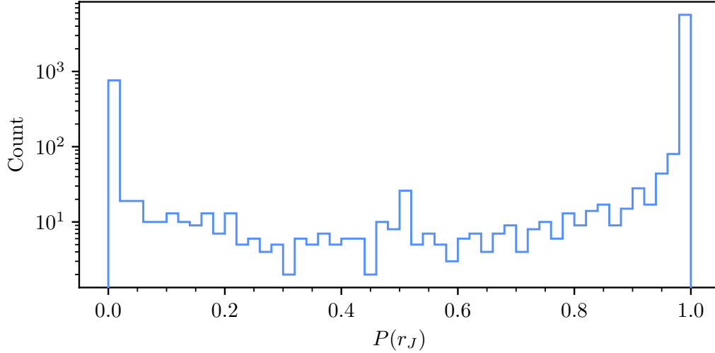
Fig. 4.8.: The distribution of probabilities that a cluster has a valid Jacobi radius for all clusters within 15 kpc.
