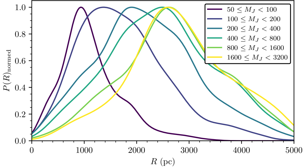
Fig. 4.14.: Distance distribution of the clusters in this work divided into multiple mass bins. Cluster distance probability distributions P(d) are smoothed using kernel density estimation, and normalised to all have a peak of one.
