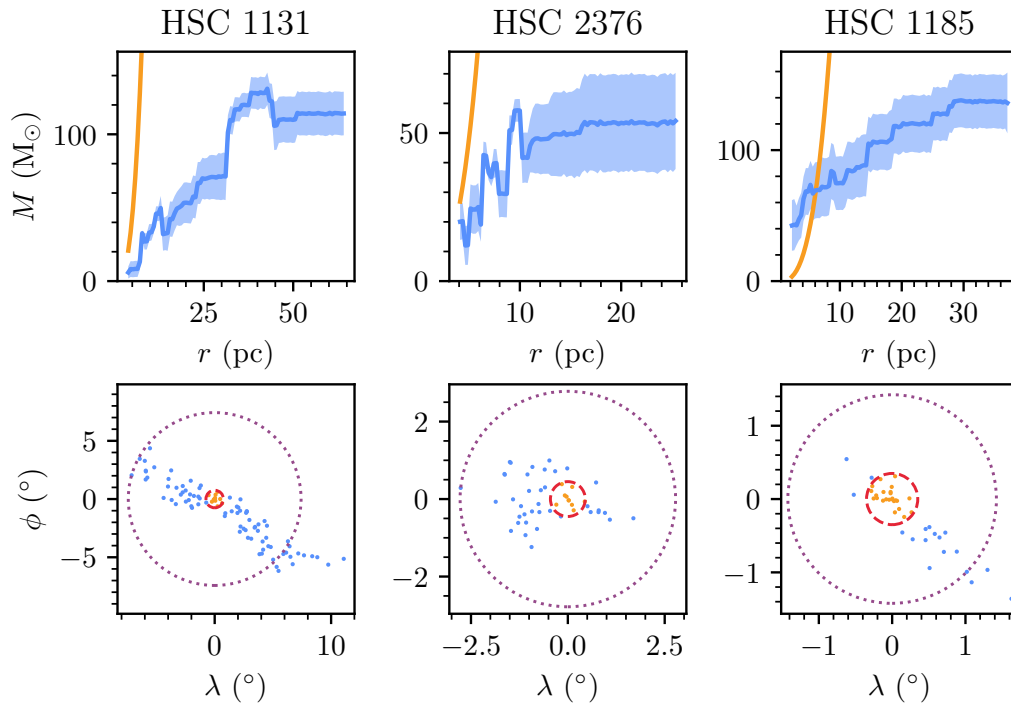
Fig. 4.5.: Jacobi radius determination for three candidate new OCs from Paper 2 that were highlighted as example new objects (see Sect. 3.9 and Fig. 3.17). The plot is formatted the same as Fig. 4.4. The most likely Jacobi radius for HSC 1131 and HSC 2376 is shown, although M_{\text{obs}}(r) < M_J(r) for all radii for both clusters, and they are hence more likely to be MGs (see text).
