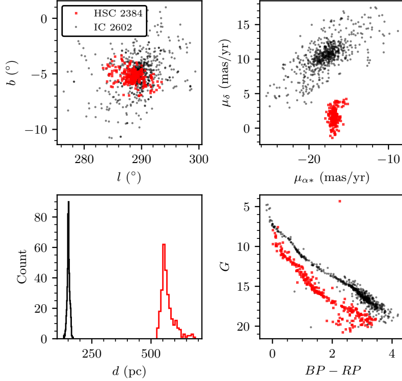
Fig. 3.8.: Member stars for the candidate new cluster HSC 2384 (red squares) compared against the nearby cluster IC 2602 (black circles). Four plots of are shown, comparing positions (top left), proper motions (top right) and photometry (bottom right). The bottom left plot shows a histogram of all distances to individual member stars.
