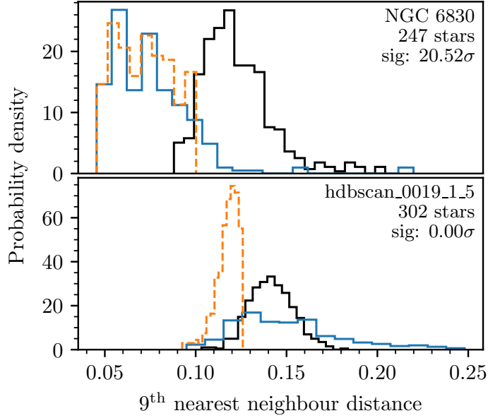
Fig. 2.5.: Two examples of NNDs used to test the significance of OC candidates. The solid black line shows the NND of nearby field stars. The blue line shows the NND of distances between cluster members. For a cluster to be significant and not simply a selection of unclustered field stars, the cluster NND must be incompatible with being drawn from the field distribution. For later illustrative purposes, the NND of a cluster member to the nearest field star is shown by the dashed orange line, although this is not used for the CST. In the upper plot, an OC candidate detected by HDBSCAN and crossmatched to the well-characterised OC NGC 6830 is shown, which has a clearly different NND to field stars with a significance of over 20\sigma . In the lower plot, a false positive OC detected by HDBSCAN in field 19 is shown that has a significance of 0\sigma .
