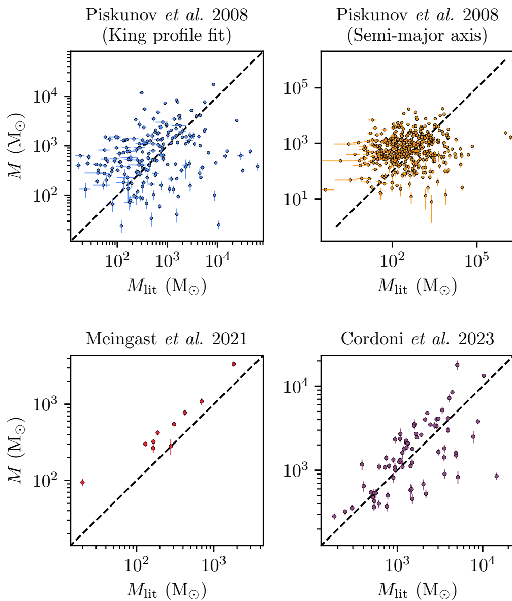
Fig. 4.7.: Cluster masses derived in this work compared against masses derived in Piskunov et al. 2008, Meingast et al. 2021, and Cordoni et al. 2023 for clusters that appear in both this work and the literature work. Values on the dashed line y = x are in agreement between this work and the literature work.
