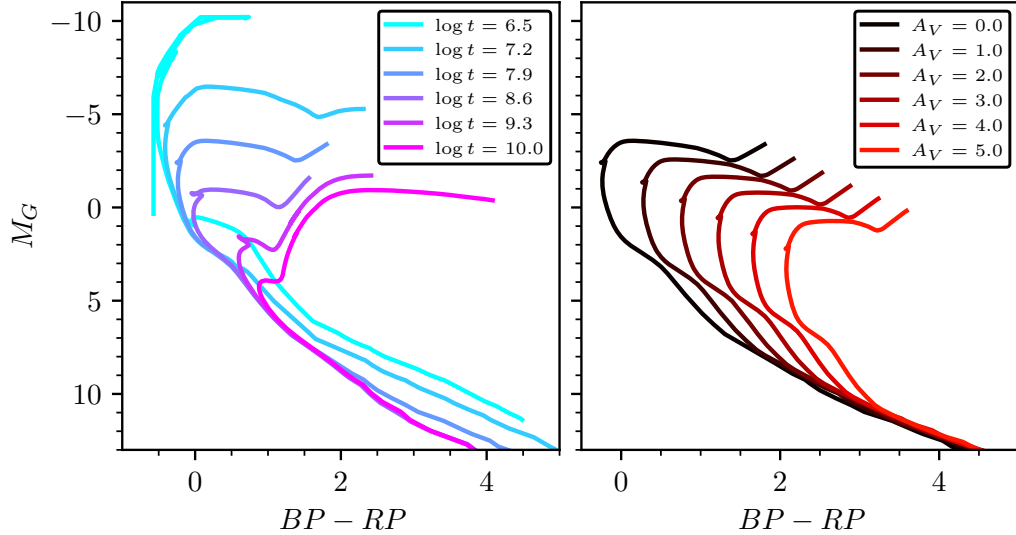
Fig. 1.11.: Comparison between stellar isochrones of various different parameters, derived from PARSEC stellar evolution models (Bressan et al. 2012) and shown in Gaia photometric bands. Left: isochrones of solar metallicity and zero extinction shown for six different ages. Most noticeably, as cluster age increases, the magnitude of the turn-off point decreases, with ever-more stars evolving into red giants and eventually reaching the end of their lives. The rest of the stars in the cluster also move down slightly, relaxing onto the main sequence as they age. Right: the \log t = 7.9 isochrone from the left plotted at a range of different extinction values. Extinction reddens cluster stars as well as reducing their overall brightness. Extinction in Gaia photometry has a strong effect on the location of the turn-off point.
