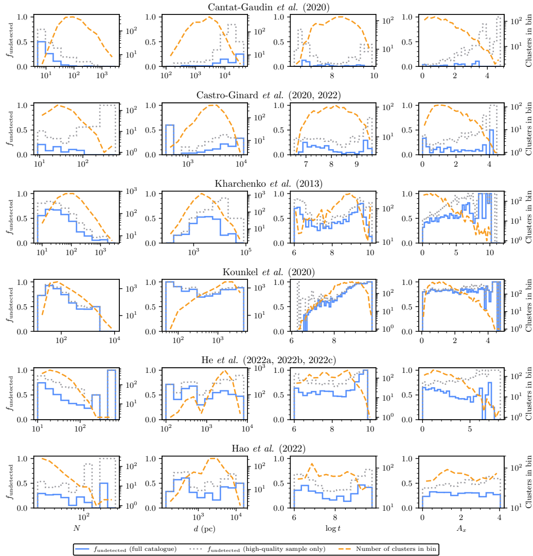
Fig. 3.15.: Plots showing the fraction of clusters undetected by this work when compared to various literature works or series of literature works, shown as a histogram of various parameters as a solid blue line for all clusters in the catalogue, and a dashed grey line for clusters in the high quality sample defined in Sect. 3.7.1. The dashed orange lines show the number of clusters in each bin. Optimum histogram bin widths were selected automatically using numpy (Harris et al. 2020). From left to right, each column shows the number of stars N , distance d , age \log t and extinction A_x reported in each catalogue. For the top four groups of catalogues, extinctions were given in the V band. For the lower two, extinctions were given in Gaia 's G band, which are generally slightly lower.
