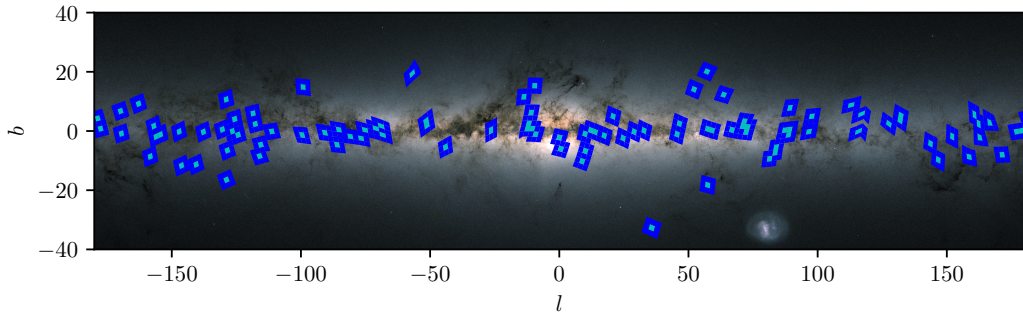
Fig. 2.1.: Target fields for this study plotted above a Gaia map of stellar density in an equirectangular projection. Cyan regions show the 100 main HEALPix level five pixels. Each main pixel was merged with its eight nearest neighbours, which are shown in blue. Some nearest neighbour pixels overlap between different fields.
