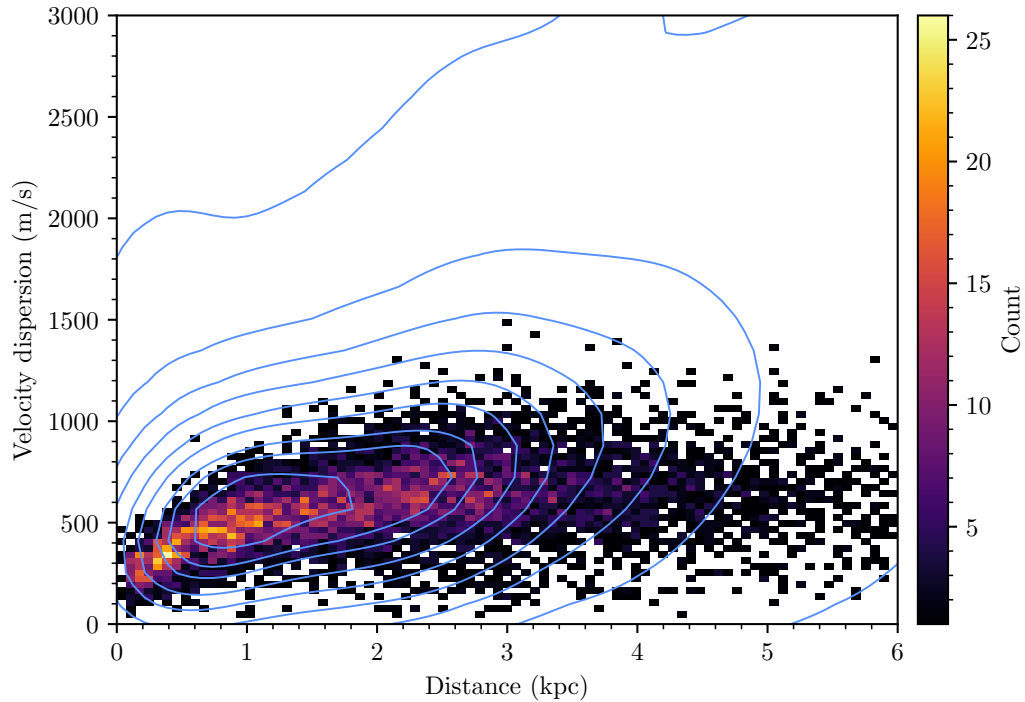
Fig. 4.11.: Simulated binary star velocity dispersion contaminations as a function of distance for all clusters in the sample. Cluster binary star contaminations are shown as a two-dimensional histogram, with bin shading giving the number of clusters in each bin. The measured velocity dispersion of all clusters is shown as a blue contour plot above this histogram.
