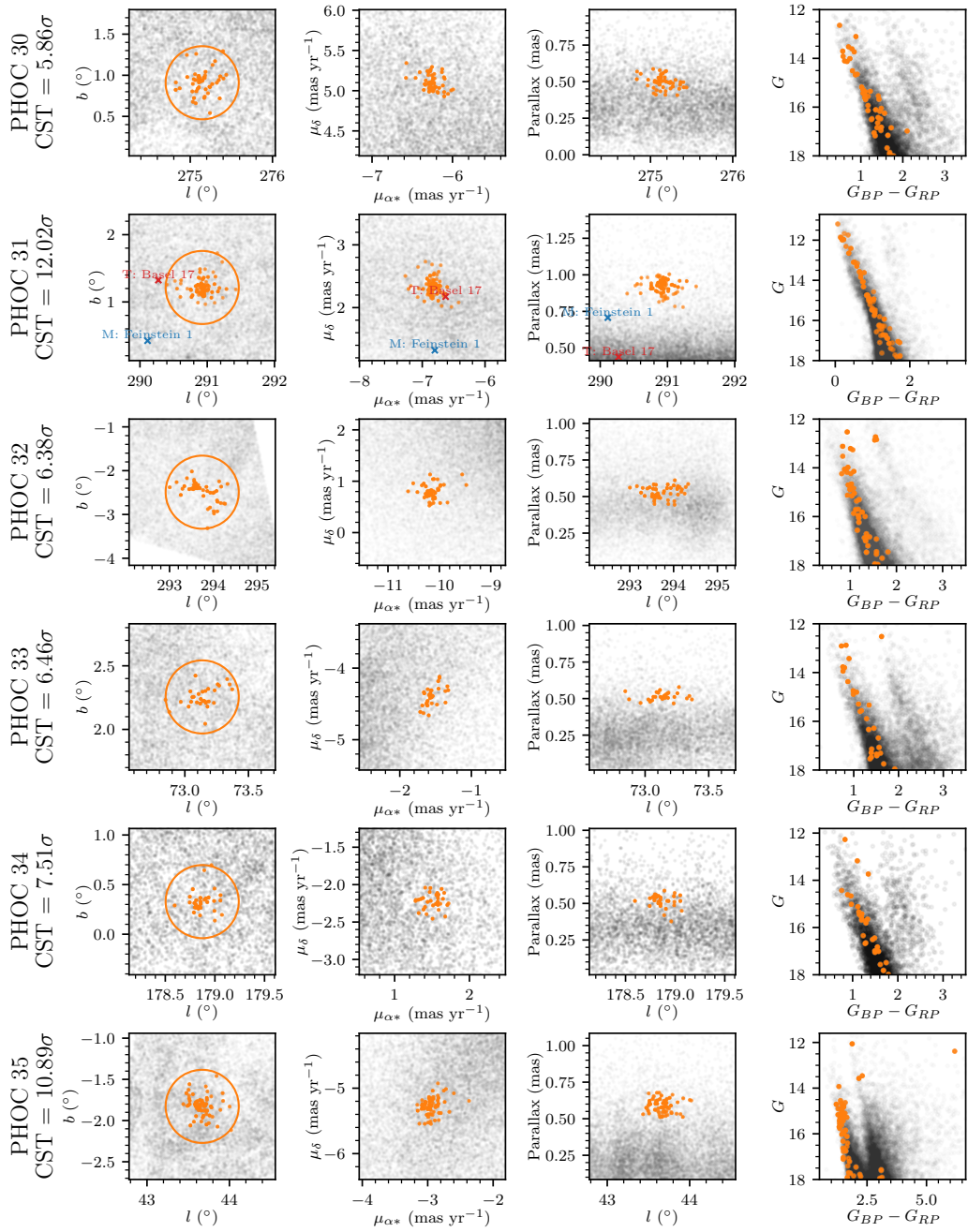
Fig. A.6.: Plots of the new OCs PHOC 30 to 35, plotted in the same style as Fig. A.1.
