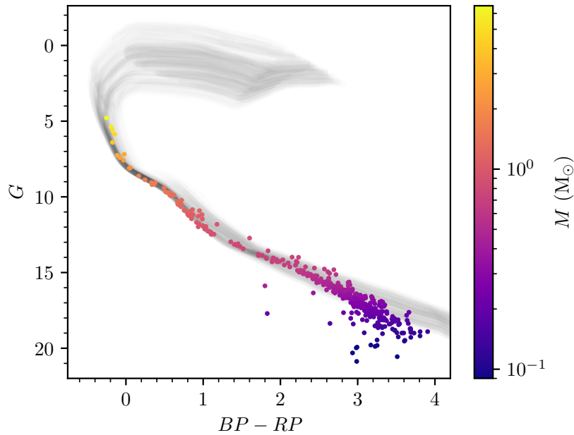
Fig. 4.1.: CMD of NGC 2451A with stars shaded by their median sampled stellar mass from interpolation against cluster isochrones. 100 isochrones sampled from the age-determination neural network in Paper 2 are plotted in black.
