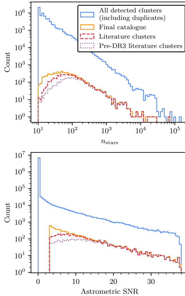
Fig. 3.2.: Statistics of all detected clusters compared against the final catalogue. Top: distribution of the number of member stars of detected clusters, n_{\text{stars}} , for all detected clusters in all fields before catalogue merging and duplicate removal (solid blue line), for the final catalogue (solid orange line), and amongst clusters in the final catalogue that crossmatch to clusters in the literature, for all literature clusters (solid red line) and for only those detected before the release of Gaia EDR3 (dotted purple line). Bottom: as above, but for the astrometric S/N (CST score) for all clusters in these sets. S/Ns have a maximum value of 38 due to numerical reasons.
