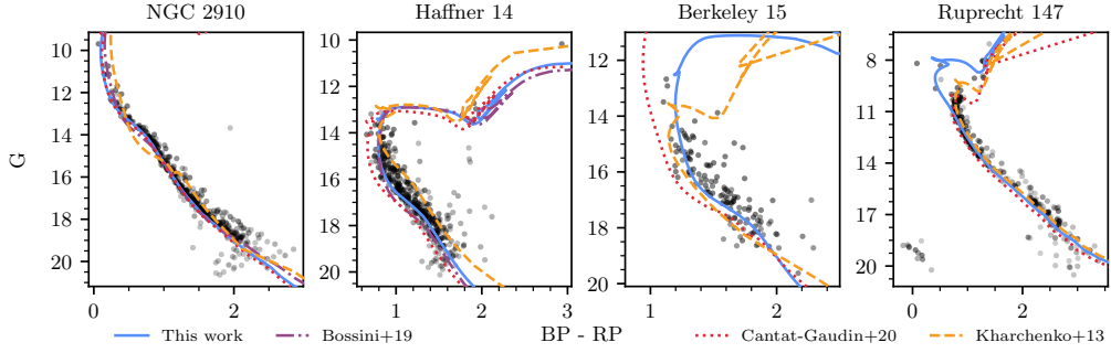
Fig. 3.7.: Predicted cluster isochrones from this work (solid blue line) compared with those from other works. Cluster members are plotted in black and shaded according to their membership probability.
