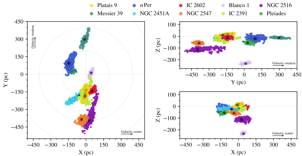
Fig. 1.9.: The detected tidal tails and comas of ten OCs near to the Sun. Clusters are shown as coloured density plots and plotted in heliocentric coordinates with the galactic centre to the right. Credit: Meingast et al. 2021
