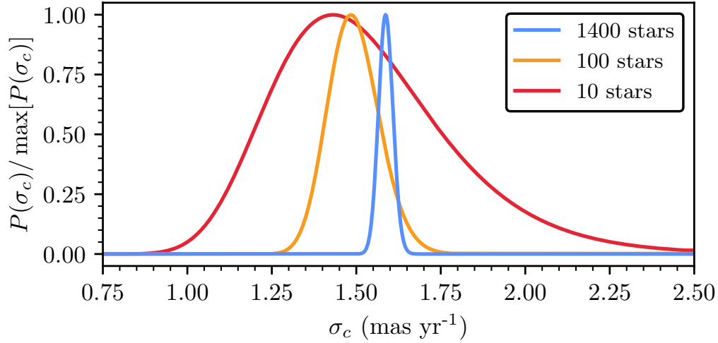
Fig. 4.6.: Proper motion dispersion likelihood in Eqn. 4.2 evaluated for different subsets of stars in Melotte 22 (the Pleiades). The blue curve shows all 1400 stars within my calculated value of r_J . The orange and red curves are for sets of 100 and 10 stars respectively that were randomly sampled from the overall cluster, showing how the likelihood becomes broader and asymmetric as uncertainty on the true value increases.
