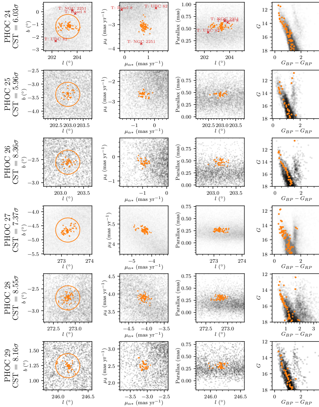
Fig. A.5.: Plots of the new OCs PHOC 24 to 29, plotted in the same style as Fig. A.1.
