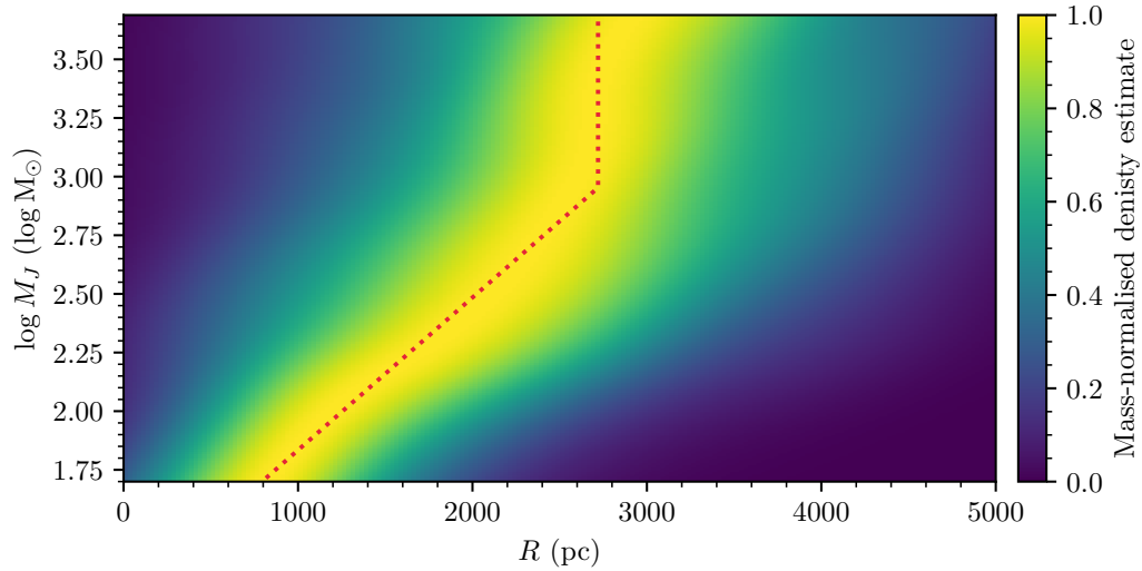
Fig. 4.15.: Mass-distance distribution of clusters shown as a kernel density estimate. At a given mass, the density estimate is normalised to have a peak of one, such that every horizontal strip of the diagram is effectively a normalised PDF of cluster distances at a given mass. The dotted red line shows the best fitting log-linear completeness model.
