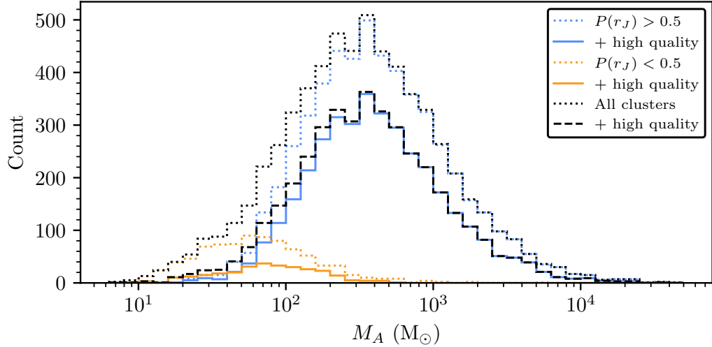
Fig. 4.9.: The distribution of total masses for all clusters with mass measurements and excluding globular clusters. Clusters are split into samples based on the probability that they have a valid Jacobi radius. In addition, solid lines show this for the ‘high quality’ sample of clusters from Paper 2 (those with an astrometric S/N greater than 5\sigma and a median CMD class greater than 0.5), while dashed lines include all clusters with mass measurements in this work.
