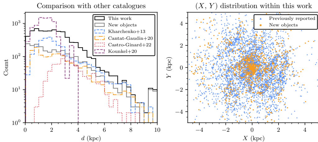
Fig. 3.9.: Distance and spatial distributions of clusters in this work. Left: the distance distribution of all clusters in this work that do not crossmatch to known GCs compared to other catalogues. Right: The distribution of clusters in this work in Cartesian coordinates centred on the Sun, cut to only those within 5 kpc in the X or Y directions. All previously reported clusters that we re-detect are shown as blue triangles, and all objects new in this work shown as orange circles.
