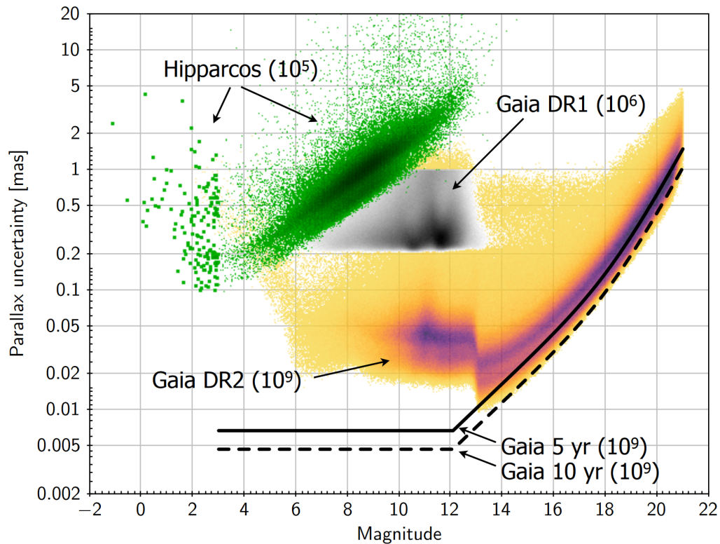
Fig. 1.5.: Comparison between the astrometric accuracy for all sources in the final data release of Hipparcos, Gaia DR1, and Gaia DR2. The predicted accuracy of future data releases using 5 and 10 years of data is shown by the solid and dashed lines respectively. Credit: Lindegren et al. 2018.
