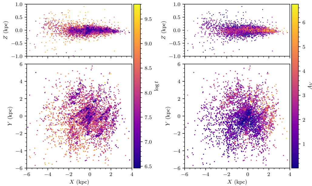
Fig. 3.10.: Spatial distributions of clusters detected in this work shaded on our derived \log t and A_V values. Left: side-on and top-down distribution of clusters in heliocentric coordinates that do not crossmatch to known GCs. The galactic centre is to the right, with the Sun at (0, 0) . Only clusters passing two quality cuts are plotted: firstly, those with a CST score above 5\sigma , meaning they are highly probable astrometric overdensities; and secondly, a median CMD class above 0.5, which are those compatible with single population star clusters. Clusters are plotted in descending age order, meaning points representing young clusters are most visible in crowded regions. Right: as left, except clusters are colour-coded by extinction A_V . Clusters are plotted in ascending order of extinction.
