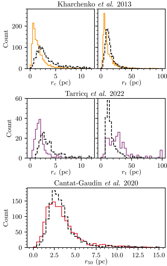
Fig. 3.12.: Cluster radii derived in this work (dashed black line) compared against the distributions of cluster radii in various literature works. Top row: r_c (top left) and r_t (top right) of 1446 clusters from Kharchenko et al. 2013 that we redetect in this work (solid orange curve) compared against our approximately estimated King 1962 radii for these 1446 clusters. Middle row: same as top, except for radii of 202 clusters from Tarricq et al. 2022 that have derived King radii (solid purple curve). Bottom: r_{50} measurements from Cantat-Gaudin and Anders 2020 compared against our r_{50} measurements for the 1343 clusters from their work that we redetect.
