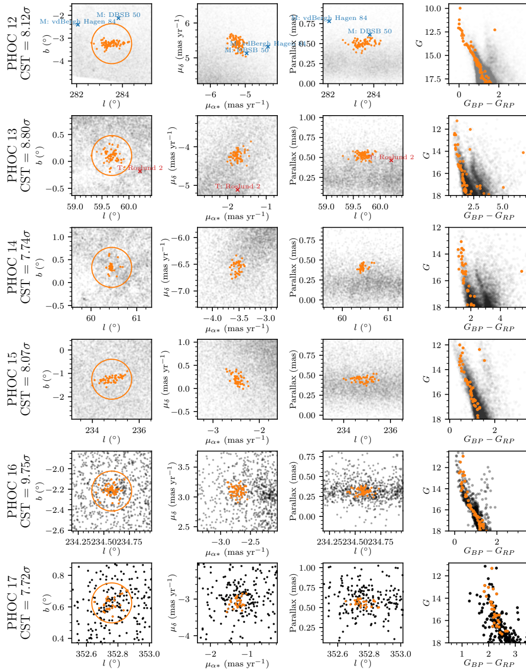
Fig. A.3.: Plots of the new OCs PHOC 12 to 17, plotted in the same style as Fig. A.1.
