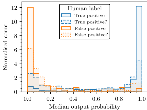
Fig. 3.3.: Performance of the CMD classifier on the independent test dataset of 2000 clusters detected by HDBSCAN in Gaia data and labelled by hand. Clusters are labelled as true positives or false positives, with clusters where the human classifier was less certain being additionally flagged.
