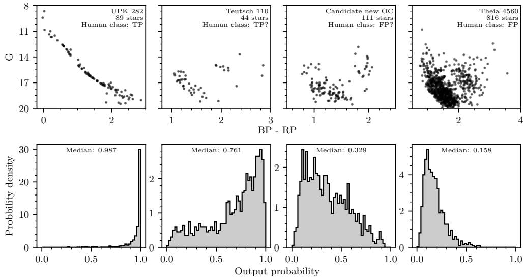
Fig. 3.4.: Four examples of classified cluster CMDs from the test dataset, with cluster CMDs on the top row and their PDFs of predicted probabilities on the bottom row. Cluster names and human-assigned labels are indicated on the figures. PDFs are generated by sampling the CMD classifier 1000 times for every cluster.
