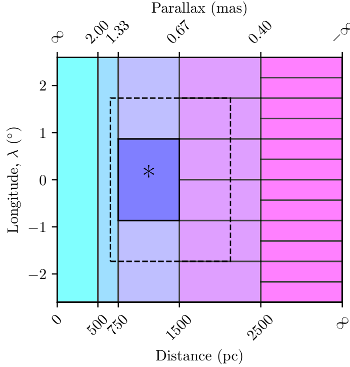
Fig. 2.4.: Schematic, top-down representation of the GMM partitioning system. Each box represents a column of sub-partitions viewed from the top. For the highlighted sub-partition also marked with an asterisk (*), the dashed width of the box shows the region in which extra stars with a parallax uncertainty of greater than 1 mas would be included. The height of the dashed box shows the extra overlap between this sub-partition and nearby other sub-partitions. Any cluster with a centroid within the dashed region but not within the main highlighted region was automatically discarded, as it will be better characterised by the neighbouring sub-partition its centroid is in.
