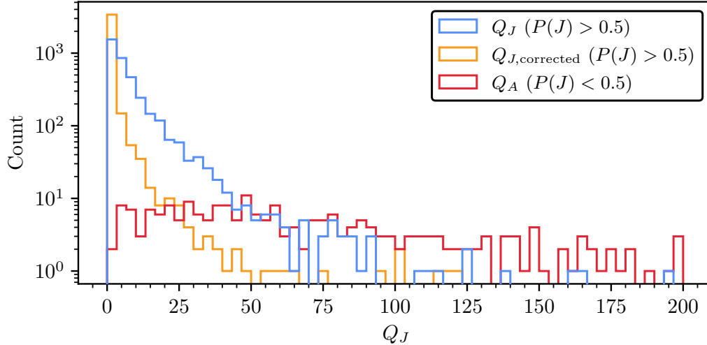
Fig. 4.12.: Distribution of cluster virial ratios. The blue histogram shows virial ratios for clusters with a valid Jacobi radius, the orange histogram shows virial ratios for the same clusters with an approximate correction for binarity applied, and the red histogram shows the virial ratio of the entire cluster for clusters without a valid Jacobi radius.
