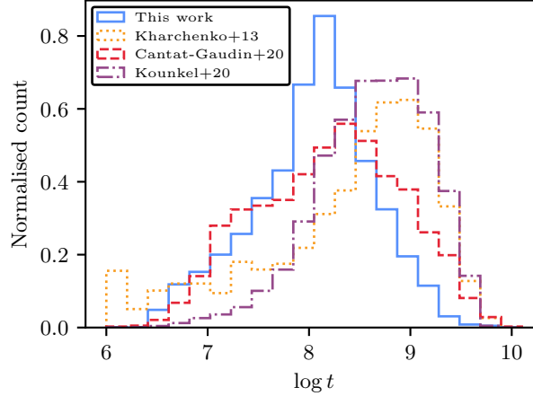
Fig. 3.11.: Histogram of ages of all clusters in this work with median CMD classes greater than 0.5 – specifically, all clusters with photometry that is compatible with a single population of stars. These are compared to the ages of all clusters in the catalogues of Kharchenko et al. 2013, Kounkel et al. 2020, and Cantat-Gaudin et al. 2020. Known GCs are excluded from the results of this work and the results of previous works for this plot.
