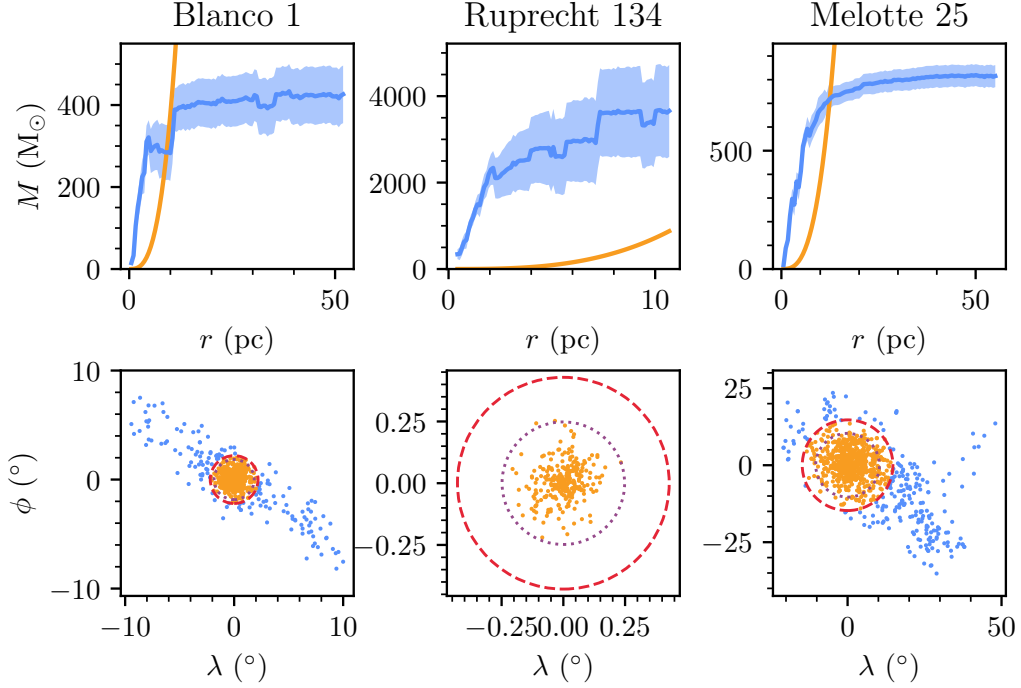
Fig. 4.4.: Jacobi radius determination for three OCs: Blanco 1, Ruprecht 134, and Melotte 25 (the Hyades). Each of the three columns corresponds to each cluster. Top row: the estimated total mass contained within a radius r is shown in blue ( M_{\text{obs}}(r) ), with the 1\sigma error region shaded on the plot. The orange line shows the theoretical amount of mass contained within a radius r according to the Jacobi radius equation ( M_J(r) , Eqn. 1.3). The intersection of these two lines corresponds to the cluster's r_J . Bottom row: the distribution of cluster member stars. To remove spherical distortions, positions are rotated to an arbitrary coordinate frame with longitude \lambda and latitude \phi centred on the cluster centre. Stars within r_J are shown in orange while stars outside r_J are shown in blue. The dashed red line shows r_J , while the dashed purple line corresponds to the approximate value of r_t determined in Paper 2.
