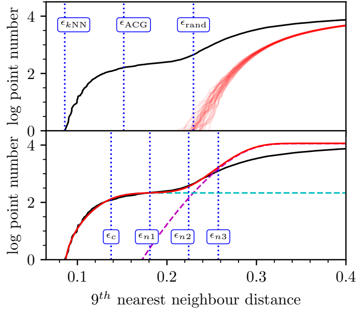
Fig. 2.2.: Nearest neighbour graphs for both methods of determining the optimum \epsilon for DBSCAN. To produce this plot, which is effectively an unnormalised log cumulative density function (CDF) of nearest neighbour distances, stars are sorted based on their k^{\text{th}} NN distances and numbered from one to n . These labels as a function of k^{\text{th}} NN distance are then plotted to form a continuous curve. The black line on both plots is the 9^{\text{th}} NN distances of a 2.5^\circ field around the nearby OC Blanco 1. On the upper plot, \epsilon estimates are determined by re-sampling the field 30 times (shown in red) to smooth out the signature of clustered stars. On the lower plot, a model of the signature of the cluster (cyan, dashed) and the field (magenta, dashed) is summed (red, solid) to approximate the curve and produce four \epsilon estimates.
