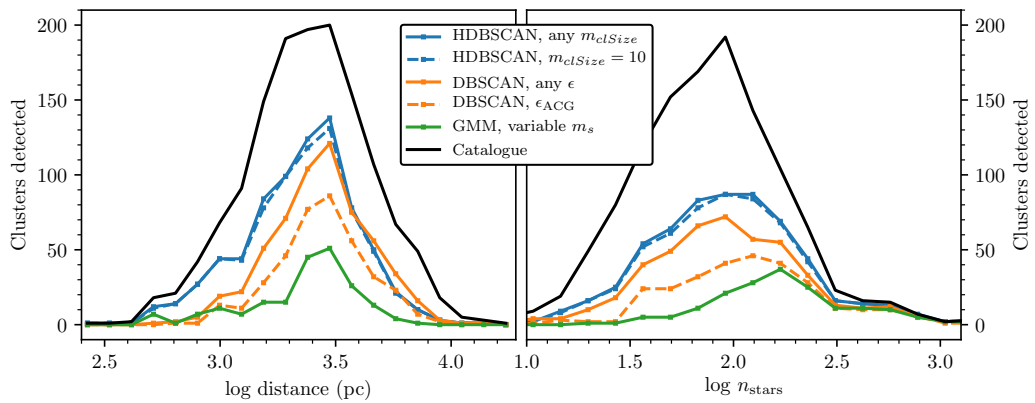
Fig. 2.6.: Distance and size dependence of detections by different algorithm and parameter combinations for all 1385 OCs in all studied fields, plotted against the reported size and distance of the OCs in the literature. OC candidates not passing the criterion in Sect. 2.4.2 and with a CST of less than 3\sigma were discarded. HDBSCAN detects the most OCs, especially at nearby distances. GMMs only perform well at detecting well populated OCs. While individual DBSCAN results at different \epsilon values do not detect especially many OCs, combining them all together nearly matches the performance of HDBSCAN – even exceeding it slightly at large distances.
