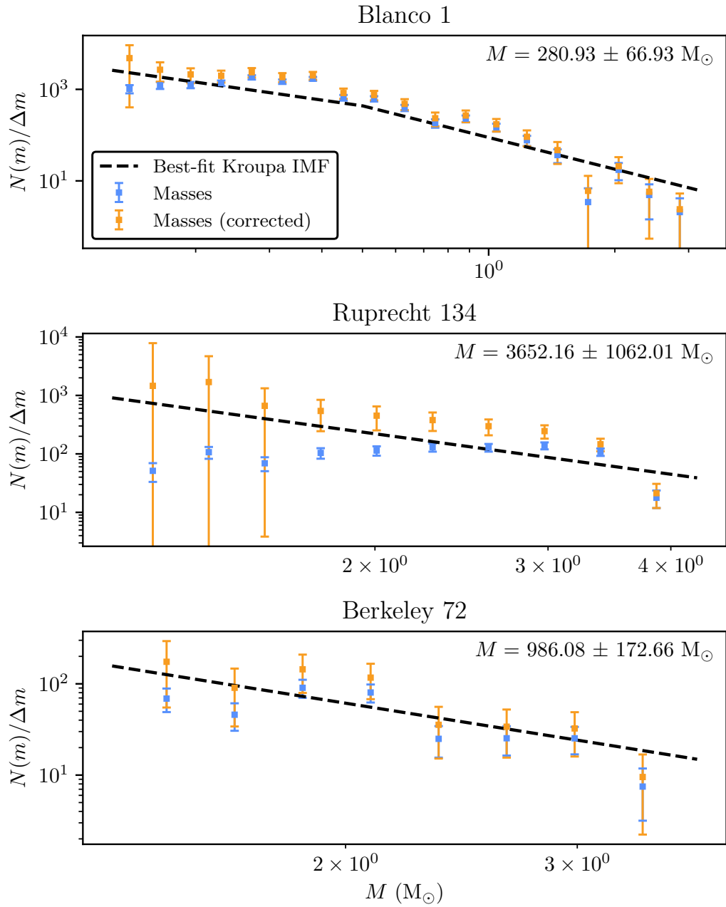
Fig. 4.3.: Mass function fits to the three OCs from Fig. 4.2. The blue points show measured binned stellar masses, the orange points show these masses after correcting for selection effects and modest assumptions about binary stars, and the black dashed line shows the best-fitting Kroupa IMF. The integral of the cluster mass function is written in the top right of each plot.
