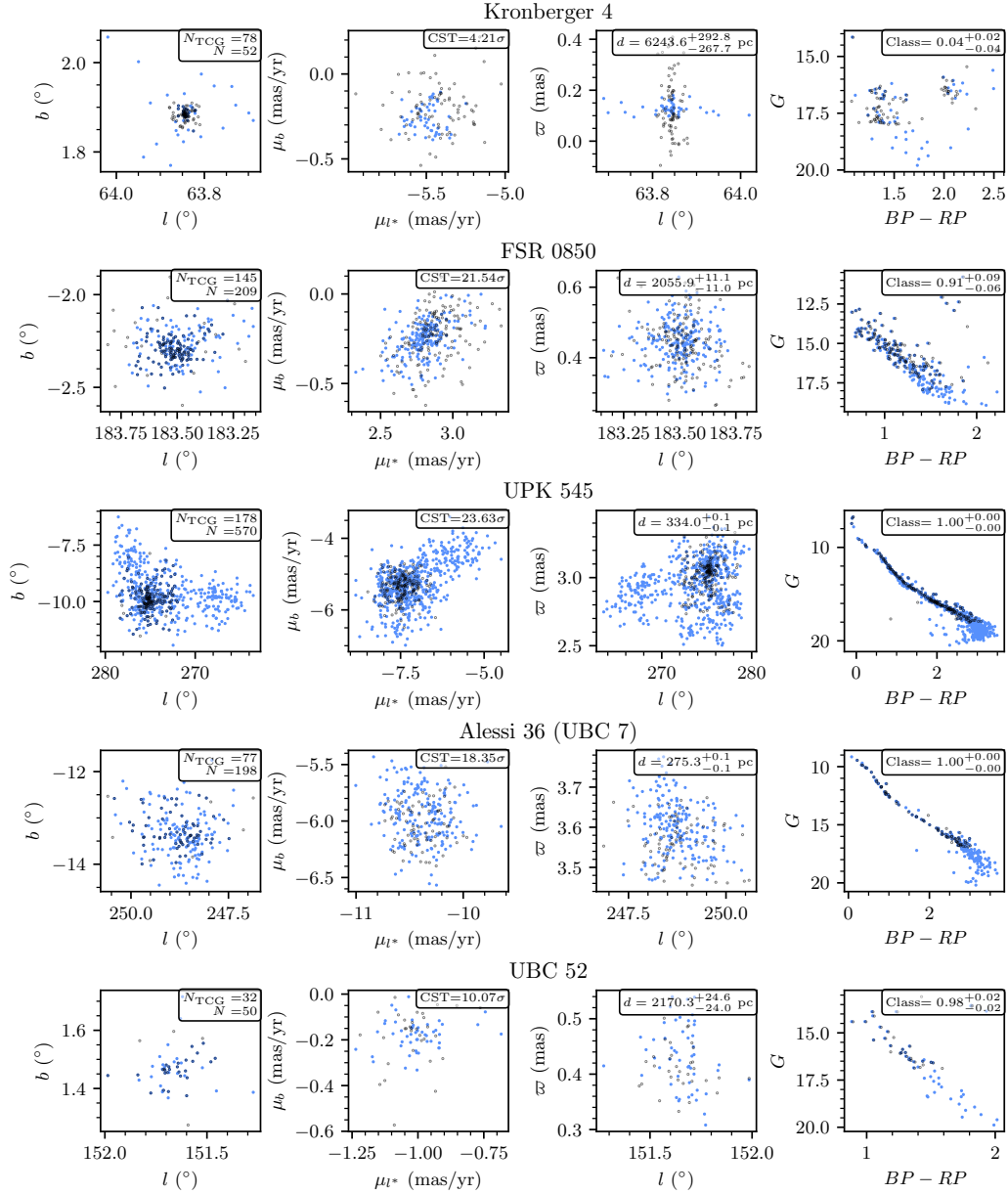
Fig. 3.13.: Membership list comparisons between this work and the catalogue of Cantat-Gaudin and Anders 2020, using three clusters selected at random (upper three) and two clusters selected at random that were detected in Castro-Ginard et al. 2018 using Gaia DR1 data. Stars assigned as members by this work are plotted with filled blue circles, while members reported by Cantat-Gaudin and Anders 2020 are plotted with empty black circles. The first three columns compare the astrometry of cluster members in galactic coordinates, proper motions, and parallax as a function of l . The final column compares colour-magnitude diagrams of each resulting membership list. For every cluster, various parameters are labelled on the plots: number of member stars in Cantat-Gaudin and Anders 2020 N_{\text{TCC}} , number of member stars in this work N , astrometric S/N as estimated by the CST, distance d , and probability of being a single stellar population given the neural network in Sect. 3.4.
