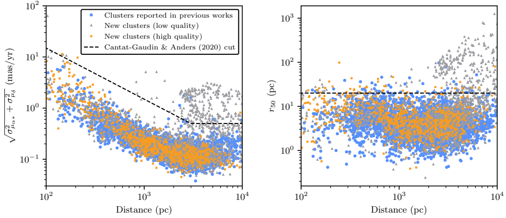
Fig. 3.16.: Geometric mean of the proper motion dispersion (left) and radius containing 50% of members (right) for the clusters reported in this work, as a function of distance. Clusters are split between those detected in previous works (blue circles) and those newly reported in this work, divided between the high quality (orange squares) and low quality (grey triangles) samples defined in Sect. 3.7.1. The cuts on cluster parameters to distinguish between bound OCs and unbound moving groups or associations proposed in Cantat-Gaudin and Anders 2020 are shown as a dashed black line.
