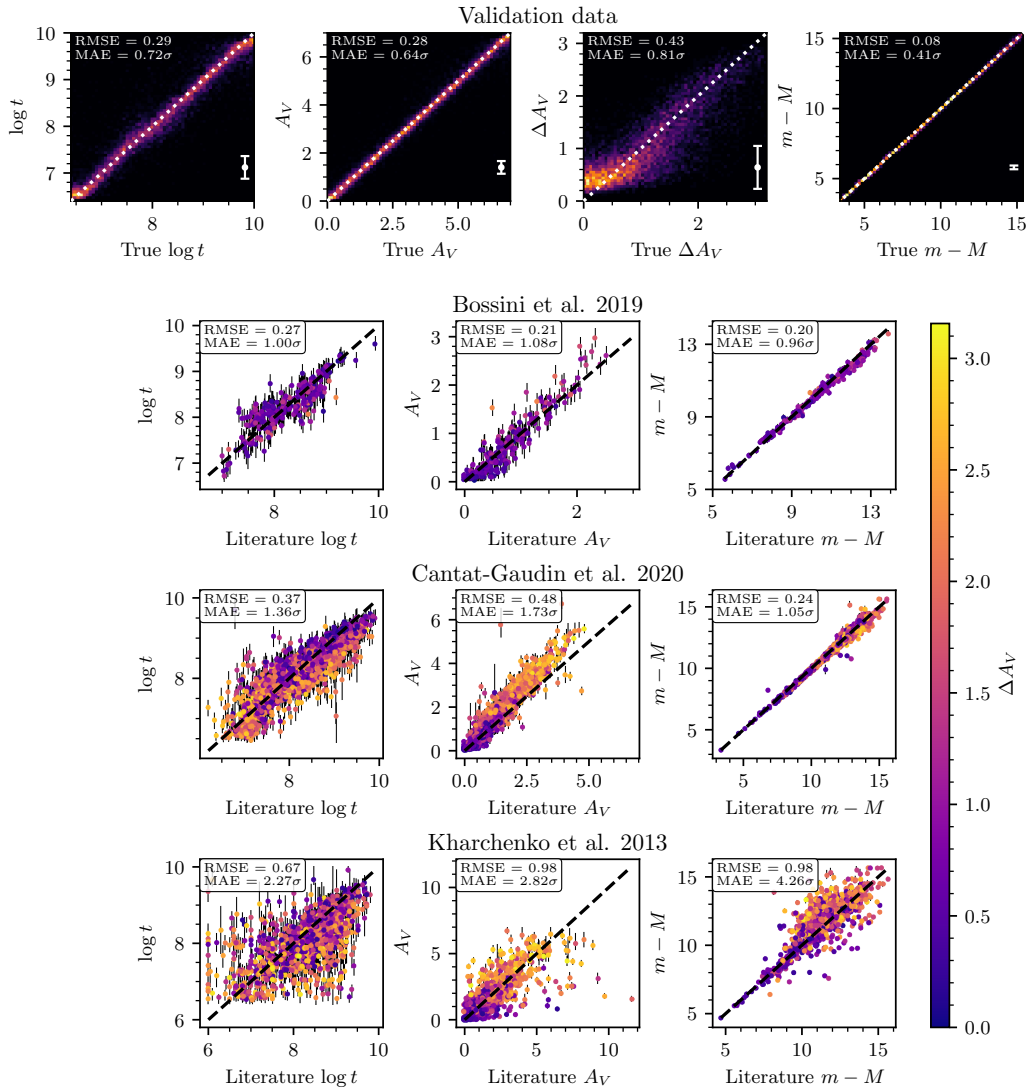
Fig. 3.5.: Photometric parameters derived in this work compared against test datasets. Top row: 2D histograms showing the performance of the trained photometric parameter inference network on all 10 000 clusters from the validation dataset. The mean output uncertainty is shown with white error bars. As indicated by the dashed lines, predicted values on the y axis should be equal to true values on the x axis. The root mean square error (RMSE) and mean absolute error in terms of output network uncertainty (MAE) are given in the top left. All plots and the RMSE are in units of magnitude other than on age plots which are logarithms of cluster age in years. Other rows: comparison between network predicted parameters and ages, extinctions, and distance moduli for 247, 1753, and 1206 clusters in common with the catalogues of Bossini et al. 2019, Cantat-Gaudin et al. 2020, and Kharchenko et al. 2013 respectively. Points are shaded based on the differential extinction we infer for each cluster.
