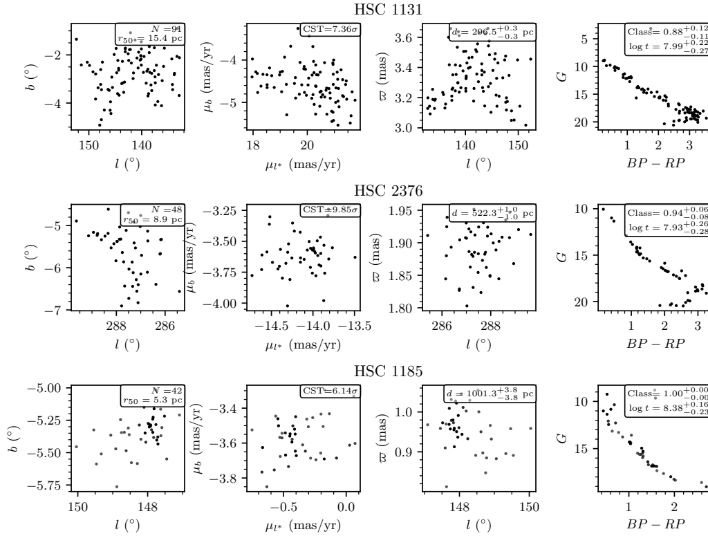
Fig. 3.17.: Three newly reported clusters randomly selected from the cluster catalogue and ordered by increasing distance, with member stars plotted as a function of their astrometric and photometric data as in Fig. 3.13. All clusters pass the cuts proposed in Cantat-Gaudin and Anders 2020, have good-quality CMDs passing the cuts from Sect. 3.4, and have astrometric significances of greater than 5\sigma , meaning they are almost certainly real overdensities in Gaia data.
