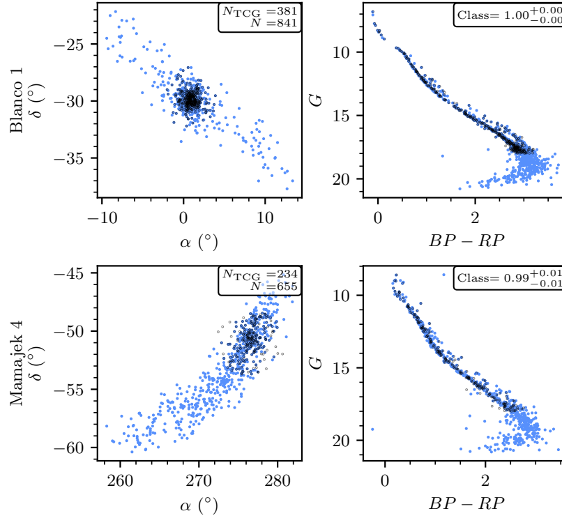
Fig. 3.14.: Two examples of clusters in the catalogue that have detected tidal structures. The spatial distribution of the clusters Blanco 1 (top row) and Mamajek 4 (bottom row) are plotted on the left, with member stars reported in this work shown as filled blue circles and compared against member stars from Cantat-Gaudin and Anders 2020 which are plotted as empty black circles. CMDs are shown in the two plots on the right for both clusters.
