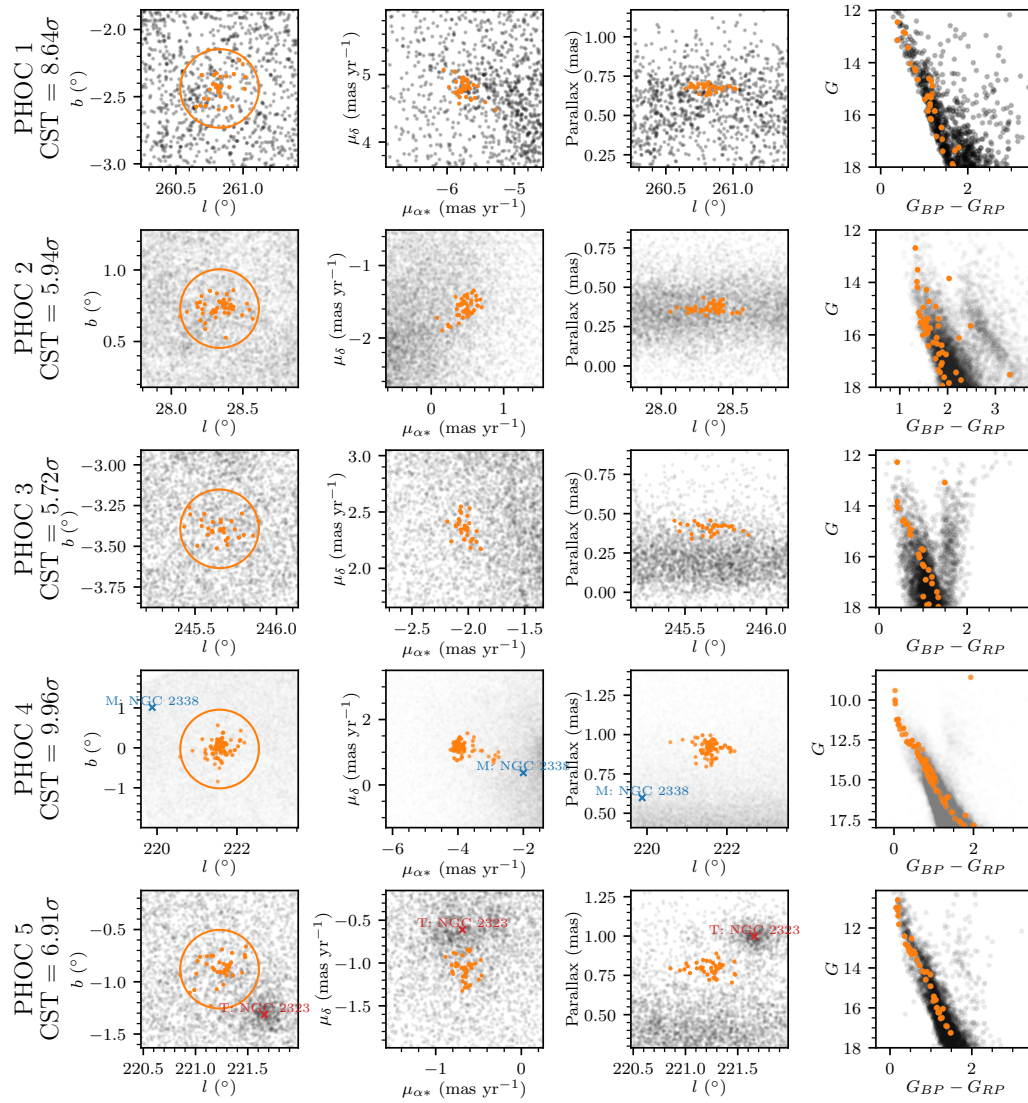
Fig. A.1.: Astrometric and photometric plots of the first five new OCs from Sect. 2.6. Identified member stars are shown in orange, with background stars in black. Only members with a membership probability of greater than 50% are plotted. The estimated tidal radius for the OCs is depicted with a circle in the l vs. b plots in the first column. CST scores for each object are shown with its name on the left. Nearby OCs from literature catalogues are marked when visible. T (in red text) denotes sources from Cantat-Gaudin and Anders 2020, while M (blue) and S (purple) denote sources from MWSC and Sim et al. 2019 respectively that were not detected by Cantat-Gaudin and Anders 2020. A (brown) denotes new OCs detected recently by Castro-Ginard et al. 2020.
