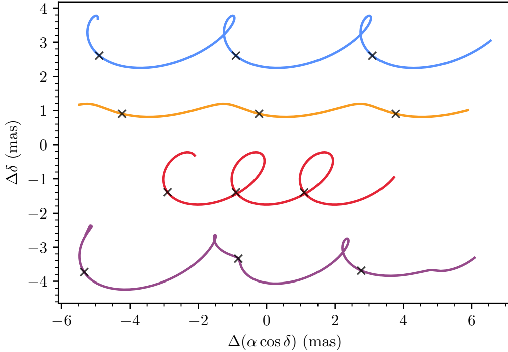
Fig. 1.6.: The predicted on-sky astrometric tracks of stars with different parameters, generated using astromet (Penoyre et al. 2022a). All sources are at coordinates \alpha, \beta = (0^\circ, 45^\circ) , but are offset in the y direction for clarity of plotting. The first source has \mu_{\alpha^*} = 4 \text{ mas yr}^{-1} , \mu_\delta = 0 , and is at a distance of 1 kpc. In the second example, the distance is quadrupled relative to the first. In the third example, the proper motion is halved relative to the first. In the final example, a binary with a period close to 1 yr, high eccentricity, and a low light ratio is added to the first example, producing a highly irregular track. The crosses denote the position of each source in one-year intervals.
