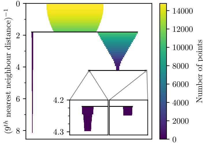
Fig. 2.3.: Condensed tree graph for HDBSCAN with m_{clSize} = 80 applied to a 2.5^\circ field around Blanco 1, a nearby cluster without any other known OCs in the field. The colour and width of each icicle denotes the number of stars remaining in the cluster. Horizontal splits occur when clusters are no longer connected. The long icicle on the left is Blanco 1, which is an extremely clear, nearby cluster and hence splits early from field stars. On the right, the algorithm continues discarding field stars, splitting into two very short icicles at the end which are false positive clusters. The two small sub-plots in the lower right are zoomed in on the two small icicles.
