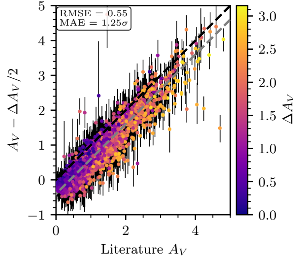
Fig. 3.6.: Extinction values from Cantat-Gaudin et al. 2020 compared against this work when corrected for differential extinction with an estimate of cluster differential extinction, plotted in the same style as Fig. 3.5. The dashed black line shows where y values equal x ones; the dashed grey line shows the same but offset by -0.4.
