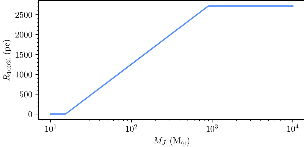
Fig. 4.16.: Simple log-linear model for the approximate 100% completeness limit ( R_{100\%} ) of the cluster census as a function of mass.
