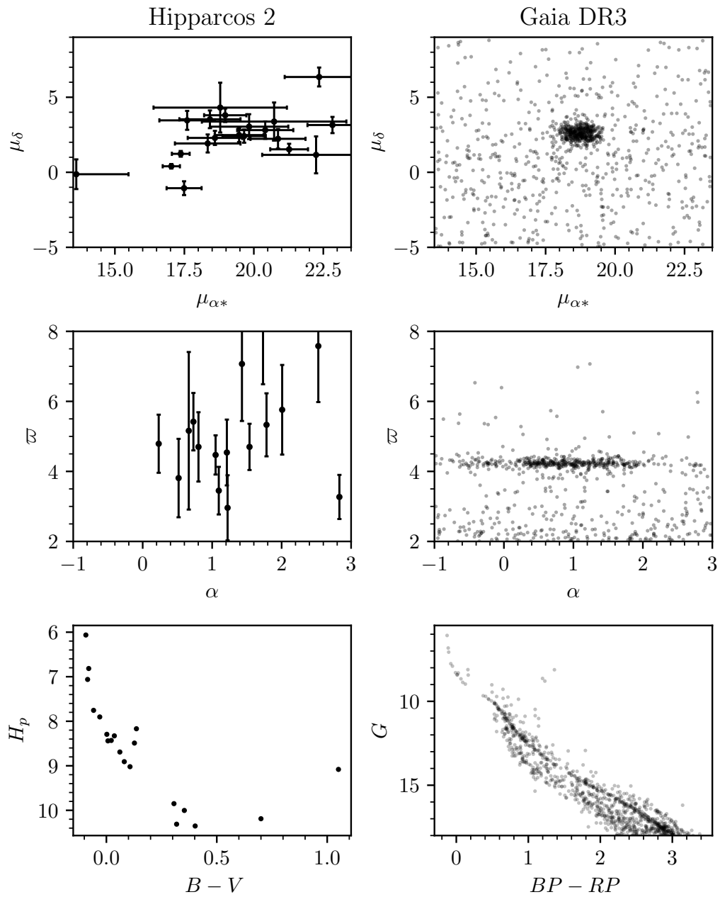
Fig. 1.7.: Comparison between the regions around the star cluster Blanco 1 in data from Hipparcos and Gaia . Hipparcos -2 data (van Leeuwen 2007) is shown on the left and Gaia DR3 data (Gaia Collaboration et al. 2022) is shown on the right. The top row shows proper motions, the middle row shows parallax as a function of right ascension, and the bottom row shows the CMD of the stars in each region. While Hipparcos only sees a few dozen bright stars for the cluster, Gaia can detect up to 1000, and to a significantly higher degree of astrometric accuracy.
