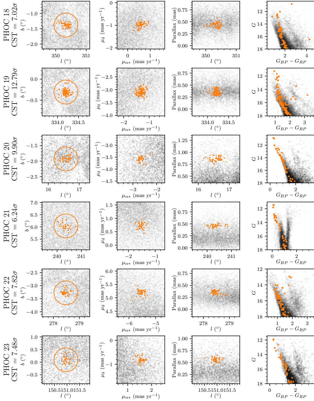
Fig. A.4.: Plots of the new OCs PHOC 18 to 23, plotted in the same style as Fig. A.1.
