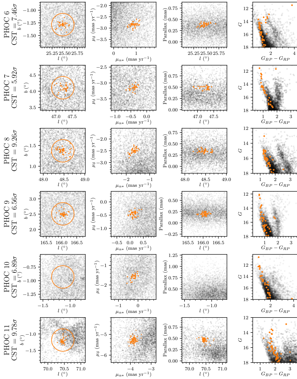
Fig. A.2.: Plots of the new OCs PHOC 6 to 11, plotted in the same style as Fig. A.1.
