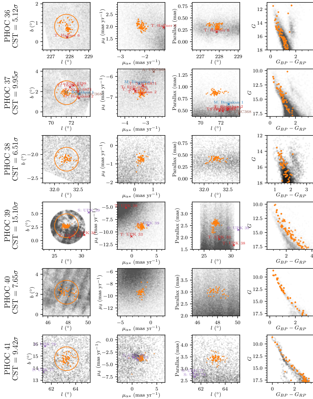
Fig. A.7.: Plots of the new OCs PHOC 36 to 41, plotted in the same style as Fig. A.1.
