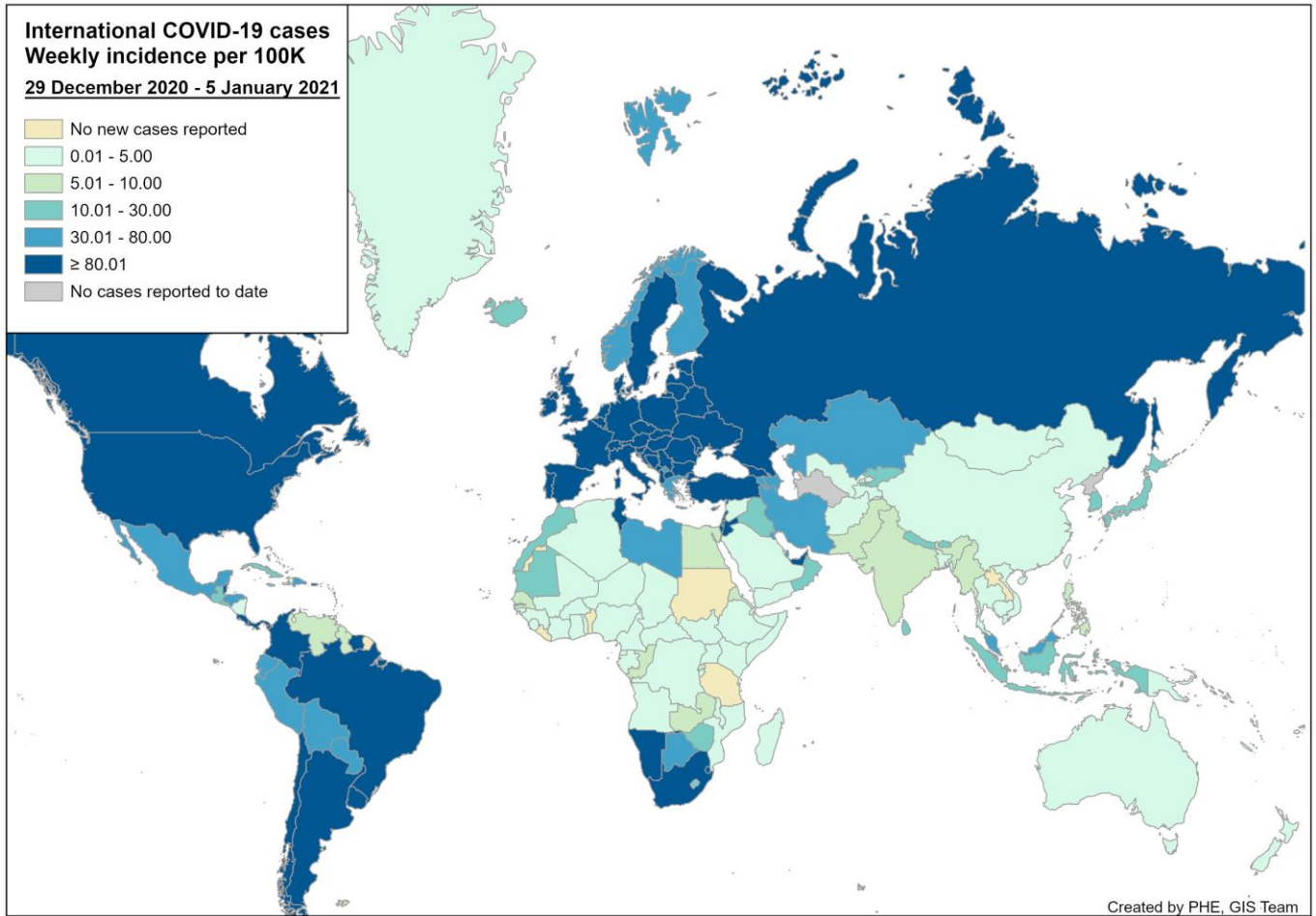
Figure 56: Global map of weekly COVID-19 case incidence rate per 100,000, week 53 2020
