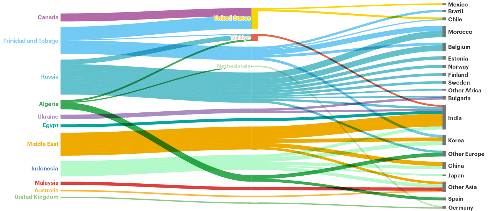
Figure 5.21 International ammonia trade flows via shipping, 2019
