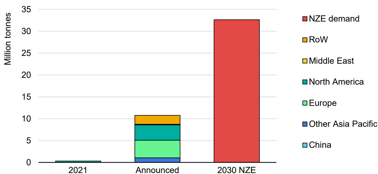
Figure 4.14 Capacity of hydrogen production from natural gas with CCS by country/region according to announced projects and in the NZE Scenario
