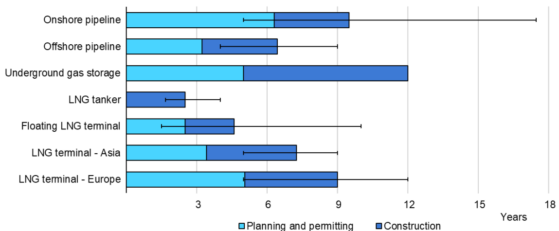
Figure 5.26 Lead times of selected natural gas infrastructure projects
