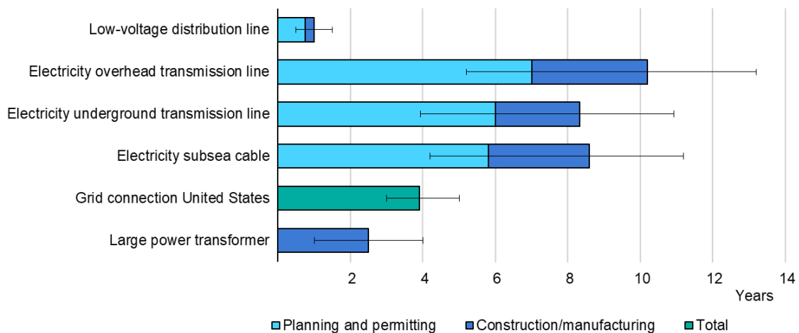
Figure 5.11 Average lead times to build new electricity grid assets in Europe and the United States, 2010-2021
