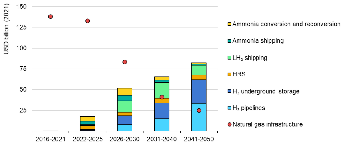
Figure 5.15 Average annual global investment in hydrogen and natural gas infrastructure in the NZE Scenario
