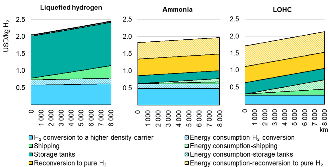
Figure 5.23 Indicative levelised cost of delivering hydrogen, by shipping-option step and distance in the NZE Scenario, 2030
