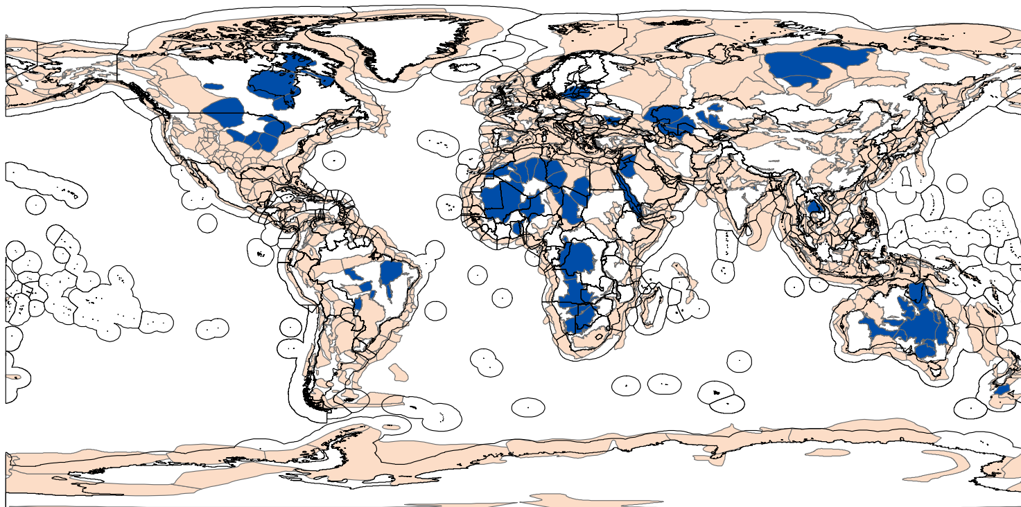
Figure A.33: Intracratonic Sag Basins
