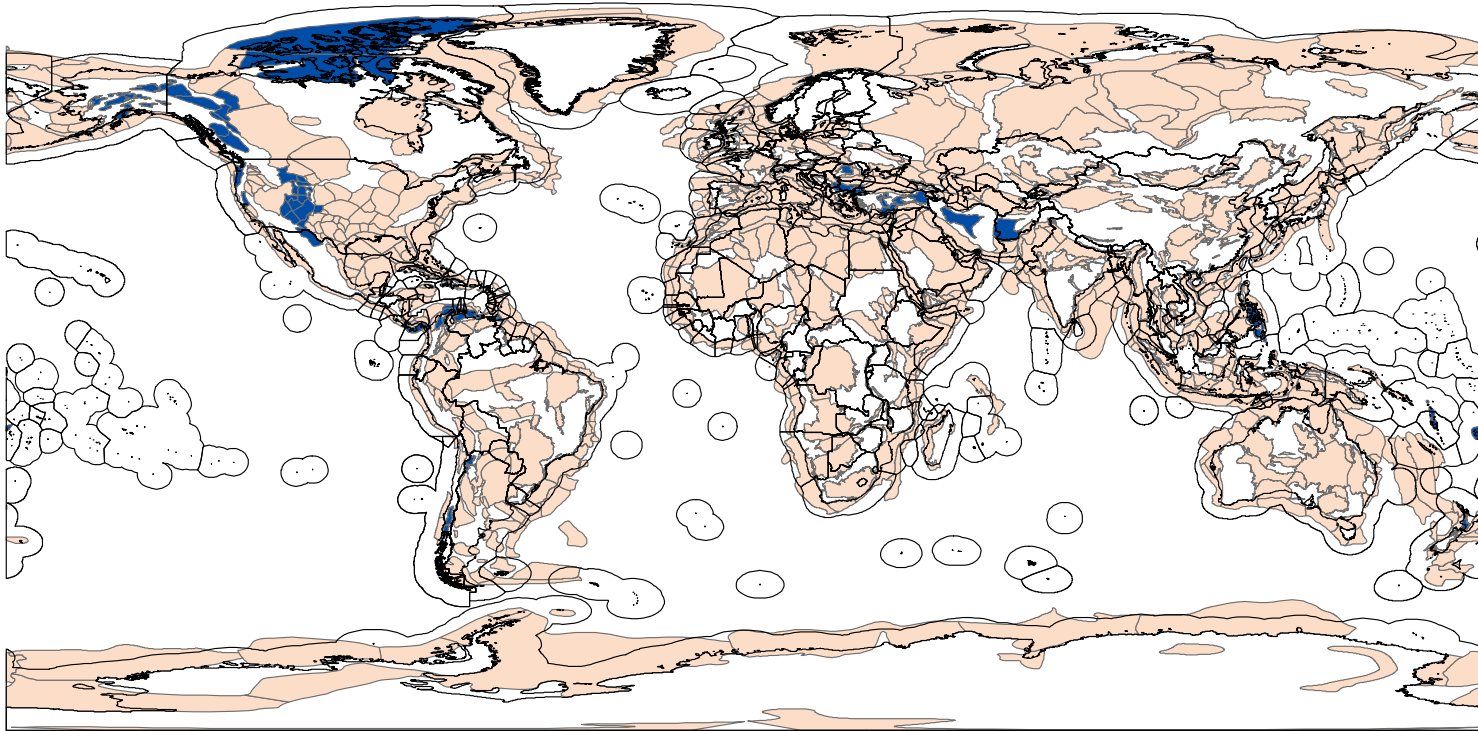
Figure A.31: Convergent Wrench Basins
