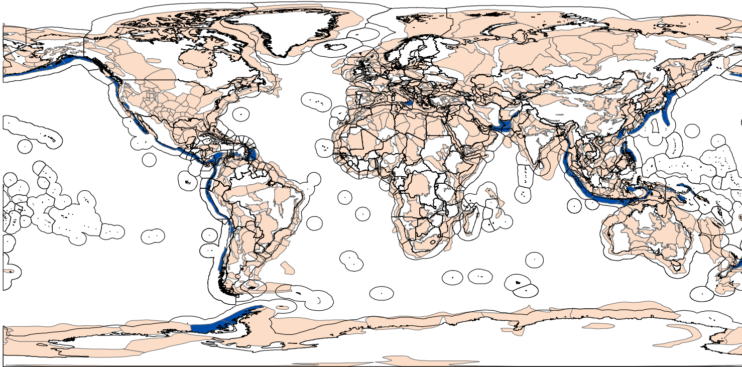
Figure A.28: Fore-Arc Basins
