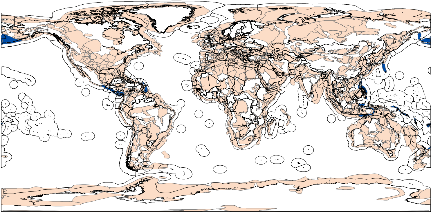
Figure A.23: Basins: Convergent Ocean-Ocean Tectonics
