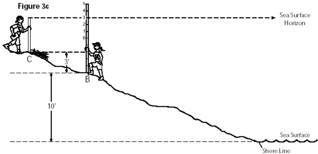
Figures 3a,b,c. A practical, short-cut method for measuring run-up. See text for detailed discussions.
