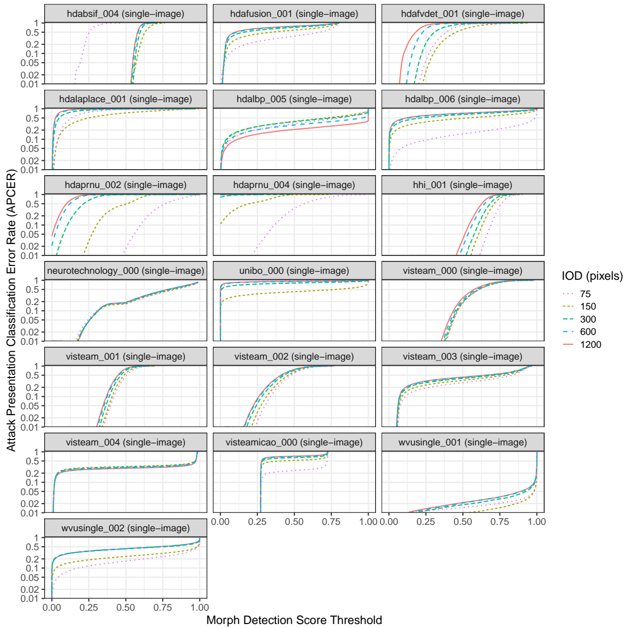
Figure 19: The curves show APCER (or morph miss rate) as a function of morph detection score threshold for different image resolutions, reported as interocular distance (IOD), the distance between the eyes. For individual algorithm results that are filterable and interactive, please refer to the algorithm report cards that are linked from the accuracy summary table on the FATE MORPH webpage .
