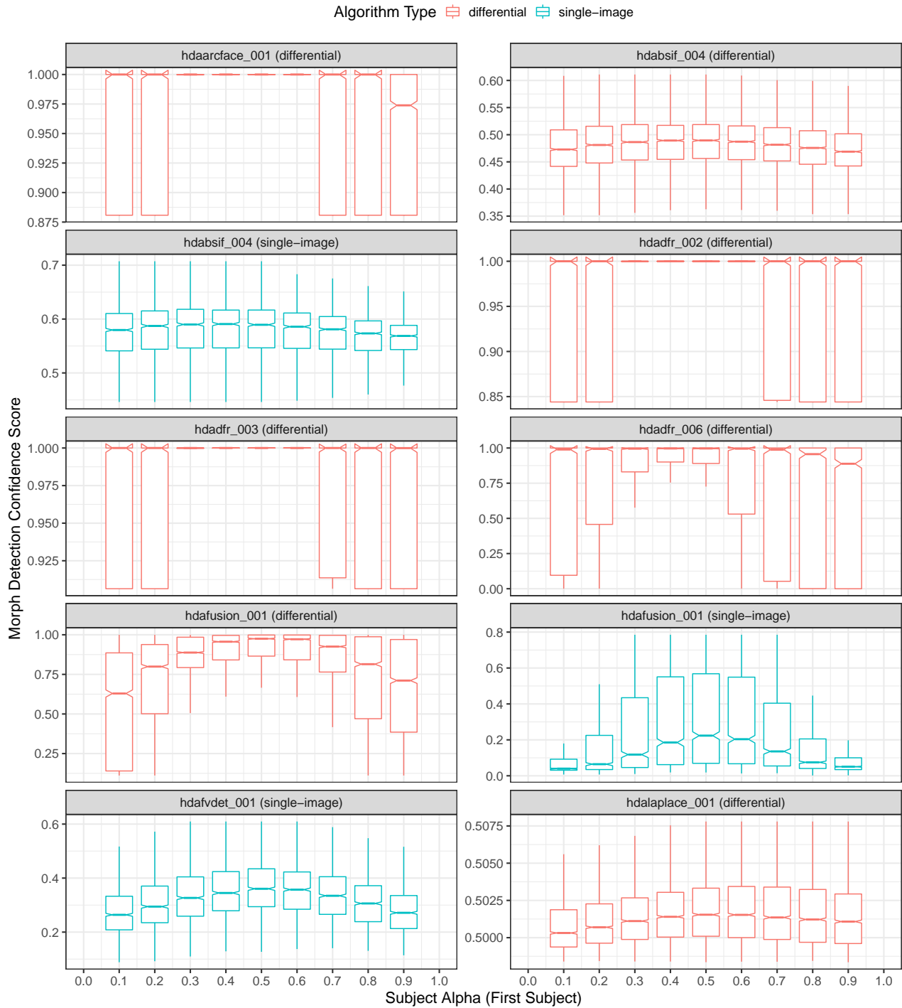
Figure 35: Boxplots plotting morph detection confidence score as a function of subject alpha (first subject in morph). Each plot includes scores that were successfully generated by the algorithm (i.e., results from failure to process were not used in this analysis). For individual algorithm results that are filterable and interactive, please refer to the algorithm report cards that are linked from the accuracy summary table on the FATE MORPH webpage .
