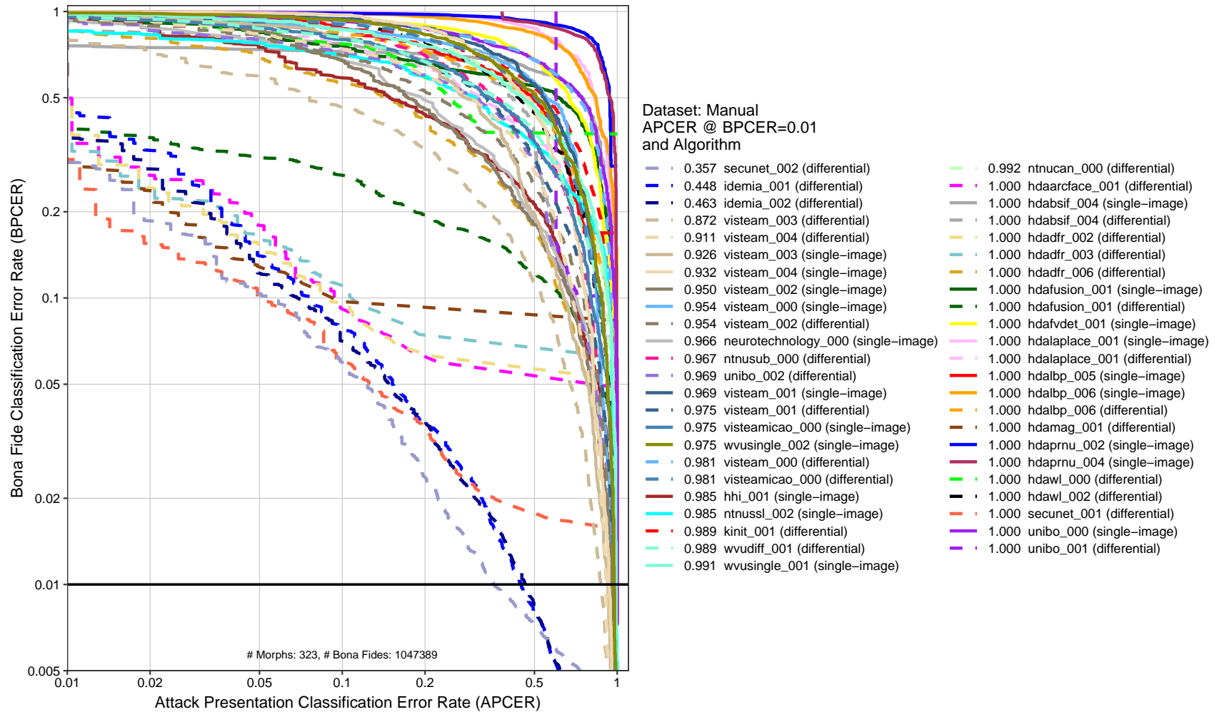
Figure 15: DET plot. This chart plots BPCER as a function of APCER. The x-axis is the rate morphs are not detected and the y-axis is the rate that bona fide images are falsely classified as morphs. The horizontal black line represents BPCER=0.01.
