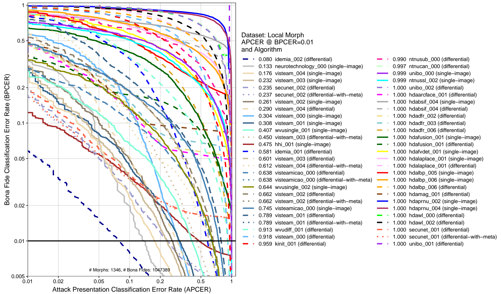
Figure 6: DET plot. This chart plots BPCER as a function of APCER. The x-axis is the rate morphs are not detected and the y-axis is the rate that bona fide images are falsely classified as morphs. The horizontal black line represents BPCER=0.01.
