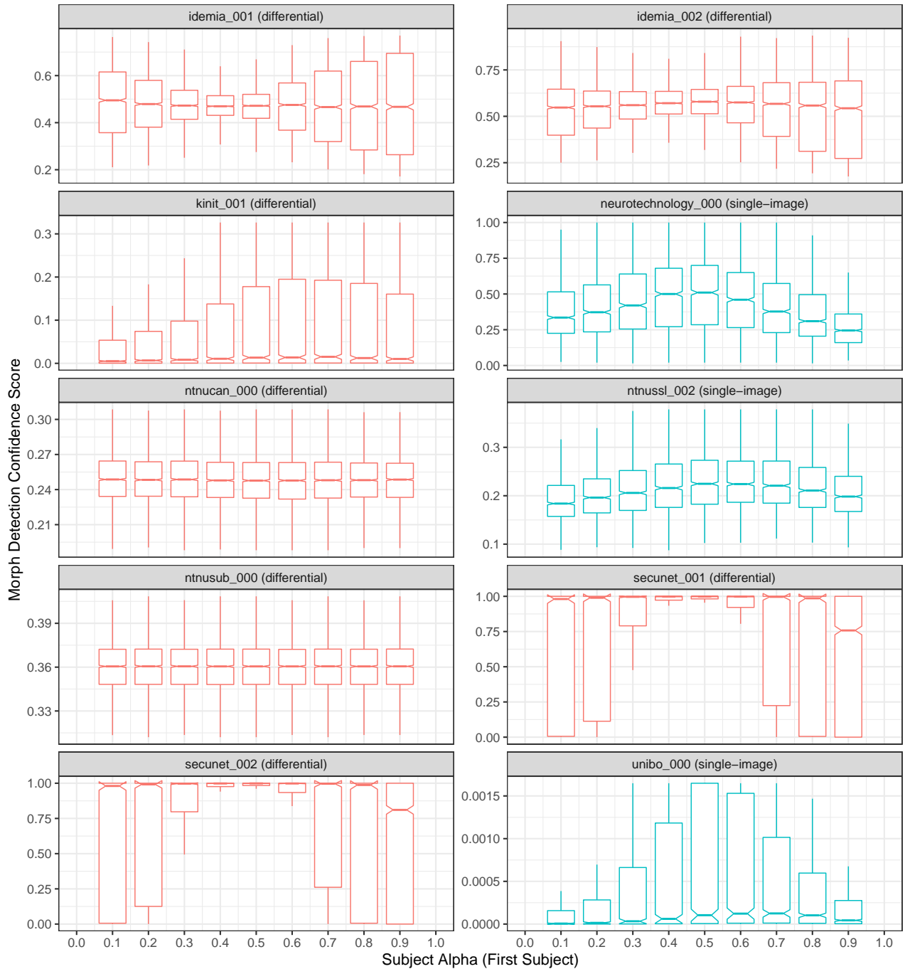
Figure 47: Boxplots plotting morph detection confidence score as a function of subject alpha (first subject in morph). Each plot includes scores that were successfully generated by the algorithm (i.e., results from failure to process were not used in this analysis). For individual algorithm results that are filterable and interactive, please refer to the algorithm report cards that are linked from the accuracy summary table on the FATE MORPH webpage .
