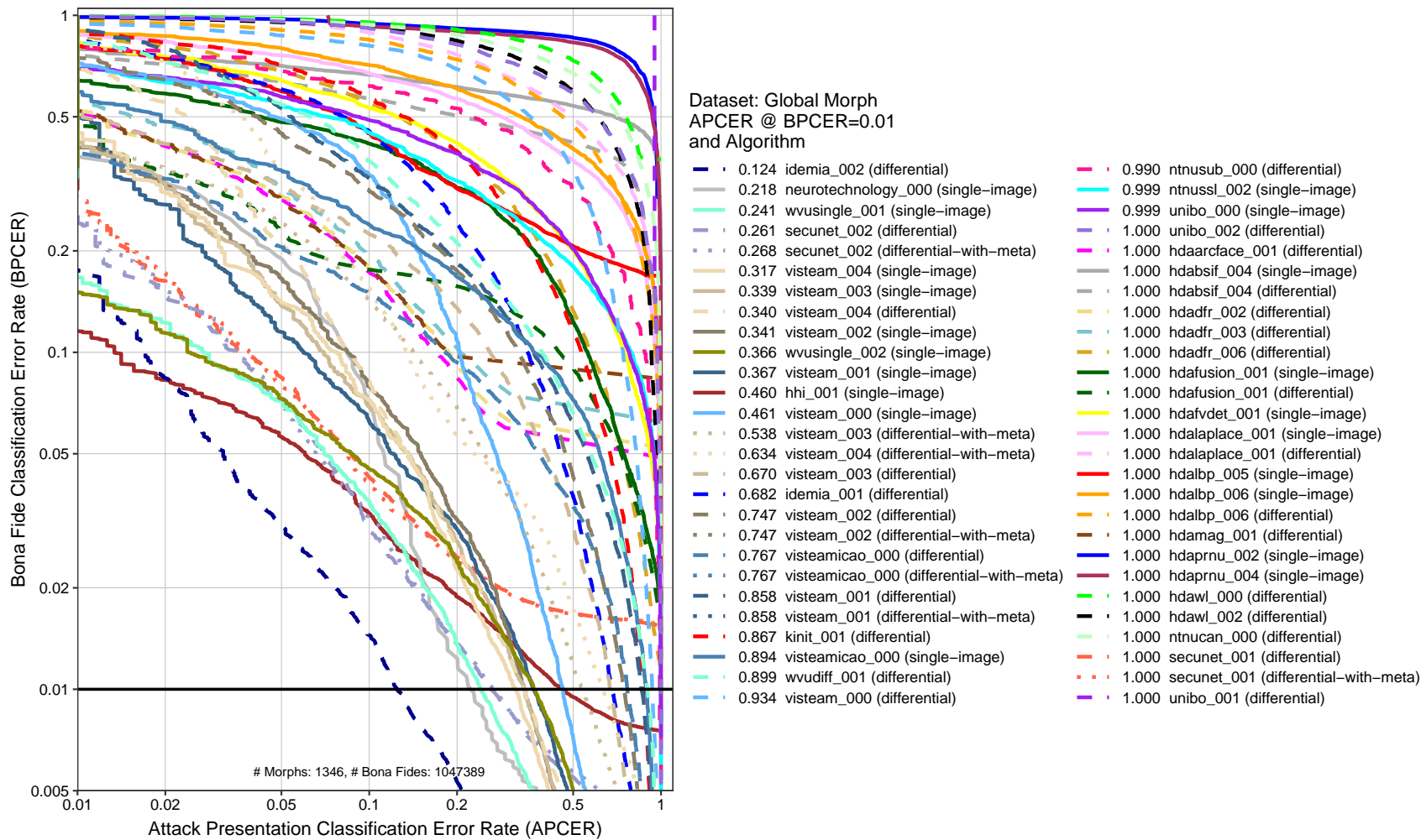
Figure 5: DET plot. This chart plots BPCER as a function of APCER. The x-axis is the rate morphs are not detected and the y-axis is the rate that bona fide images are falsely classified as morphs. The horizontal black line represents BPCER=0.01.
