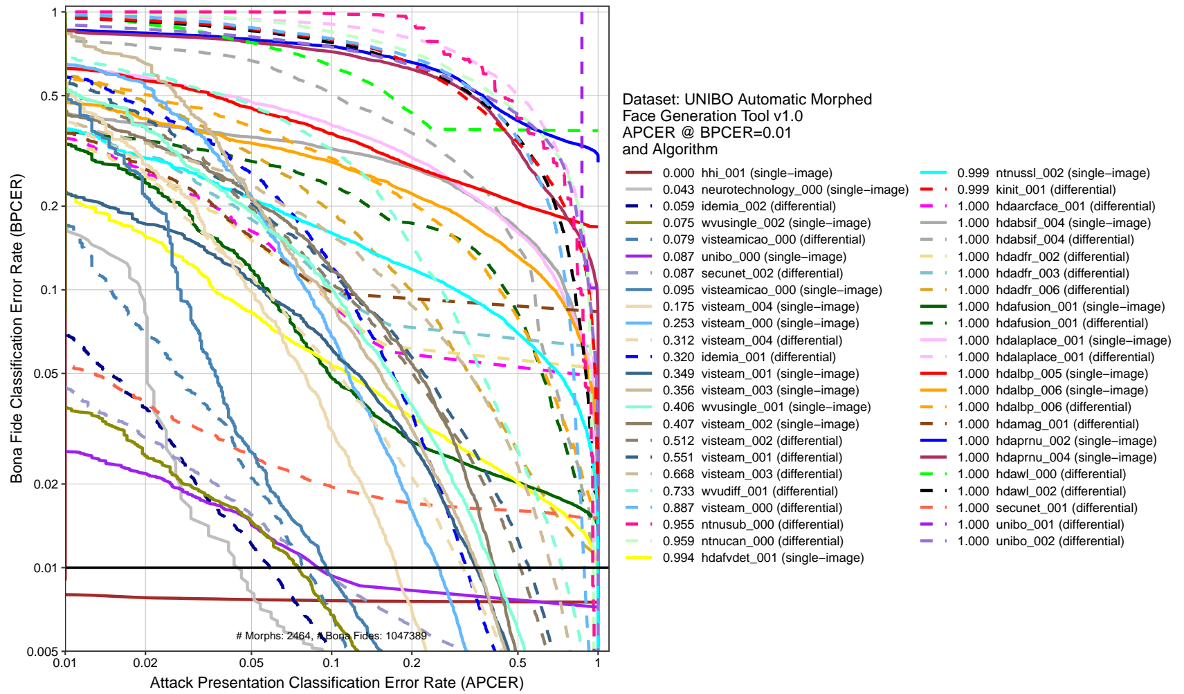
Figure 9: DET plot. This chart plots BPCER as a function of APCER. The x-axis is the rate morphs are not detected and the y-axis is the rate that bona fide images are falsely classified as morphs. The horizontal black line represents BPCER=0.01.
