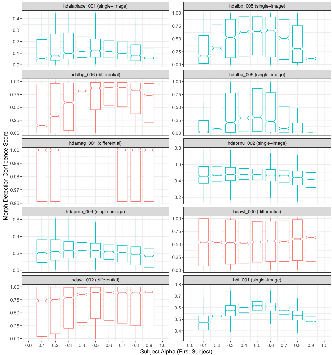
Figure 41: Boxplots plotting morph detection confidence score as a function of subject alpha (first subject in morph). Each plot includes scores that were successfully generated by the algorithm (i.e., results from failure to process were not used in this analysis). For individual algorithm results that are filterable and interactive, please refer to the algorithm report cards that are linked from the accuracy summary table on the FATE MORPH webpage .
