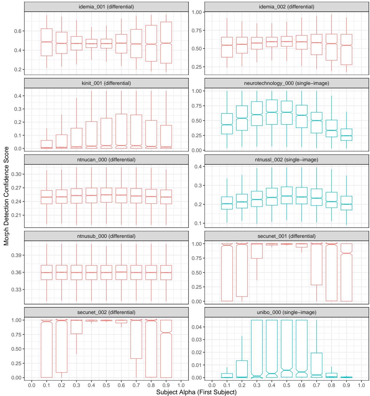
Figure 42: Boxplots plotting morph detection confidence score as a function of subject alpha (first subject in morph). Each plot includes scores that were successfully generated by the algorithm (i.e., results from failure to process were not used in this analysis). For individual algorithm results that are filterable and interactive, please refer to the algorithm report cards that are linked from the accuracy summary table on the FATE MORPH webpage .
