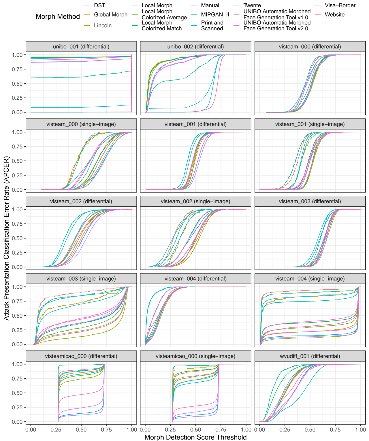
Figure 27: The APCER calibration curves show APCER (or morph miss rate) vs. morph detection score threshold. Separate curves appear for each morph dataset. For individual algorithm results that are filterable and interactive, please refer to the algorithm report cards that are linked from the accuracy summary table on the FATE MORPH webpage .
