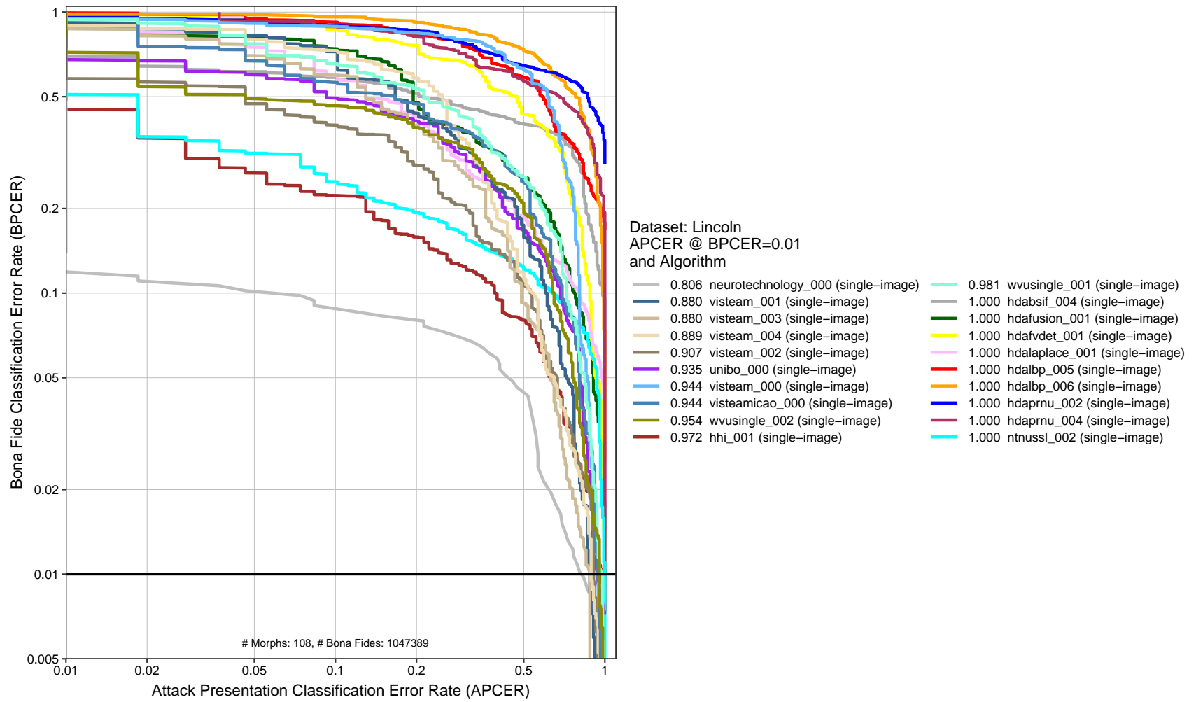
Figure 16: DET plot. This chart plots BPCER as a function of APCER. The x-axis is the rate morphs are not detected and the y-axis is the rate that bona fide images are falsely classified as morphs. The horizontal black line represents BPCER=0.01.
