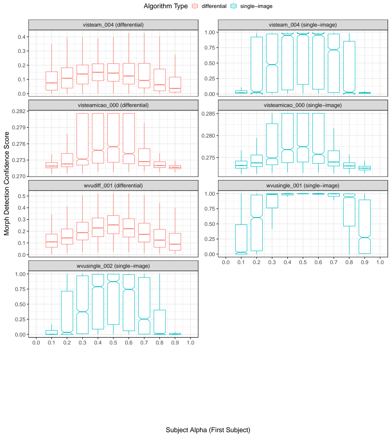
Figure 44: Boxplots plotting morph detection confidence score as a function of subject alpha (first subject in morph). Each plot includes scores that were successfully generated by the algorithm (i.e., results from failure to process were not used in this analysis). For individual algorithm results that are filterable and interactive, please refer to the algorithm report cards that are linked from the accuracy summary table on the FATE MORPH webpage .
