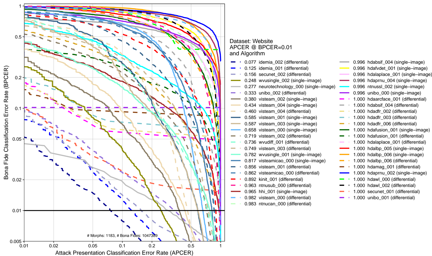
Figure 4: DET plot. This chart plots BPCER as a function of APCER. The x-axis is the rate morphs are not detected and the y-axis is the rate that bona fide images are falsely classified as morphs. The horizontal black line represents BPCER=0.01.
