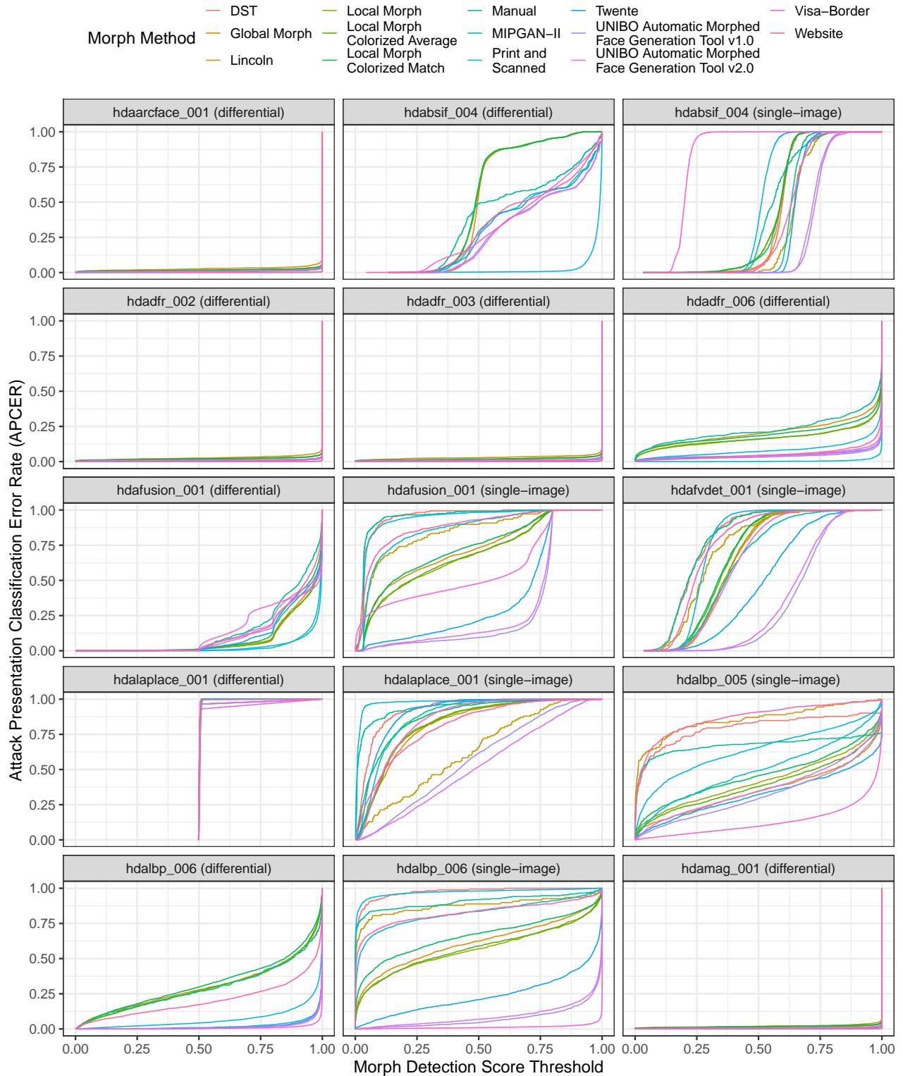
Figure 25: The APCER calibration curves show APCER (or morph miss rate) vs. morph detection score threshold. Separate curves appear for each morph dataset. For individual algorithm results that are filterable and interactive, please refer to the algorithm report cards that are linked from the accuracy summary table on the FATE MORPH webpage .
