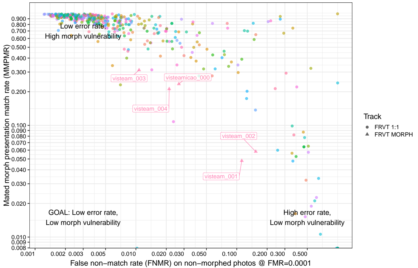
Figure 50: This graph plots face recognition algorithm vulnerability on morphs against general algorithm accuracy on non-morphed photos. Each circular point represents a face recognition algorithm recently submitted to the NIST FRTE 1:1 activity, and each triangular point represents a face recognition algorithm submitted to the NIST FATE MORPH activity. Note that algorithms submitted to FRTE 1:1 are not necessarily designed to handle morphed photos, and results are presented only as a point of reference. Submissions to FATE MORPH are designed with goals of face recognition algorithm resistance against morphing. The y-axis plots MMPMR, which is the fraction of morphs where both subjects incorrectly match to the morph. The x-axis plots FNMR or miss rate on regular photos, which provides an indication of general algorithm accuracy. Both MMPMR and FNMR are calculated with thresholds set to where the false match rate (FMR) is 0.0001. These results were generated with the Visa-Border morph dataset.
