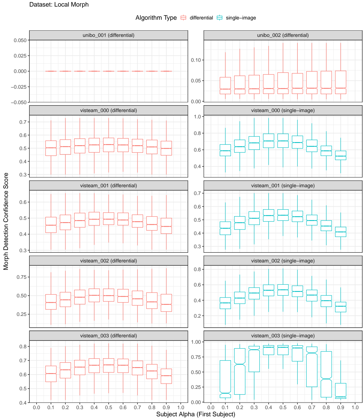
Figure 38: Boxplots plotting morph detection confidence score as a function of subject alpha (first subject in morph). Each plot includes scores that were successfully generated by the algorithm (i.e., results from failure to process were not used in this analysis). For individual algorithm results that are filterable and interactive, please refer to the algorithm report cards that are linked from the accuracy summary table on the FATE MORPH webpage .
