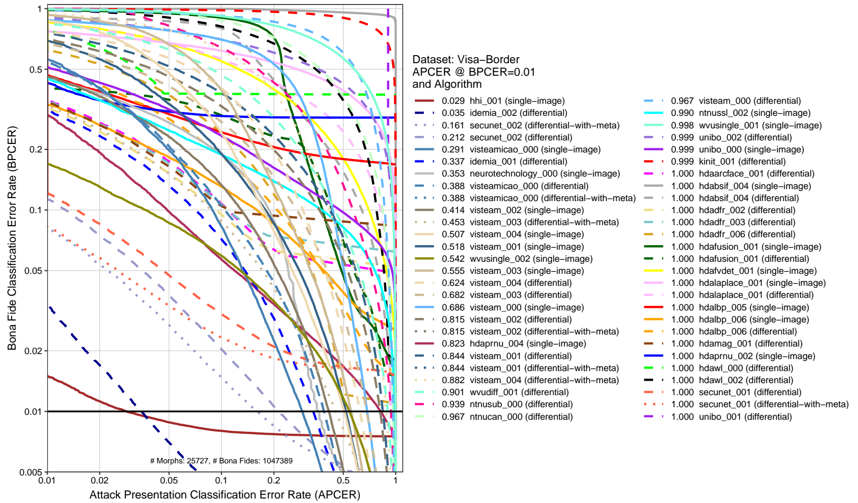
Figure 11: DET plot. This chart plots BPCER as a function of APCER. The x-axis is the rate morphs are not detected and the y-axis is the rate that bona fide images are falsely classified as morphs. The horizontal black line represents BPCER=0.01.
