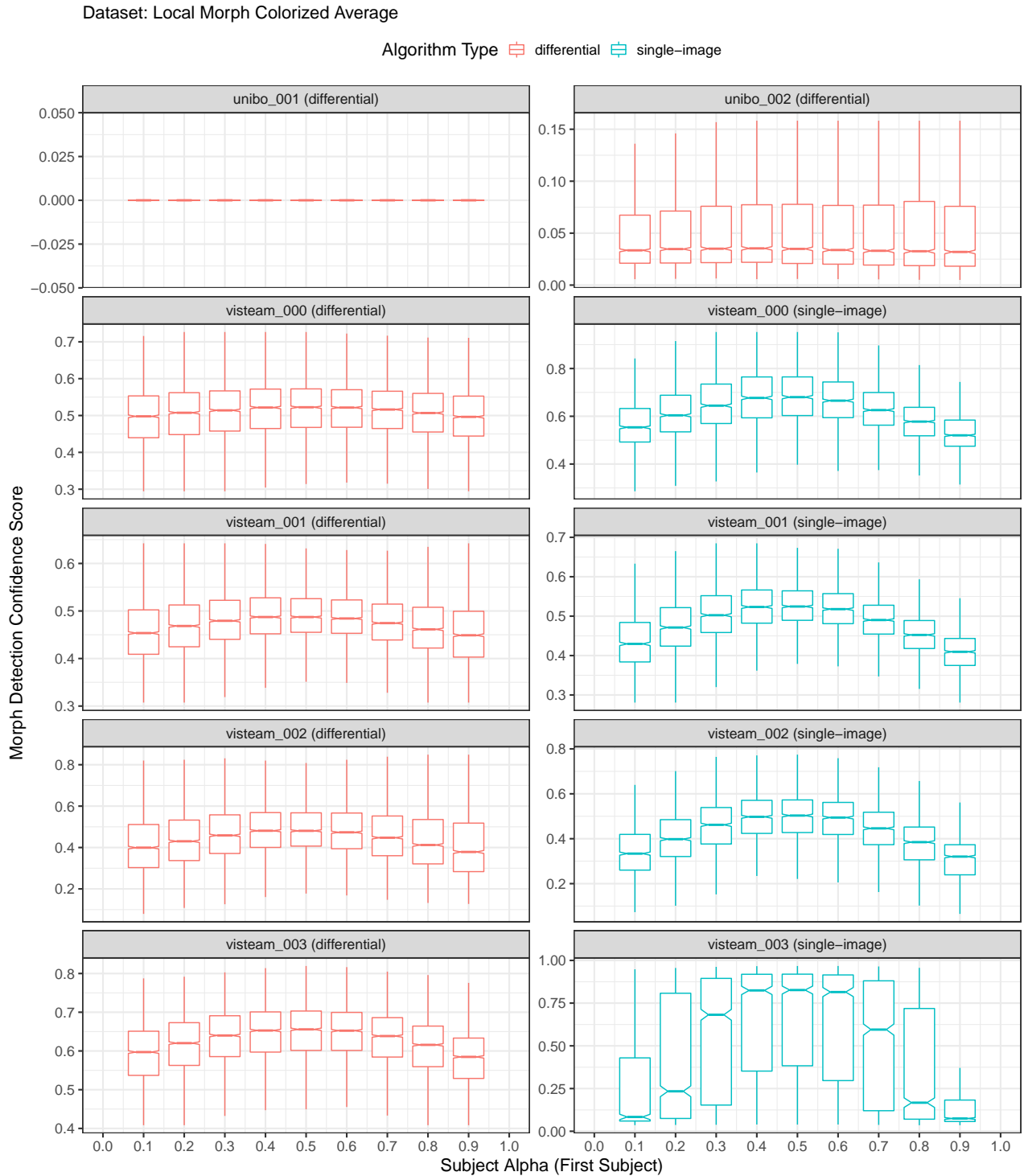
Figure 43: Boxplots plotting morph detection confidence score as a function of subject alpha (first subject in morph). Each plot includes scores that were successfully generated by the algorithm (i.e., results from failure to process were not used in this analysis). For individual algorithm results that are filterable and interactive, please refer to the algorithm report cards that are linked from the accuracy summary table on the FATE MORPH webpage .
