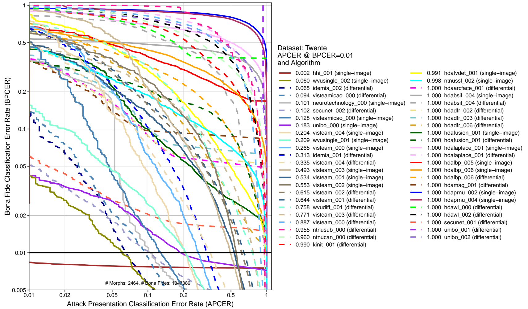
Figure 13: DET plot. This chart plots BPCER as a function of APCER. The x-axis is the rate morphs are not detected and the y-axis is the rate that bona fide images are falsely classified as morphs. The horizontal black line represents BPCER=0.01.
