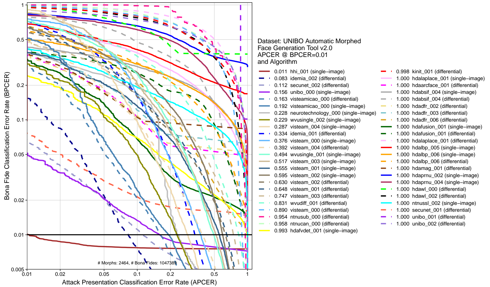
Figure 12: DET plot. This chart plots BPCER as a function of APCER. The x-axis is the rate morphs are not detected and the y-axis is the rate that bona fide images are falsely classified as morphs. The horizontal black line represents BPCER=0.01.
