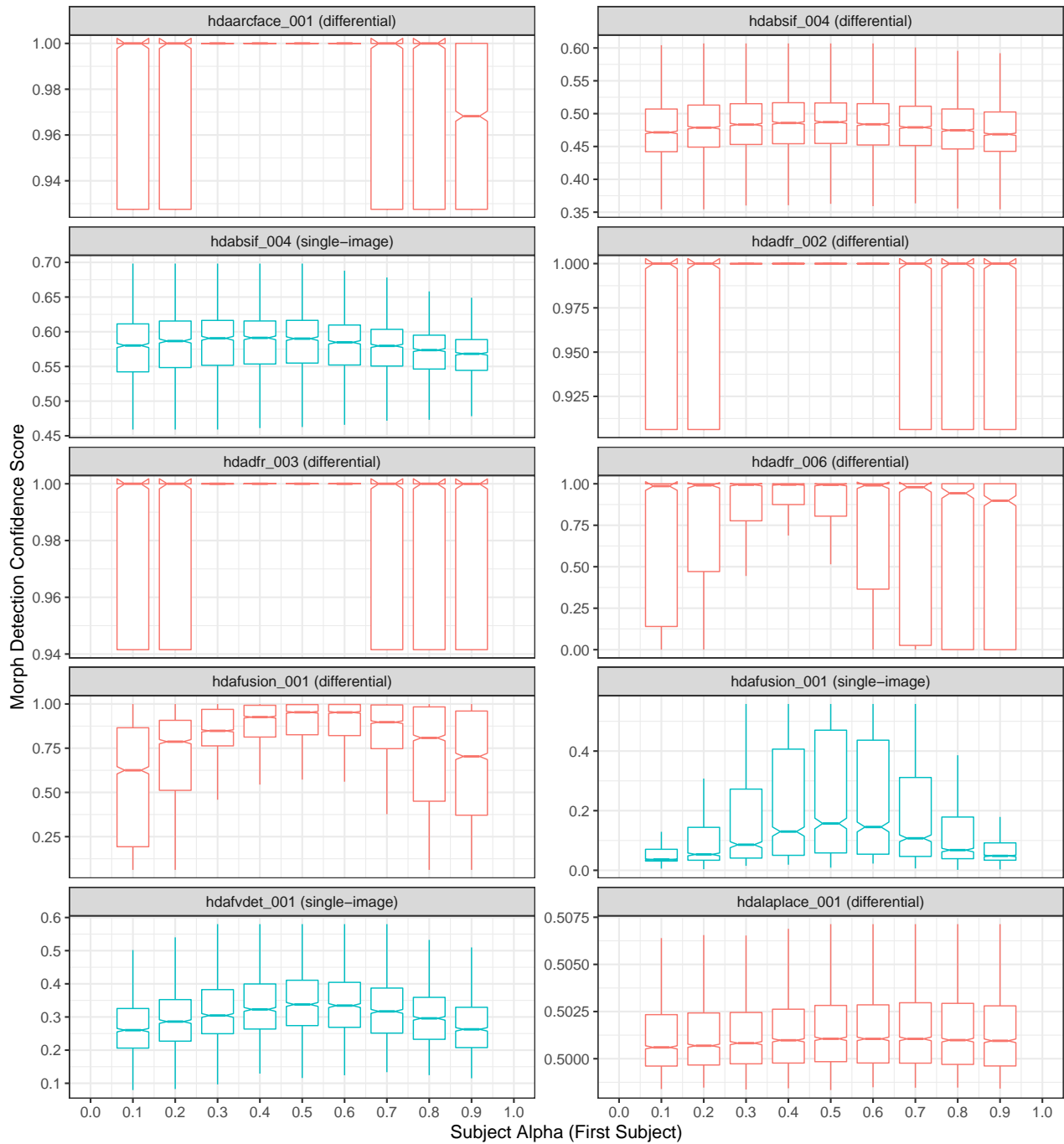
Figure 45: Boxplots plotting morph detection confidence score as a function of subject alpha (first subject in morph). Each plot includes scores that were successfully generated by the algorithm (i.e., results from failure to process were not used in this analysis). For individual algorithm results that are filterable and interactive, please refer to the algorithm report cards that are linked from the accuracy summary table on the FATE MORPH webpage .
