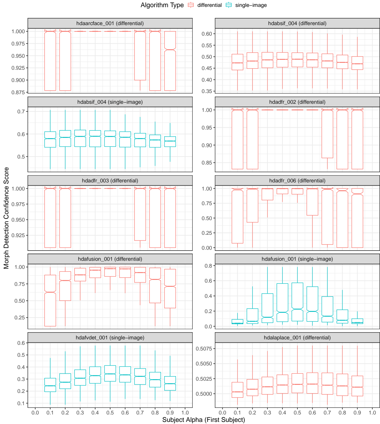
Figure 40: Boxplots plotting morph detection confidence score as a function of subject alpha (first subject in morph). Each plot includes scores that were successfully generated by the algorithm (i.e., results from failure to process were not used in this analysis). For individual algorithm results that are filterable and interactive, please refer to the algorithm report cards that are linked from the accuracy summary table on the FATE MORPH webpage .
