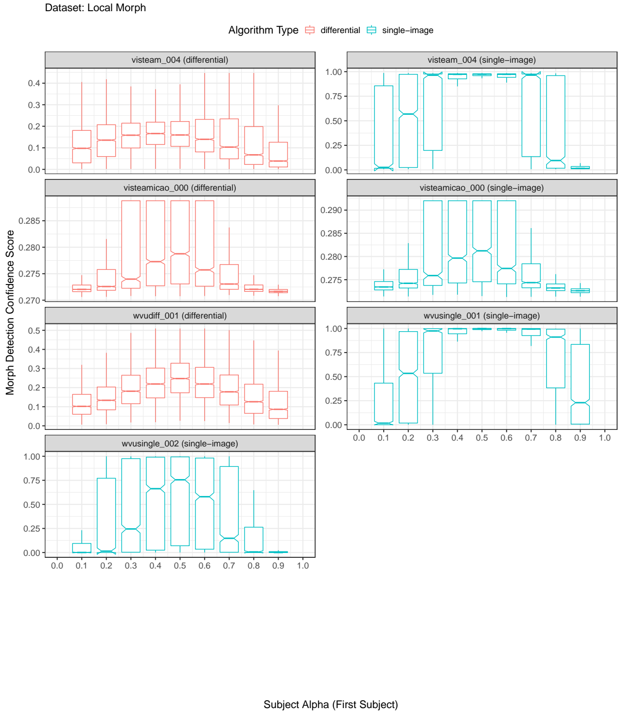
Figure 39: Boxplots plotting morph detection confidence score as a function of subject alpha (first subject in morph). Each plot includes scores that were successfully generated by the algorithm (i.e., results from failure to process were not used in this analysis). For individual algorithm results that are filterable and interactive, please refer to the algorithm report cards that are linked from the accuracy summary table on the FATE MORPH webpage .
