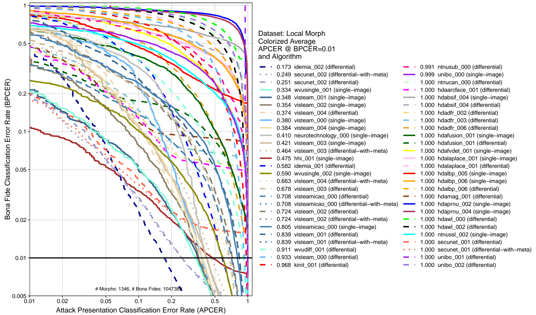
Figure 7: DET plot. This chart plots BPCER as a function of APCER. The x-axis is the rate morphs are not detected and the y-axis is the rate that bona fide images are falsely classified as morphs. The horizontal black line represents BPCER=0.01.
