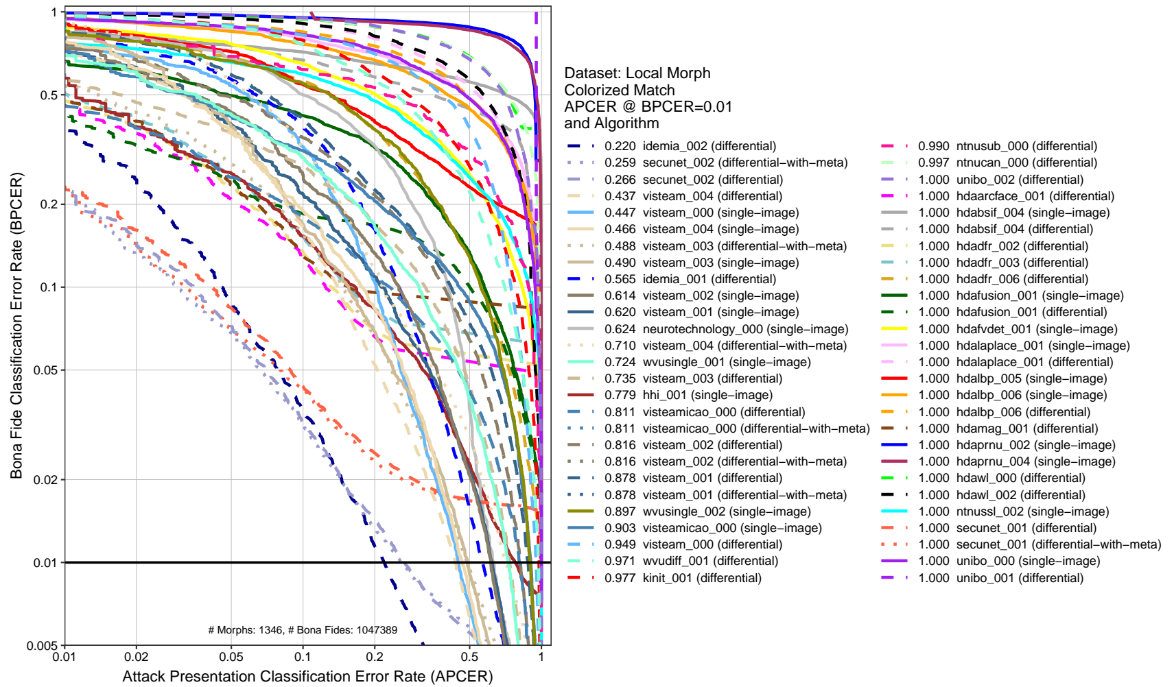
Figure 8: DET plot. This chart plots BPCER as a function of APCER. The x-axis is the rate morphs are not detected and the y-axis is the rate that bona fide images are falsely classified as morphs. The horizontal black line represents BPCER=0.01.
