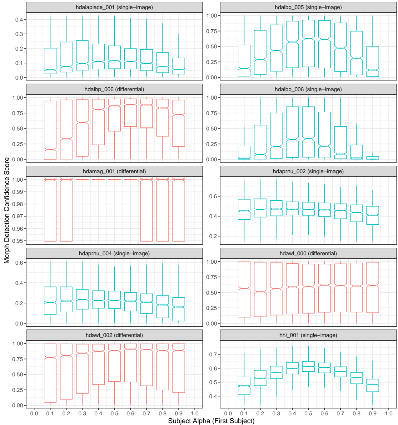
Figure 36: Boxplots plotting morph detection confidence score as a function of subject alpha (first subject in morph). Each plot includes scores that were successfully generated by the algorithm (i.e., results from failure to process were not used in this analysis). For individual algorithm results that are filterable and interactive, please refer to the algorithm report cards that are linked from the accuracy summary table on the FATE MORPH webpage .
