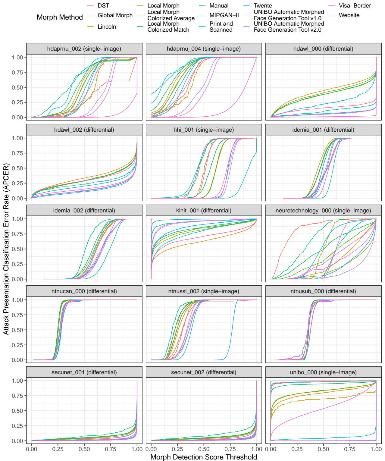
Figure 26: The APCER calibration curves show APCER (or morph miss rate) vs. morph detection score threshold. Separate curves appear for each morph dataset. For individual algorithm results that are filterable and interactive, please refer to the algorithm report cards that are linked from the accuracy summary table on the FATE MORPH webpage .
