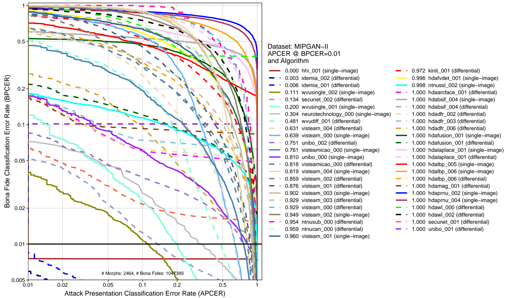
Figure 14: DET plot. This chart plots BPCER as a function of APCER. The x-axis is the rate morphs are not detected and the y-axis is the rate that bona fide images are falsely classified as morphs. The horizontal black line represents BPCER=0.01.
