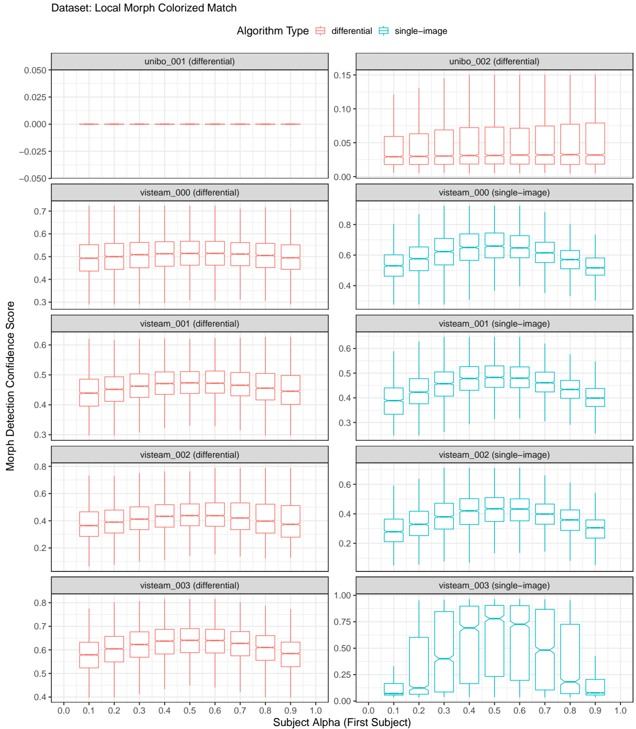
Figure 48: Boxplots plotting morph detection confidence score as a function of subject alpha (first subject in morph). Each plot includes scores that were successfully generated by the algorithm (i.e., results from failure to process were not used in this analysis). For individual algorithm results that are filterable and interactive, please refer to the algorithm report cards that are linked from the accuracy summary table on the FATE MORPH webpage .
