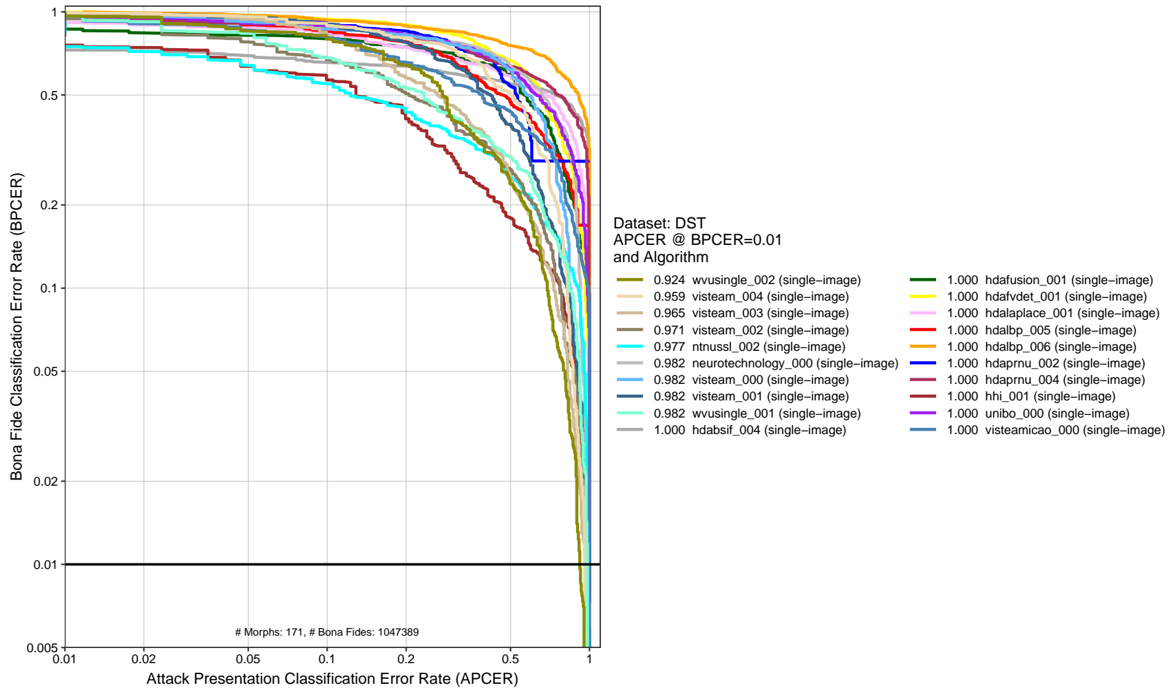
Figure 10: DET plot. This chart plots BPCER as a function of APCER. The x-axis is the rate morphs are not detected and the y-axis is the rate that bona fide images are falsely classified as morphs. The horizontal black line represents BPCER=0.01.
