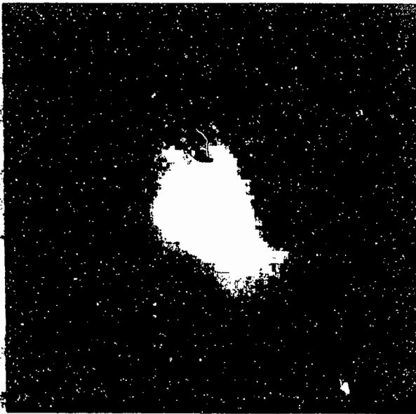
A NASA Hubble Space Telescope image of a spiral-shaped disk of hot gas in the core of active galaxy M87. Hubble measurements show the disk is rotating so rapidly it contains a massive black hole at its hub. Source: National Aeronautics and Space Administration
